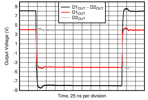
图 5-24. Overdrive Recovery
