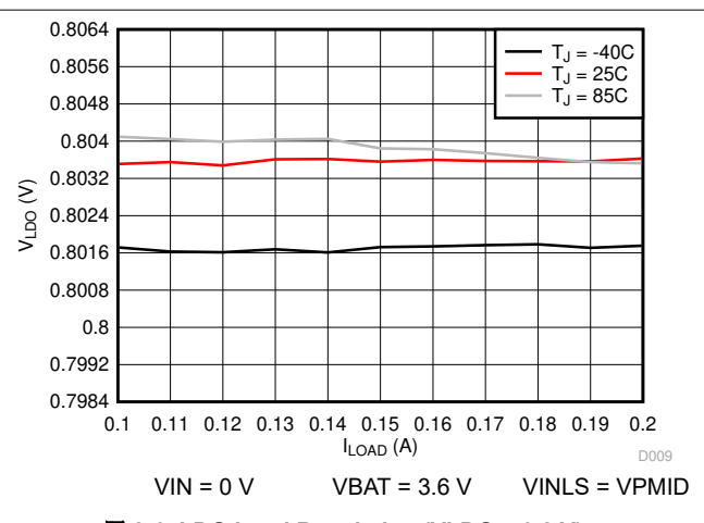
图 8-6. LDO Load Regulation (VLDO = 0.8 V)
