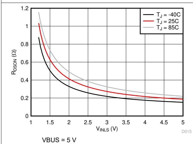
图 8-5. LS/LDO Switch On Resistance vs. VINLS
