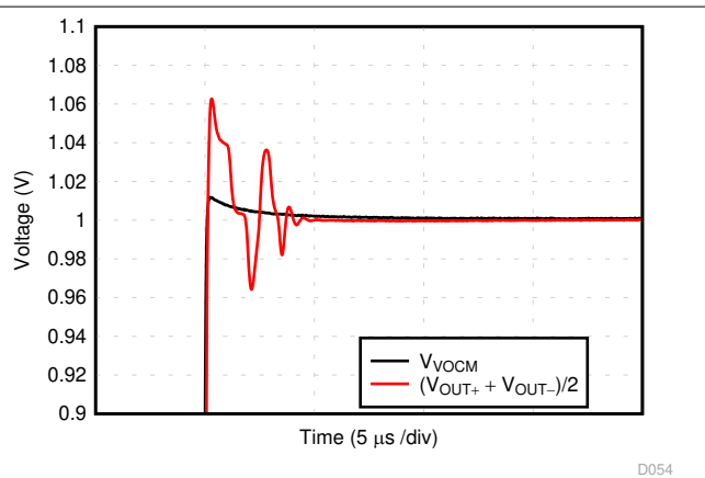
图 6-34. Output Common-Mode Step Response, Rising
