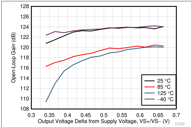
图 6-31. Open-Loop Gain vs Ouput Delta From Supply
