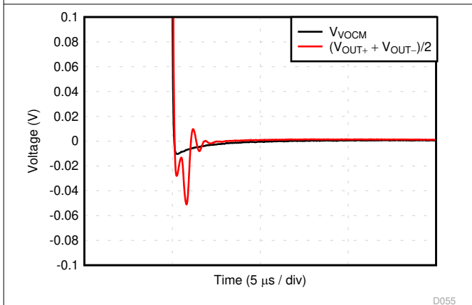
图 6-35. Output Common-Mode Step Response, Falling
