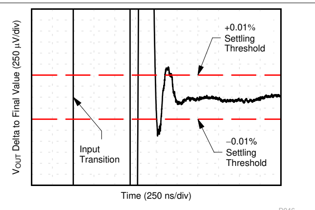
图 6-36. Output Settling Time to \pm 0.01\%
