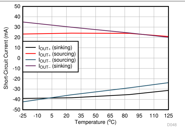
图 6-32. Short-Circuit Current vs Temperature
