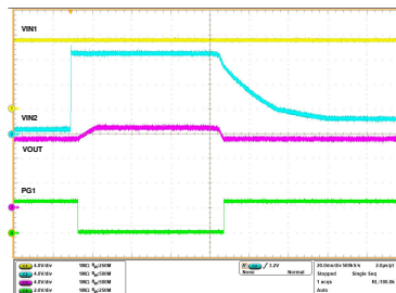
图 9-9. Active ORing Response
