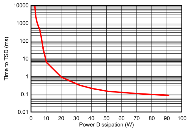
图 7-36. Time to Thermal Shut-Down During Inrush State
