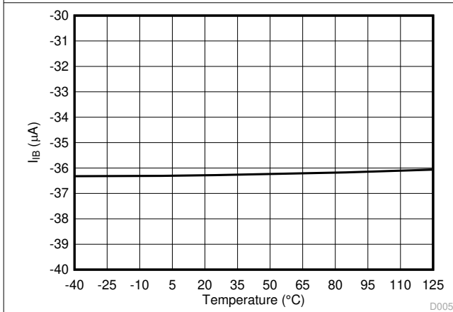
图 6-8. Input Bias Current vs Temperature
