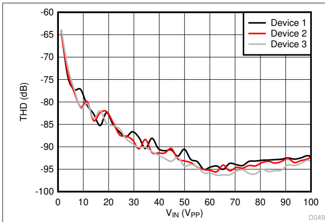
图 6-24. Total Harmonic Distortion vs Input Signal Amplitude
