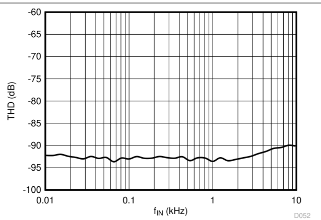
图 6-25. Total Harmonic Distortion vs Input Signal Frequency
