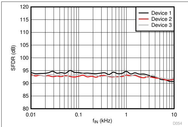
图 6-30. Spurious-Free Dynamic Range vs Input Signal Frequency
