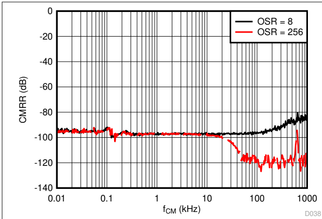
图 6-36. Common-Mode Rejection Ratio vs Input Signal Frequency
