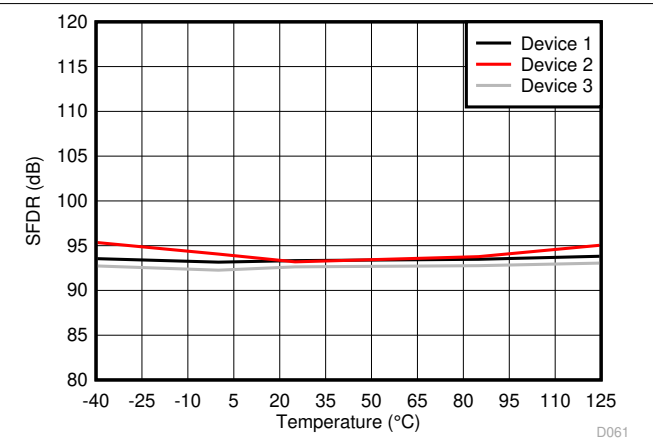
图 6-33. Spurious-Free Dynamic Range vs Temperature
