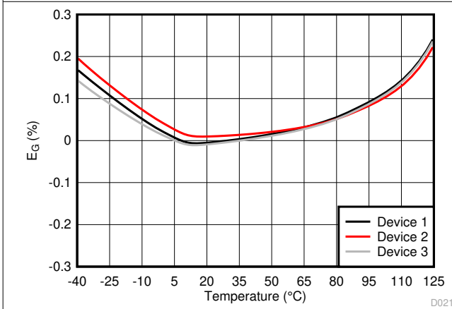
图 6-14. Gain Error vs Temperature
