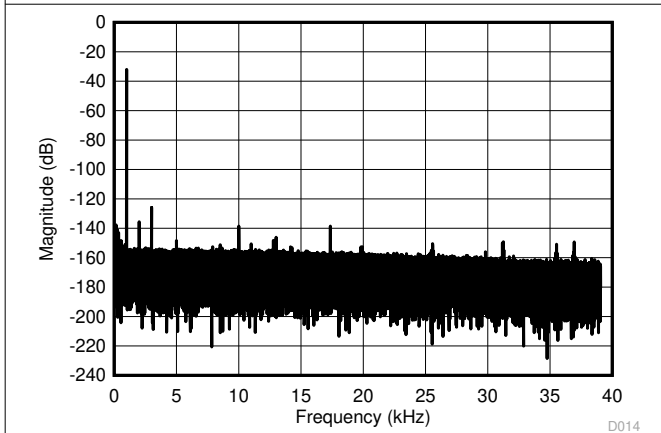
图 6-34. Output Frequency Spectrum With a 1-kHz Input Signal
