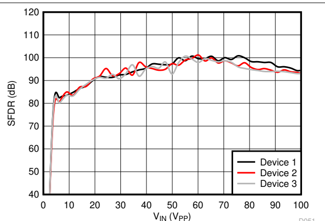
图 6-29. Spurious-Free Dynamic Range vs Input Signal Amplitude
