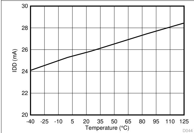
图 6-40. Supply Current vs Temperature
