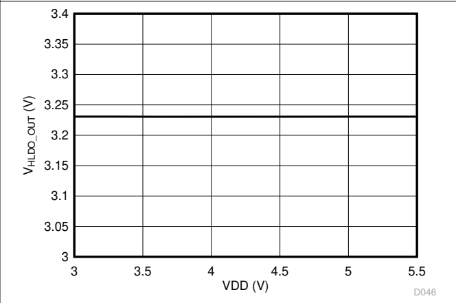
图 6-41. High-Side LDO Output Voltage vs Supply Voltage
