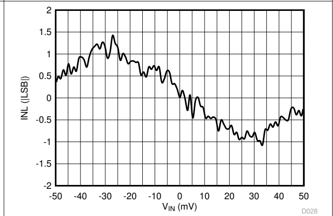
图 6-15. Integral Nonlinearity vs Input Voltage
