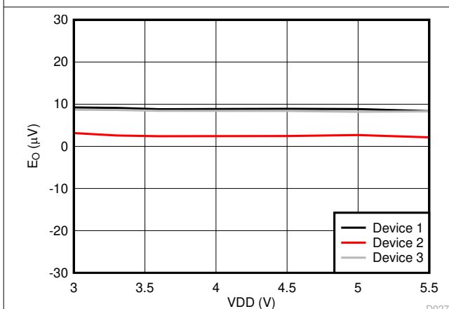
图 6-10. Offset Error vs Supply Voltage
