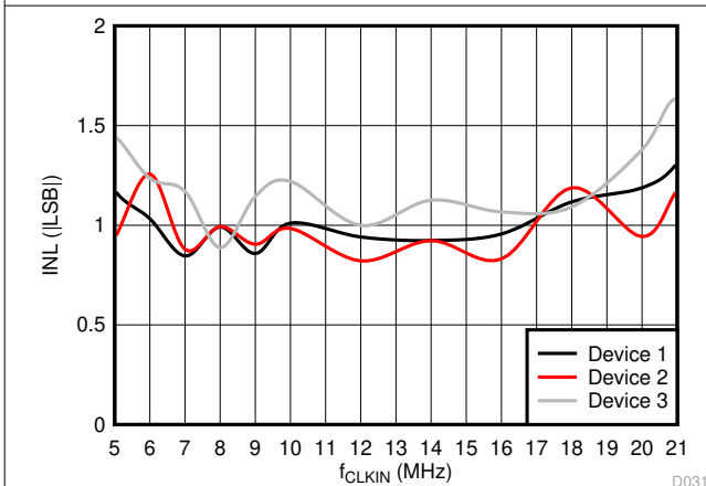
图 6-16. Integral Nonlinearity vs Input Clock Frequency
