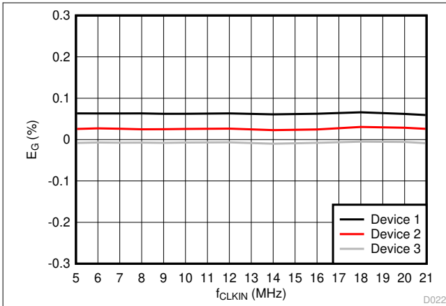
图 6-12. Gain Error vs Input Clock Frequency
