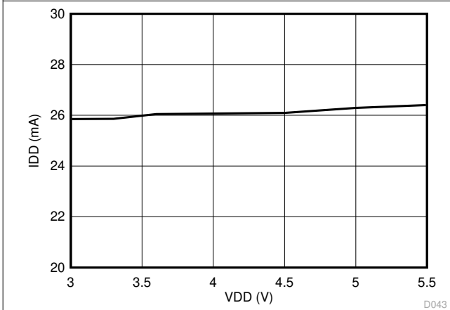
图 6-38. Supply Current vs Supply Voltage
