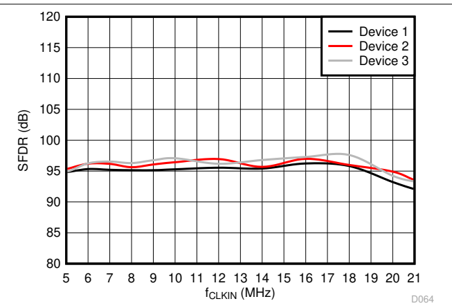
图 6-31. Spurious-Free Dynamic Range vs Input Clock Frequency
