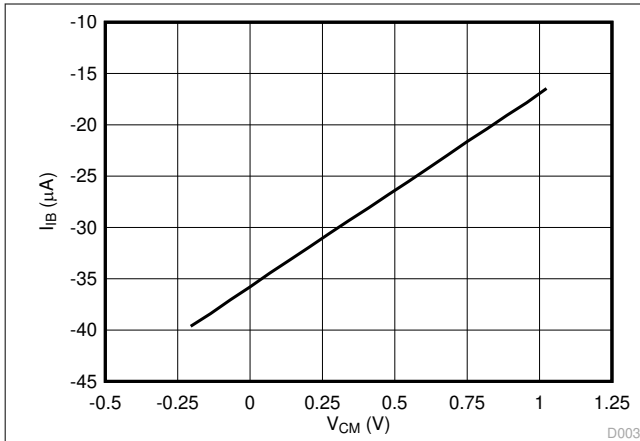
图 6-6. Input Bias Current vs Common-Mode Input Voltage
