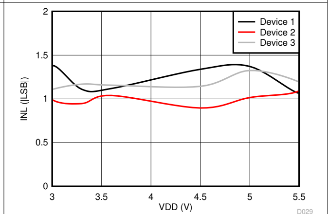
图 6-17. Integral Nonlinearity vs Supply Voltage
