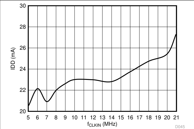
图 6-39. Supply Current vs Input Clock Frequency
