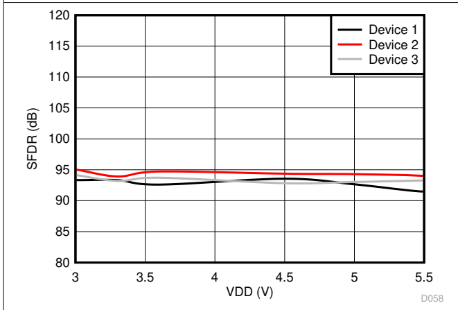
图 6-32. Spurious-Free Dynamic Range vs Supply Voltage
