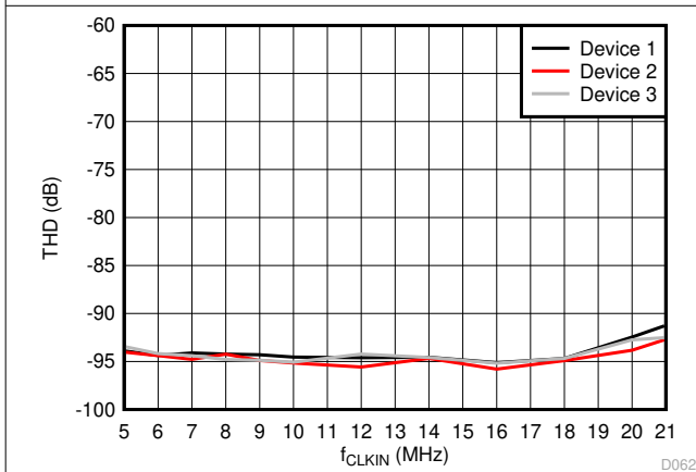
图 6-26. Total Harmonic Distortion vs Input Clock Frequency
