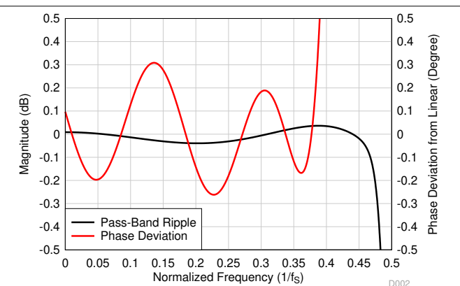
图 7-42. Low-Latency Decimation Filter Pass-Band Ripple and Phase Deviation
