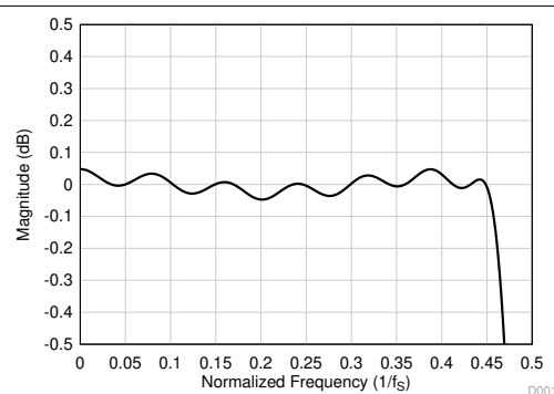
图 7-24. Linear Phase Decimation Filter Pass-Band Ripple
