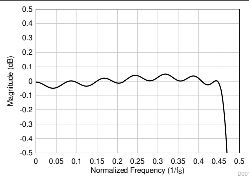
图 7-22. Linear Phase Decimation Filter Pass-Band Ripple
