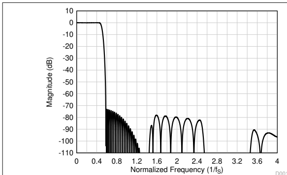
图 7-23. Linear Phase Decimation Filter Magnitude Response
