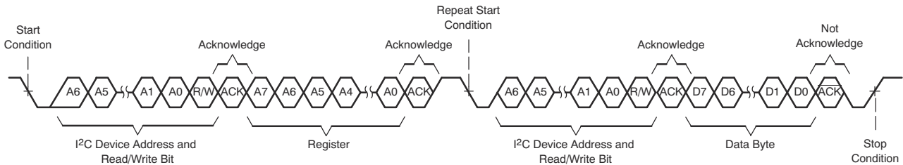
图 7-66. I 2 C Single-Byte Read Transfer
