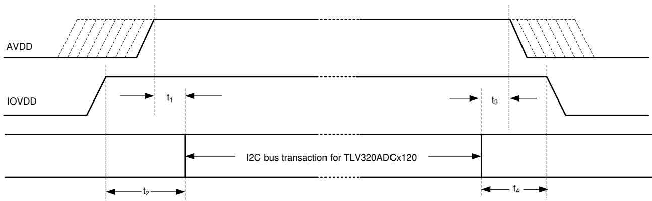
图 9-1. Power-Supply Sequencing Requirement Timing Diagram
