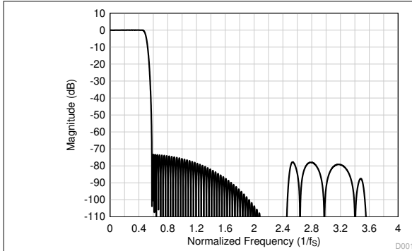
图 7-21. Linear Phase Decimation Filter Magnitude Response
