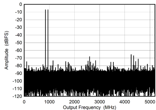
图 6-12. DES Mode: Two Tone FFT at 897 MHz
