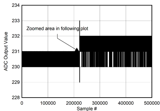
图 6-121. Background Calibration Core Transition (DC Signal)
