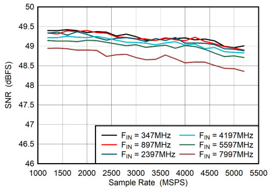
图 6-45. Dual Channel Mode: SNR vs Sample Rate A_{IN} = -6\text{ dBFS}
