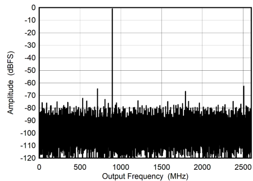
图 6-18. Dual Channel Mode: Single Tone FFT at 897 MHz
