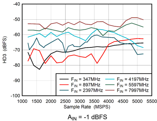
图 6-53. Dual Channel Mode: HD3 vs Sample Rate
