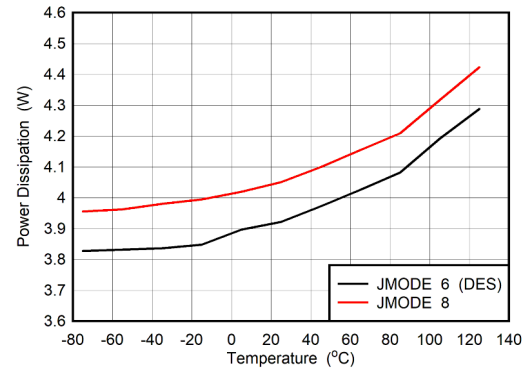
图 6-118. Power Dissipation vs Temperature
