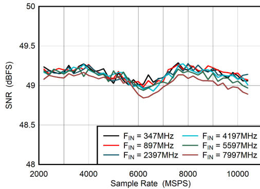
图 6-31. DES Mode: SNR vs Sample Rate
