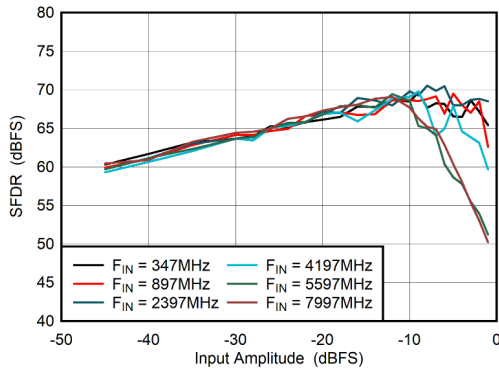
图 6-73. Dual Channel Mode: SFDR vs Input Amplitude
