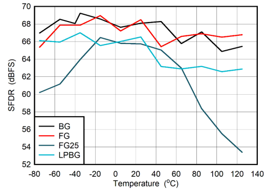
图 6-92. Dual Channel Mode: SFDR vs Temperature and Calibration
