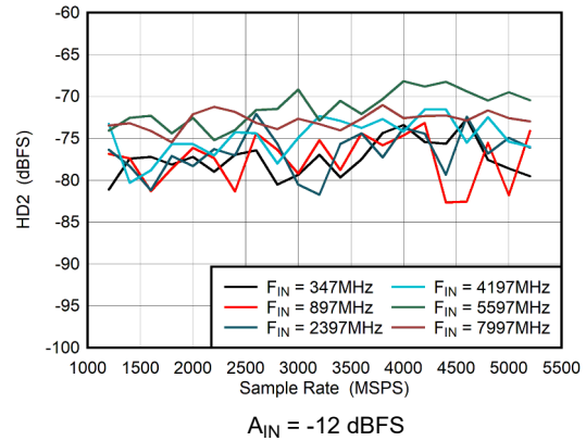
图 6-52. Dual Channel Mode: HD2 vs Sample Rate
