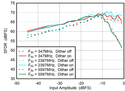
图 6-74. Dual Channel Mode: SFDR vs Input Amplitude and Dither
