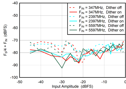
图 6-68. DES Mode: F_S/4 + F_{IN} vs Input Amplitude and Dither
