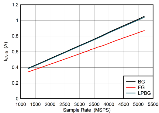
图 6-115. Dual Channel Mode: I_{VA11} vs Sample Rate
