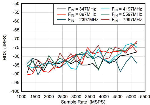
图 6-55. Dual Channel Mode: HD3 vs Sample Rate
