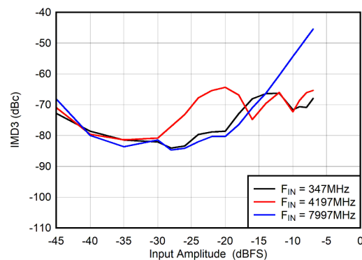
图 6-106. Dual Channel Mode: IMD3 vs Input Amplitude
