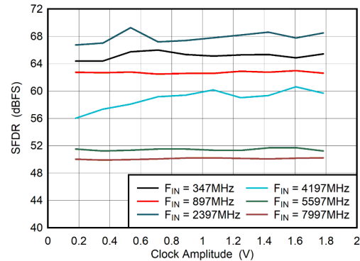
图 6-84. Dual Channel Mode: SFDR vs Clock Amplitude
