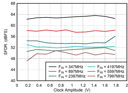
图 6-82. DES Mode: SFDR vs Clock Amplitude
