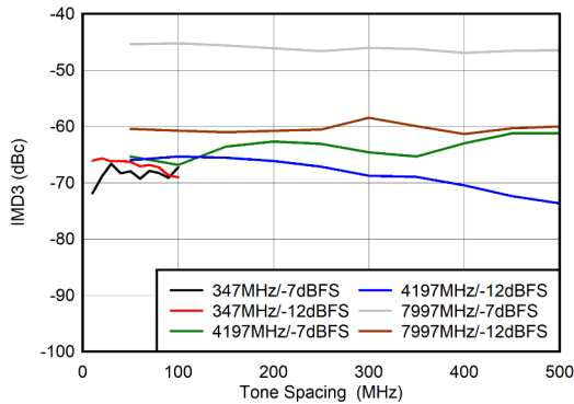
图 6-107. Dual Channel Mode: IMD3 vs Tone Spacing
