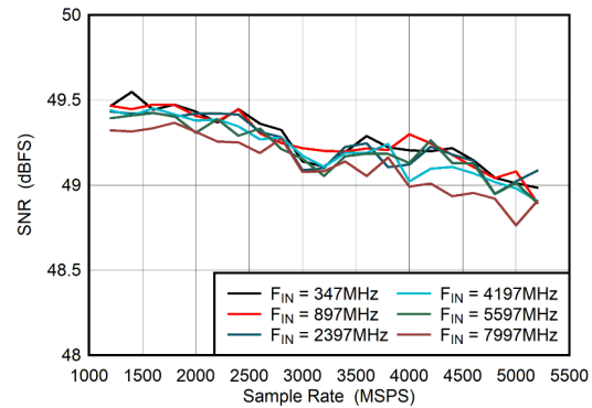
图 6-46. Dual Channel Mode: SNR vs Sample Rate A_{IN} = -12\text{ dBFS}
