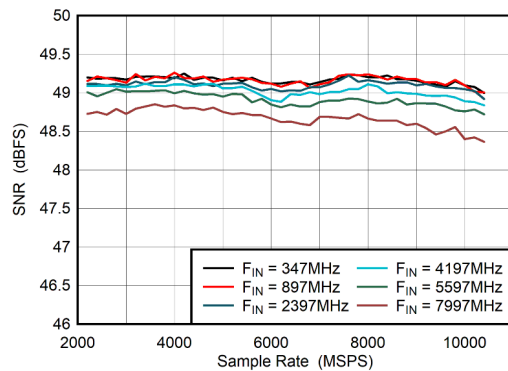
图 6-30. DES Mode: SNR vs Sample Rate
