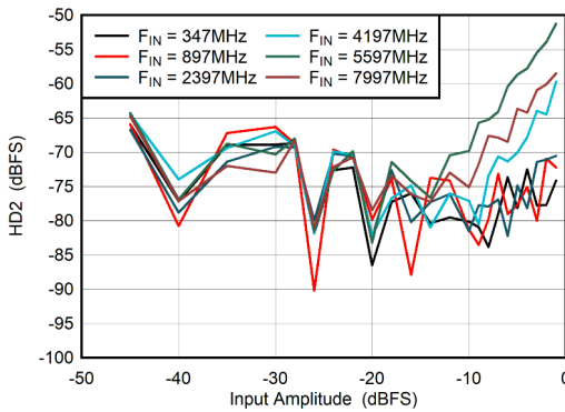
图 6-75. Dual Channel Mode: HD2 vs Input Amplitude
