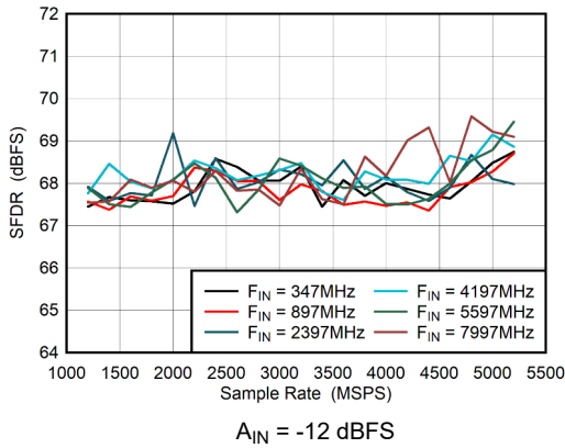
图 6-49. Dual Channel Mode: SFDR vs Sample Rate
