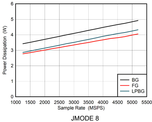
图 6-117. Dual Channel Mode: Power Dissipation vs Sample Rate
