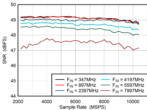
图 6-29. DES Mode: SNR vs Sample Rate
