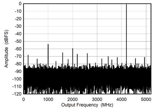
图 6-8. DES Mode: Single Tone FFT at 4197 MHz
