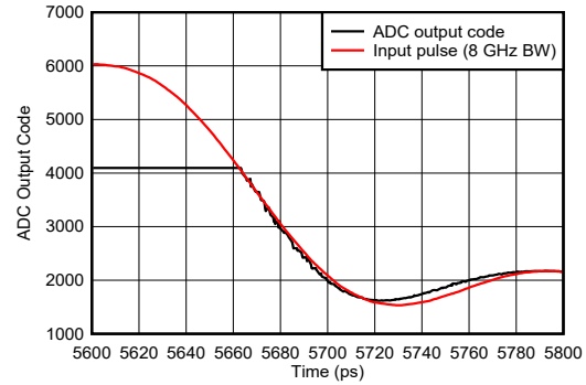
图 6-124. Pulse Overdrive Recovery Zoomed
