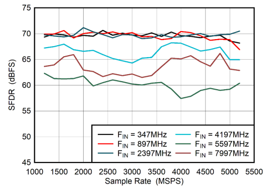
图 6-48. Dual Channel Mode: SFDR vs Sample Rate A_{IN} = -6\text{ dBFS}
