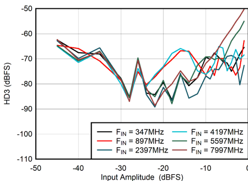
图 6-77. Dual Channel Mode: HD3 vs Input Amplitude
