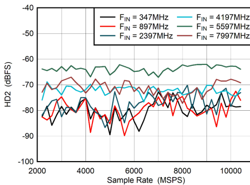
图 6-36. DES Mode: HD2 vs Sample Rate
