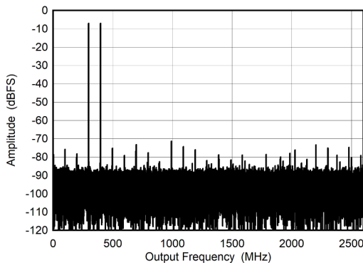
图 6-23. Dual Channel Mode: Two Tone FFT at 347 MHz
