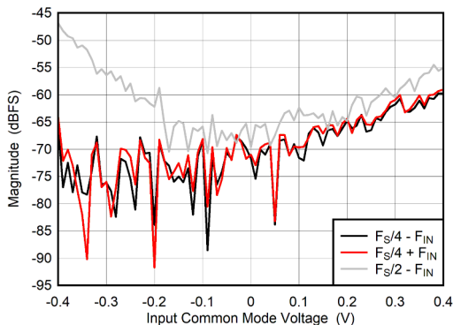
图 6-99. DES Mode: F_S/2 - F_{IN} , F_S/4 + F_{IN} vs Input Common Mode Voltage
