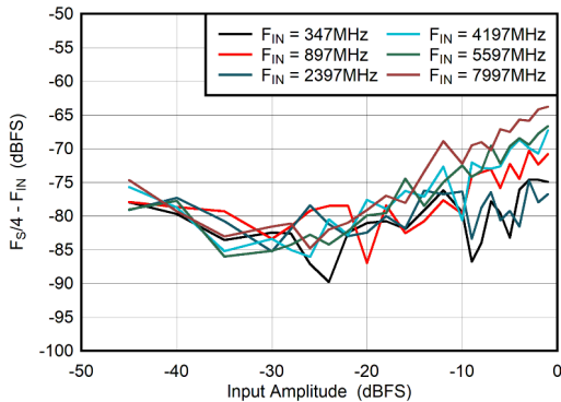
图 6-69. DES Mode: F_S/4 - F_{IN} vs Input Amplitude
