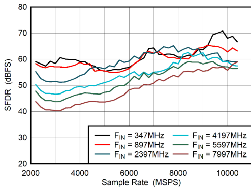
图 6-33. DES Mode: SFDR vs Sample Rate
