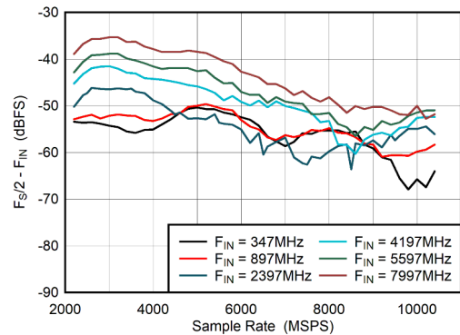
图 6-41. DES Mode: F_S/2 - F_{IN} vs Sample Rate
