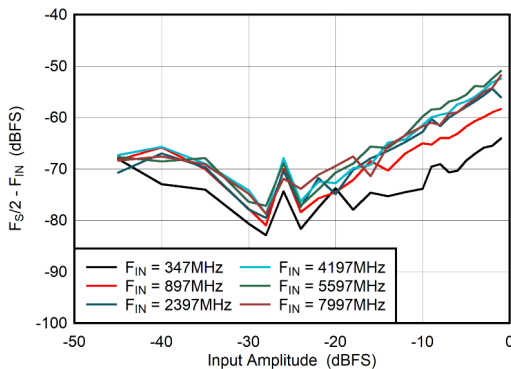
图 6-65. DES Mode: F_s/2 - F_{IN} vs Input Amplitude
