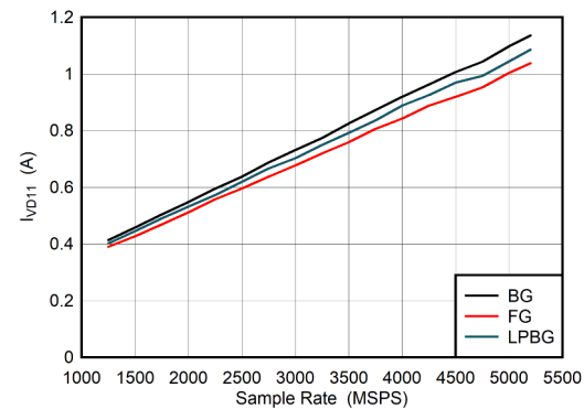
图 6-116. Dual Channel Mode: I_{VD11} vs Sample Rate
