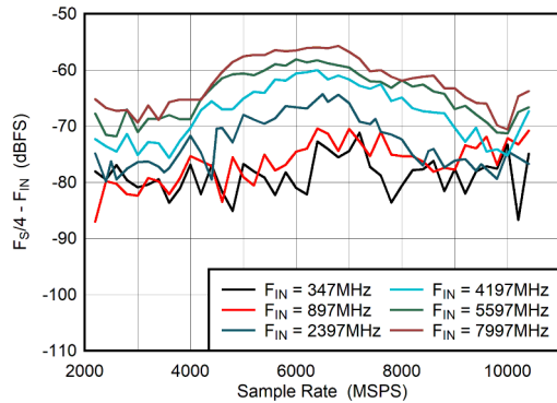
图 6-43. DES Mode: F_S/4 - F_{IN} vs Sample Rate
