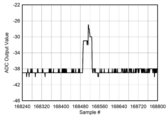
图 6-120. Background Calibration Core Transition (AC Signal Zoomed)
