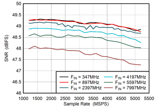
图 6-44. Dual Channel Mode: SNR vs Sample Rate A_{IN} = -1\text{ dBFS}
