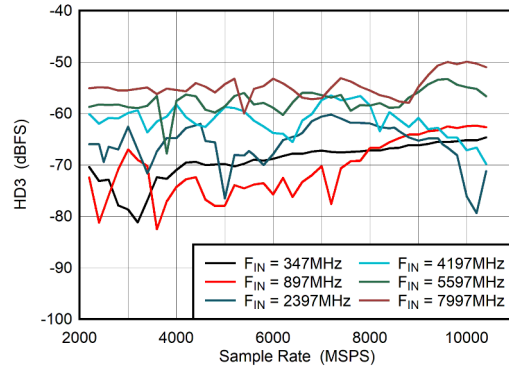
图 6-38. DES Mode: HD3 vs Sample Rate
