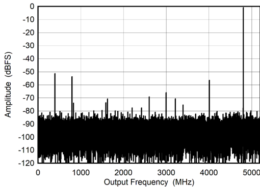
图 6-9. DES Mode: Single Tone FFT at 5597 MHz
