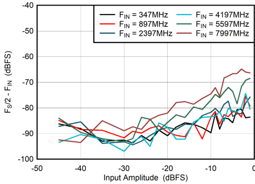
图 6-79. Dual Channel Mode: F_{S/2} - F_{IN} vs Input Amplitude
