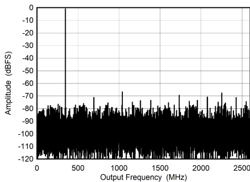
图 6-17. Dual Channel Mode: Single Tone FFT at 347 MHz
