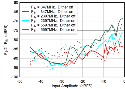
图 6-80. Dual Channel Mode: F_{S/2} - F_{IN} vs Input Amplitude and Dither
