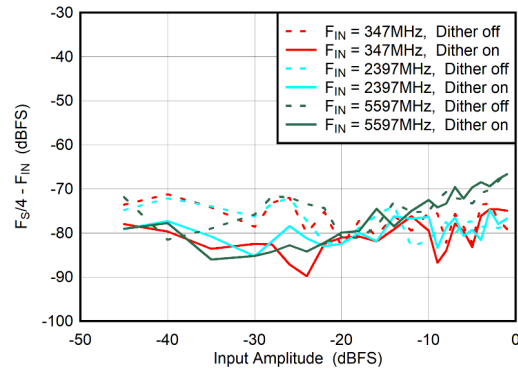
图 6-70. DES Mode: F_S/4 - F_{IN} vs Input Amplitude and Dither
