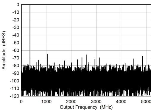
图 6-5. DES Mode: Single Tone FFT at 347 MHz
