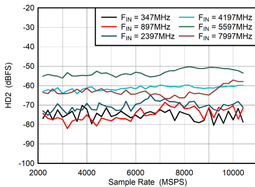
图 6-35. DES Mode: HD2 vs Sample Rate
