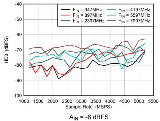
图 6-54. Dual Channel Mode: HD3 vs Sample Rate
