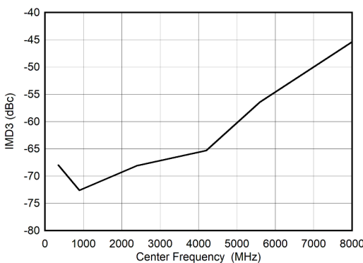
图 6-105. Dual Channel Mode: IMD3 vs Input Frequency
