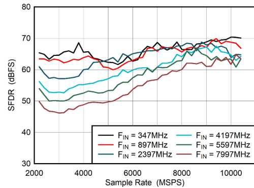
图 6-34. DES Mode: SFDR vs Sample Rate
