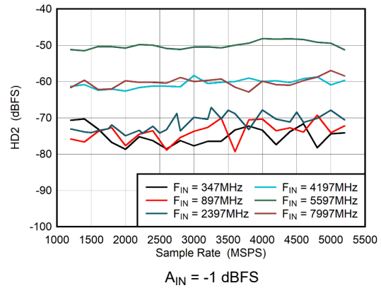
图 6-50. Dual Channel Mode: HD2 vs Sample Rate
