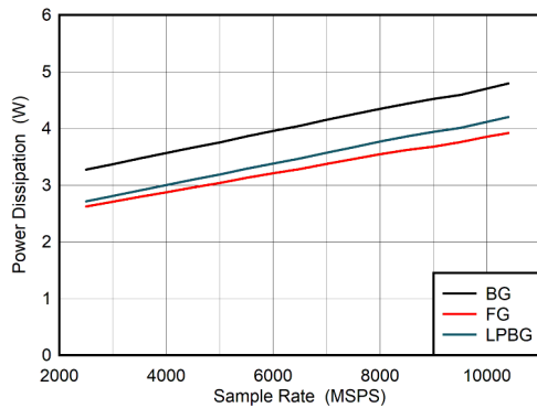
图 6-113. DES Mode: Power Dissipation vs Sample Rate
