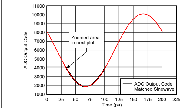
图 6-125. Sinewave Overdrive Recovery
