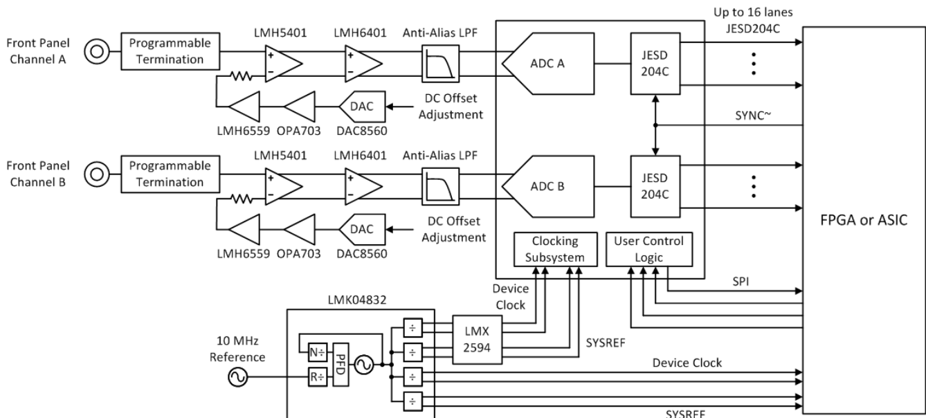
图 8-1. Typical Configuration for Reconfigurable Oscilloscope
