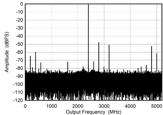
图 6-10. DES Mode: Single Tone FFT at 7997 MHz
