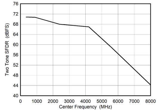
图 6-108. Dual Channel Mode: Two Tone SFDR vs Input Frequency
