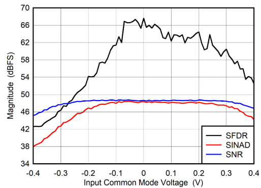
图 6-98. DES Mode: SNR, SFDR and SINAD vs Input Common Mode Voltage
