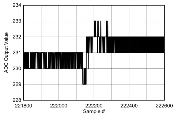
图 6-122. Background Calibration Core Transition (DC Signal Zoomed)
