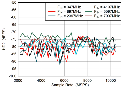
图 6-37. DES Mode: HD2 vs Sample Rate
