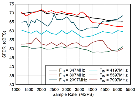
图 6-47. Dual Channel Mode: SFDR vs Sample Rate A_{IN} = -1\text{ dBFS}
