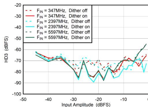
图 6-78. Dual Channel Mode: HD3 vs Input Amplitude and Dither
