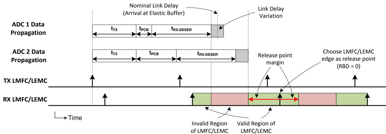
图 7-12. LMFC/LEMC Valid Region Definition for Elastic Buffer Release Point Selection
