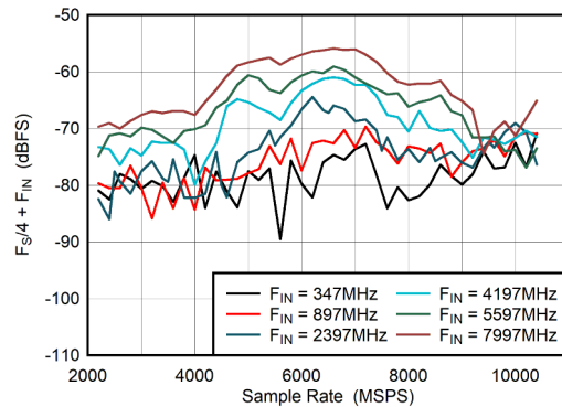
图 6-42. DES Mode: F_S/4 + F_{IN} vs Sample Rate
