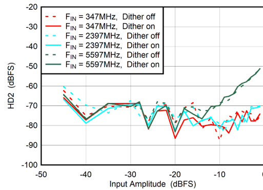
图 6-76. Dual Channel Mode: HD2 vs Input Amplitude and Dither
