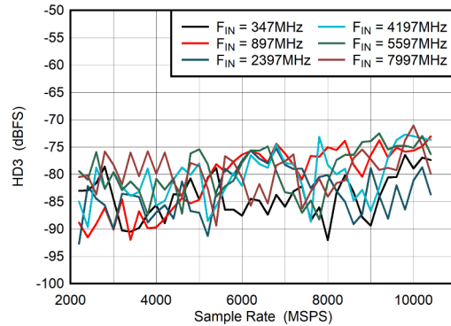
图 6-40. DES Mode: HD3 vs Sample Rate
