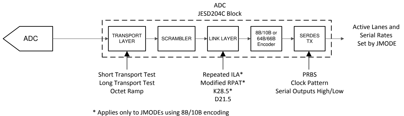
图 7-13. Test Mode Insertion Points
