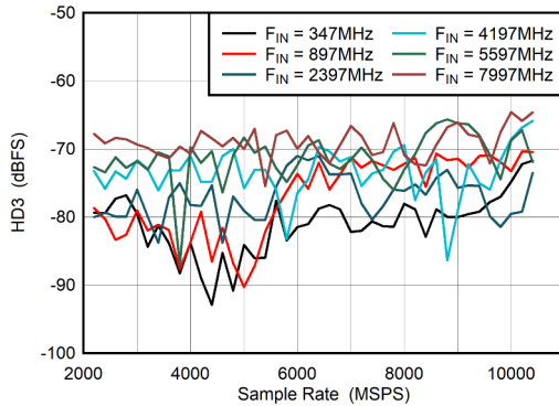
图 6-39. DES Mode: HD3 vs Sample Rate
