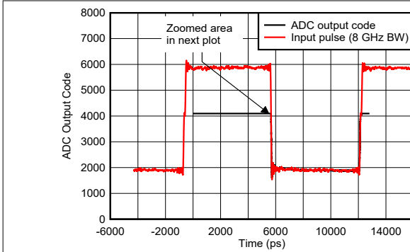
图 6-123. Pulse Overdrive Recovery
