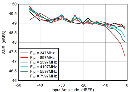
图 6-71. Dual Channel Mode: SNR vs Input Amplitude
