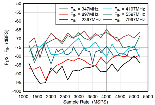
图 6-56. Dual Channel Mode: F_s/2 - F_{IN} vs Sample Rate
