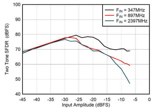
图 6-104. DES Mode: Two Tone SFDR vs Input Amplitude
