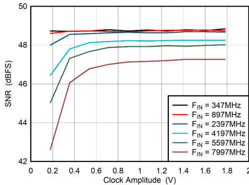
图 6-83. Dual Channel Mode: SNR vs Clock Amplitude
