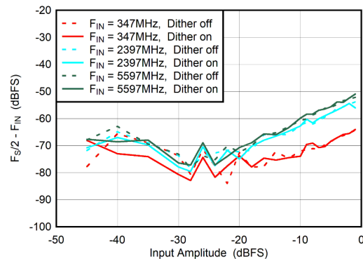
图 6-66. DES Mode: F_s/2 - F_{IN} vs Input Amplitude and Dither
