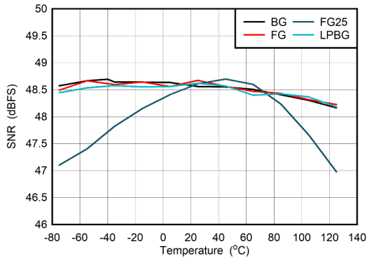
图 6-91. Dual Channel Mode: SNR vs Temperature and Calibration
