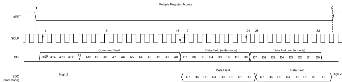
图 7-16. Serial Interface Protocol: Streaming Read/Write
