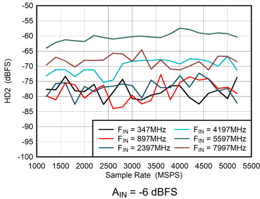
图 6-51. Dual Channel Mode: HD2 vs Sample Rate
