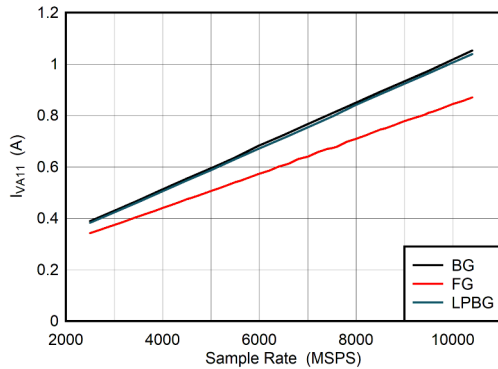
图 6-111. DES Mode: I_{VA11} vs Sample Rate
