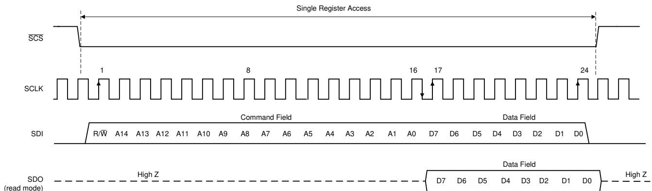
图 7-15. Serial Interface Protocol: Single Read/Write
