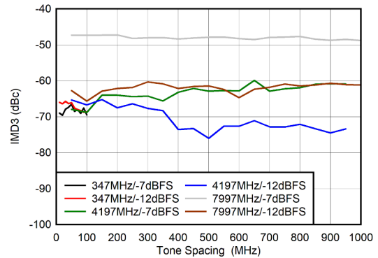
图 6-102. DES Mode: IMD3 vs Tone Spacing
