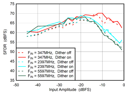
图 6-60. DES Mode: SFDR vs Input Amplitude and Dither
