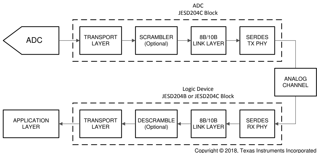
图 7-8. Simplified 8B/10B Encoded JESD204C Interface Diagram
