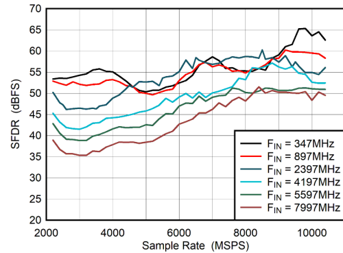
图 6-32. DES Mode: SFDR vs Sample Rate
