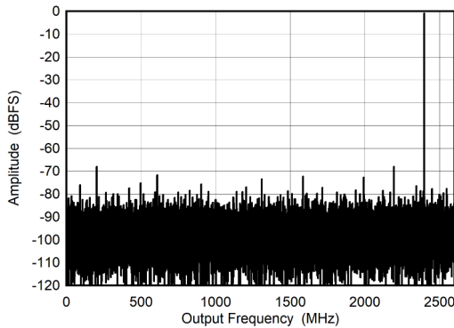
图 6-19. Dual Channel Mode: Single Tone FFT at 2397 MHz
