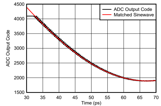
图 6-126. Sinewave Overdrive Recovery
