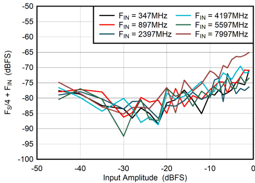
图 6-67. DES Mode: F_S/4 + F_{IN} vs Input Amplitude
