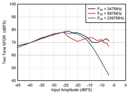
图 6-109. Dual Channel Mode: Two Tone SFDR vs Input Amplitude
