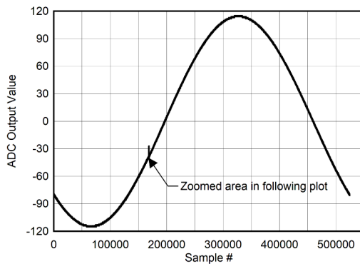
图 6-119. Background Calibration Core Transition (AC Signal)
