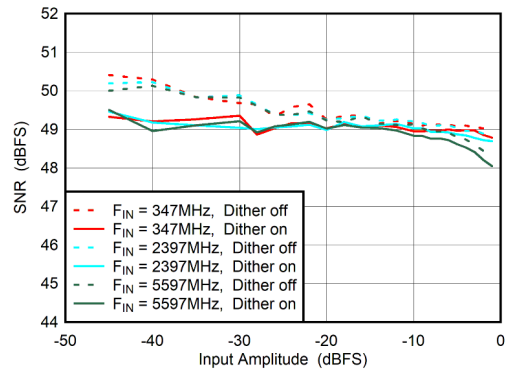
图 6-58. DES Mode: SNR vs Input Amplitude and Dither
