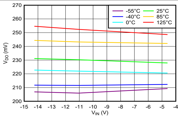
I_{OUT} = 500\text{ mA} C_{IN} = 30\ \mu\text{F} 图 6-9. Dropout Voltage vs Input Voltage Across Temperature
