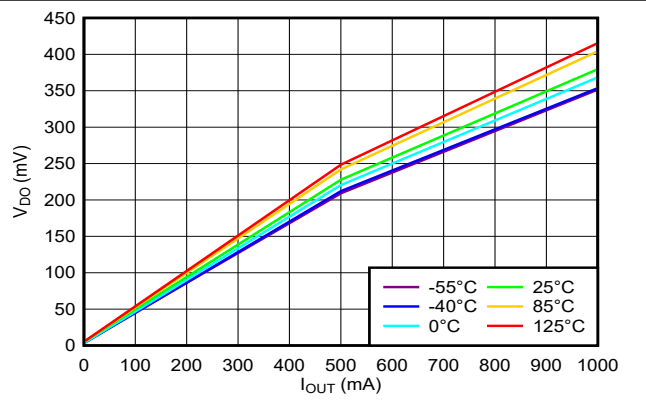
V_{IN} = -4.6\text{ V} V_{OUT(SET)} = -5\text{ V} C_{IN} = 30\ \mu\text{F} 图 6-10. Dropout Voltage vs Output Current Across Temperature
