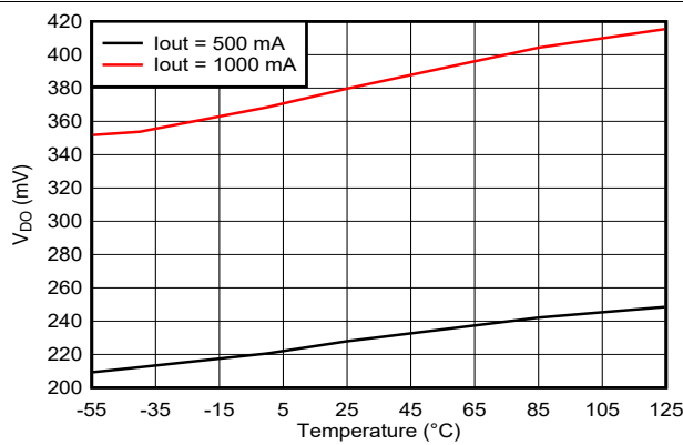
V_{IN} = -4.6\text{ V} V_{OUT(SET)} = -5\text{ V} C_{IN} = 30\ \mu\text{F} 图 6-11. Dropout Voltage vs Temperature Across Output Current
