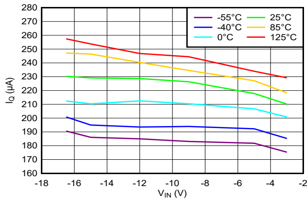
I_{OUT} = 0\text{ mA} 图 6-7. Quiescent Current vs Input Voltage Across Temperature
