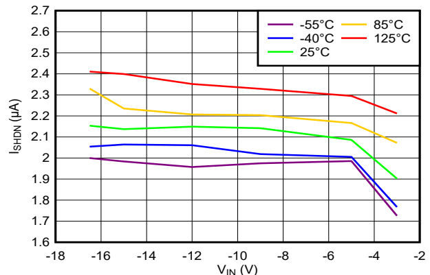
V_{EN} = 0.4\text{ V} 图 6-8. Shutdown Current vs Input Voltage Across Temperature
