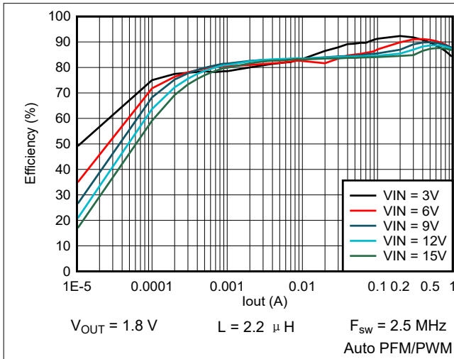
图 9-26. Efficiency vs Output Current
