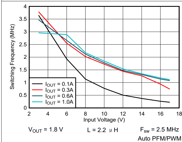
图 9-28. Switching Frequency vs Input Voltage
