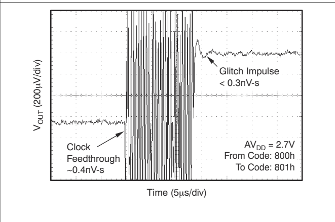
图 7-67. Glitch Energy, 2.7-V, 12-Bit, 1-LSB Step, Rising Edge
