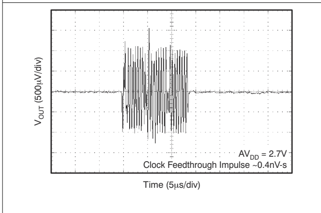
图 7-66. Clock Feedthrough 2.7-V, 20-MHz, Midscale
