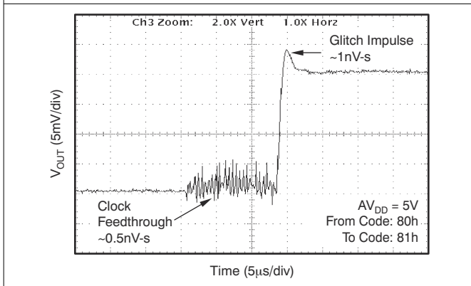
图 7-26. Glitch Energy, 5-V, 12-Bit, 1-LSB Step, Rising Edge
