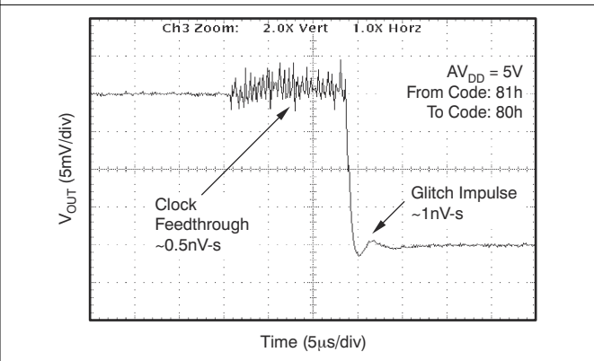
图 7-27. Glitch Energy, 5-V, 12-Bit, 1-LSB Step, Falling Edge
