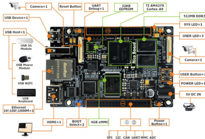
图 7. Rico Board Top View
