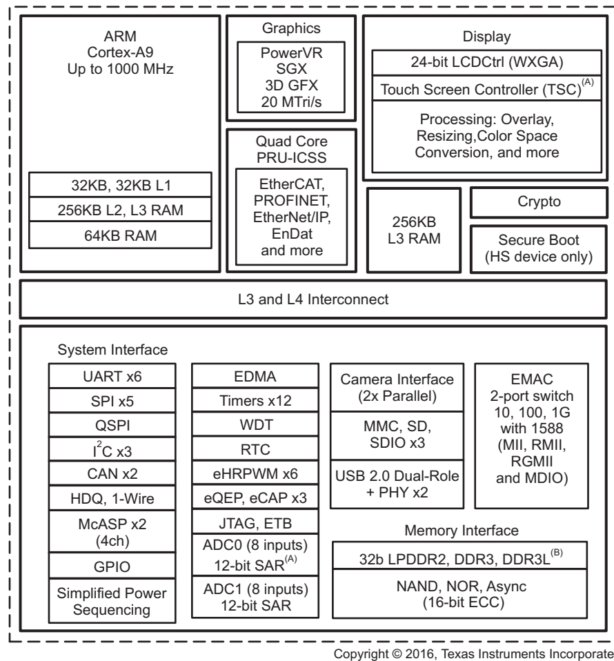
图 4. AM437x Functional Block Diagram
