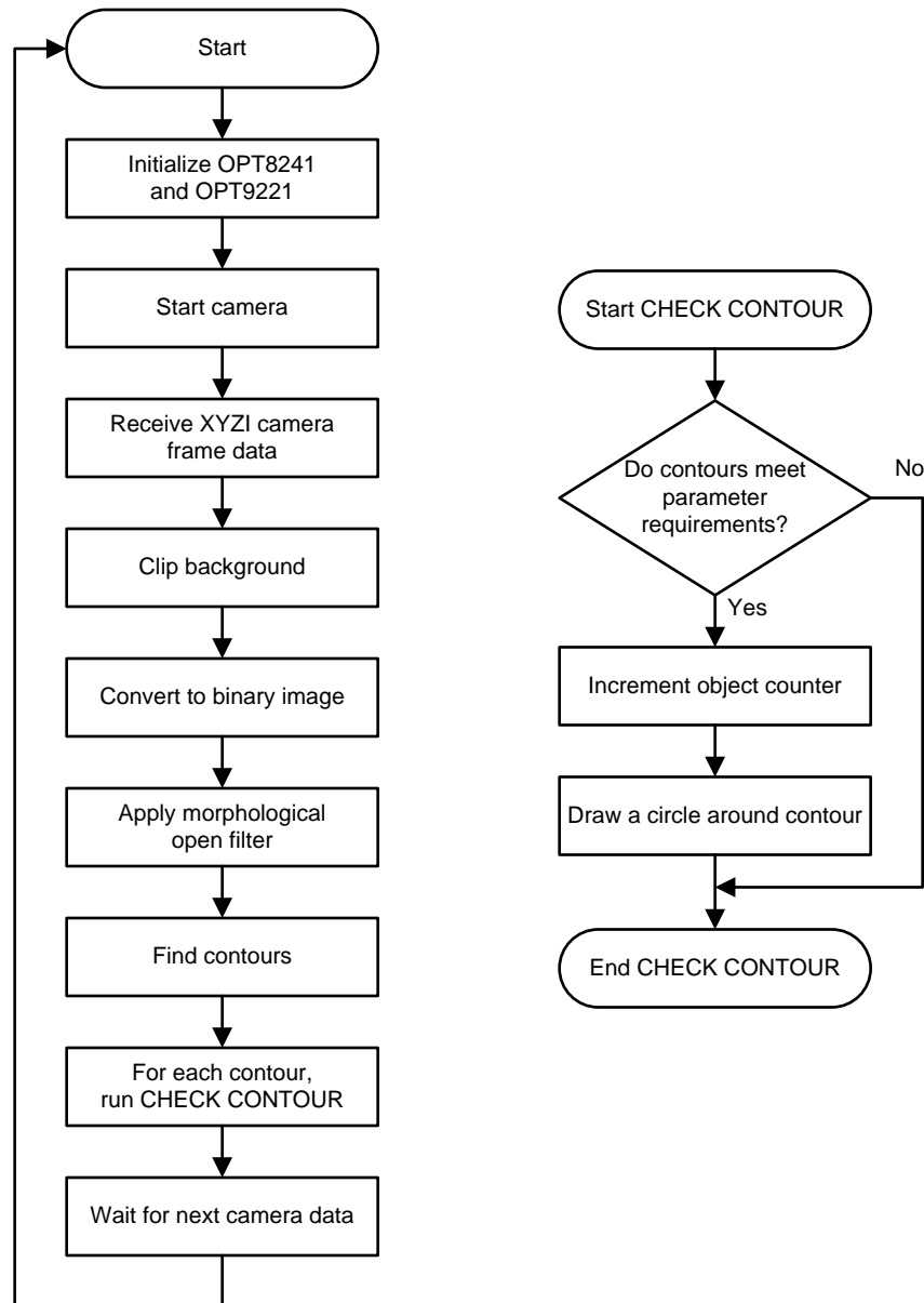
图 23. Simple People Tracking Algorithm Flowchart
