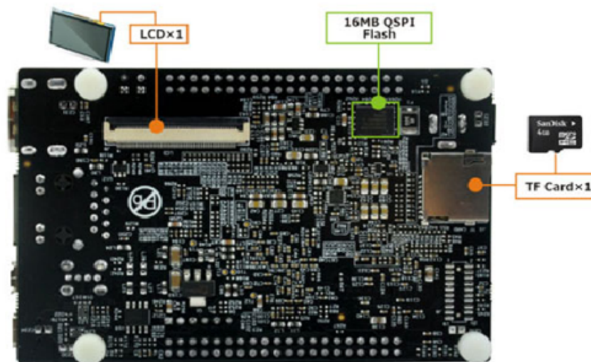
图 8. Rico Board Bottom View
