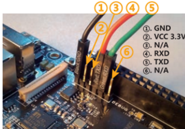
图 16. Rico Board UART Connection
