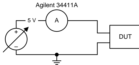
图 24. Test Circuit Used for Measuring Supply Current
