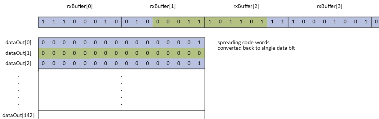
图 11. DataOut[] Buffer Converted into “0” or “1” for all 142 Groups
