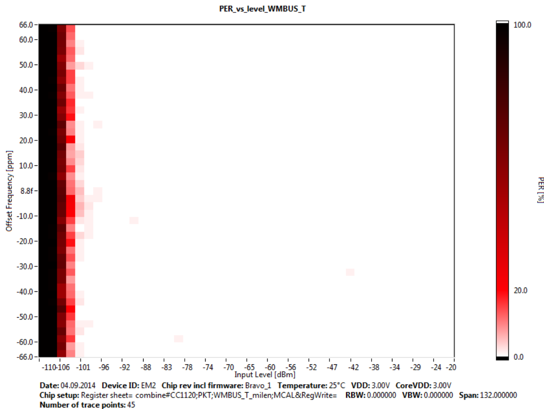
图 12. T-Mode Receive Operation With CC1125 With 10-Byte Payload, 100 kcps, 2-FSK, and Frequency = 868.95 MHz
