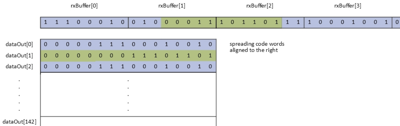
图 10. DataOut[] Buffer Filled Up With 11-Bit Spreading Sequence
