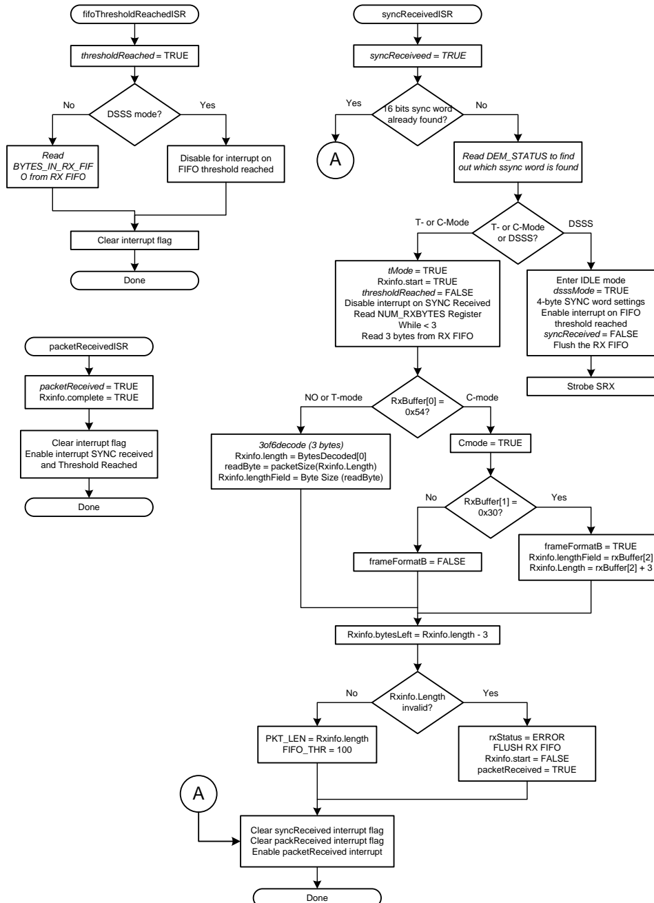
图 9. Flow Chart of Interrupt Functions in TIDC-DSSS868WMBUS-DC Firmware
