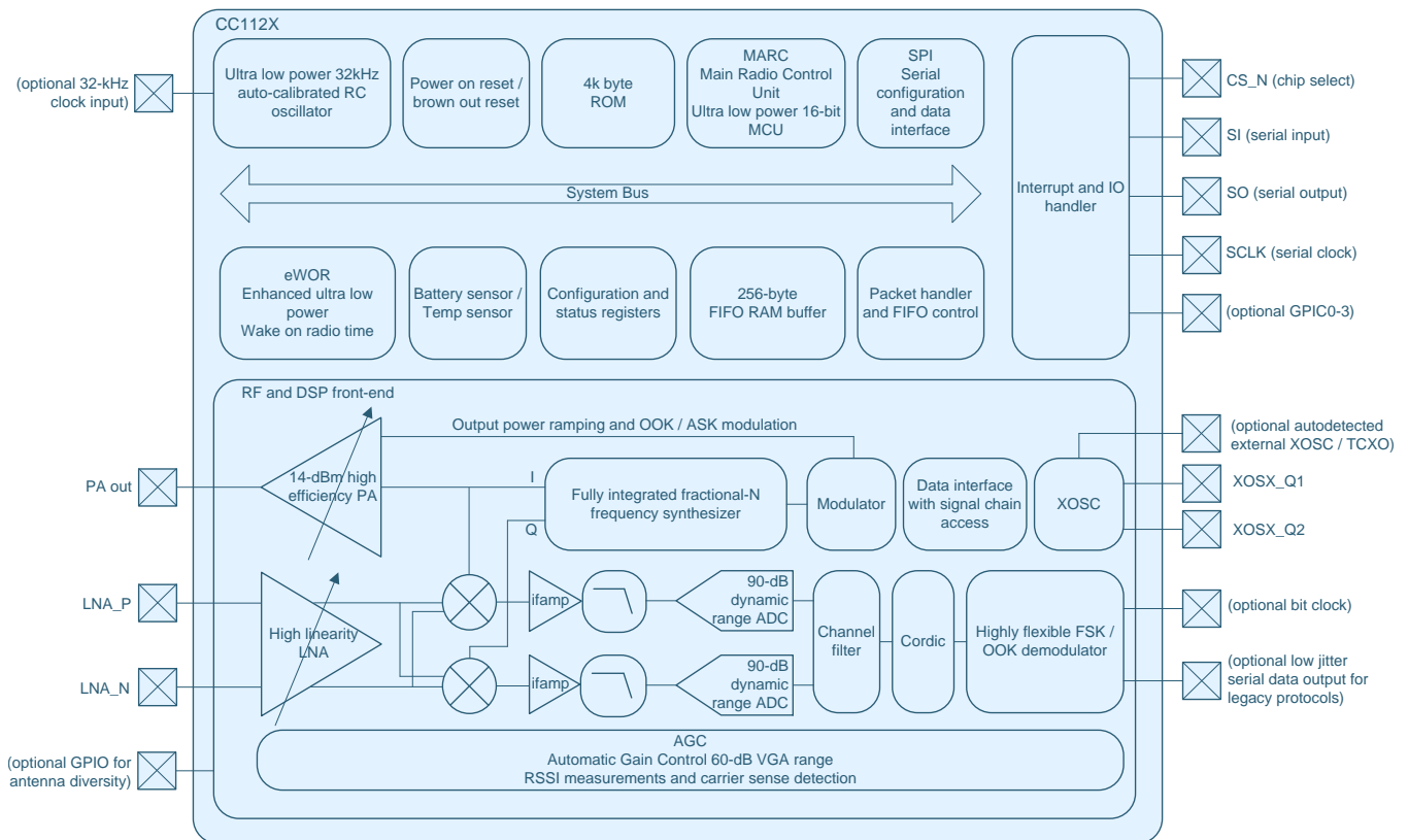
图 2. CC1125 Functional Block Diagram
