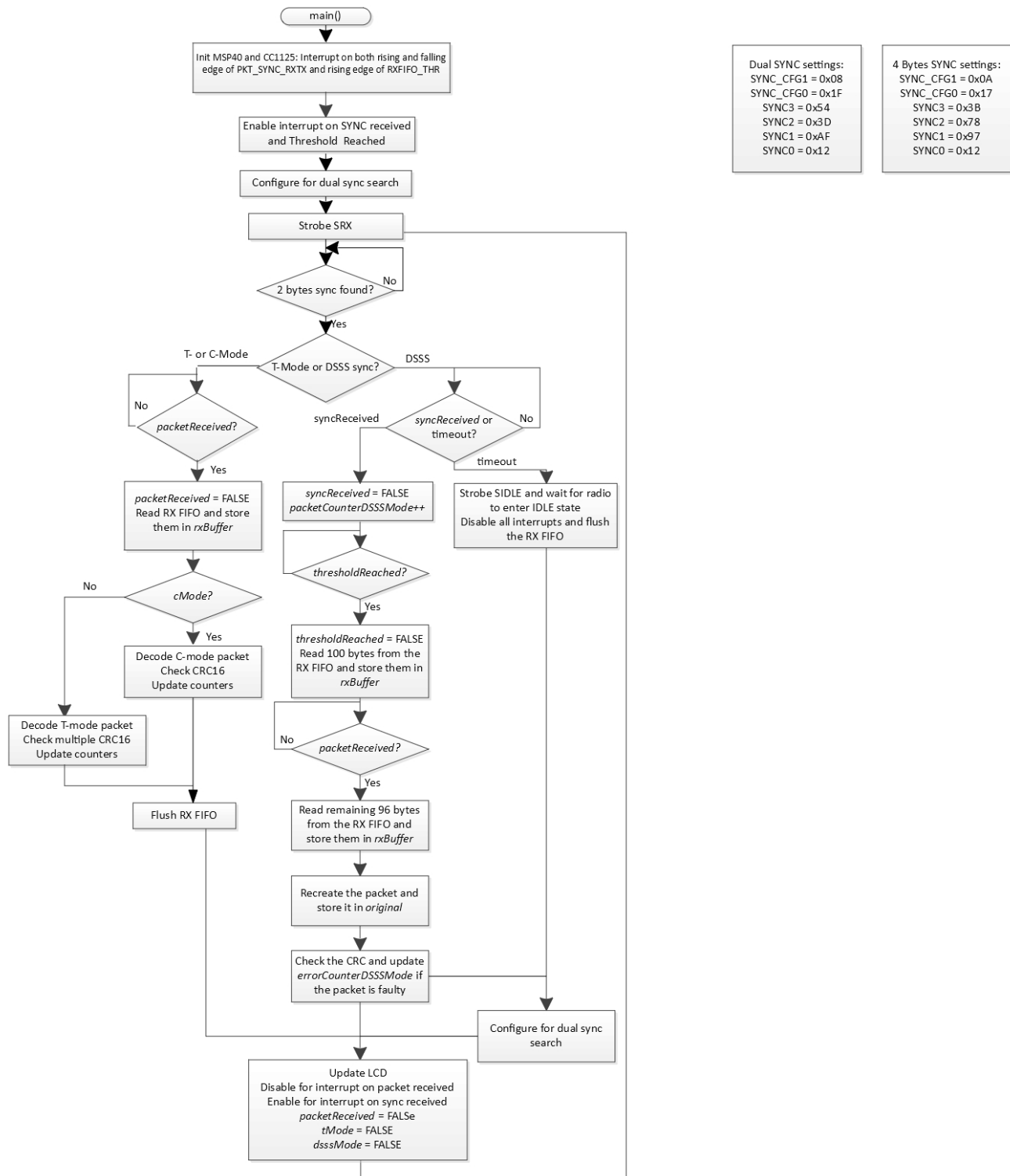
图 8. Flow Chart of main() Function in TIDC-DSSS868WMBUS-DC Firmware
