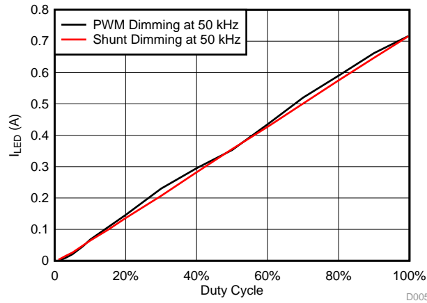
图 31. I_{LED} (A) versus Duty Cycle (%) for PWM or Shunt Dimming at 50 kHz for Red LED String
