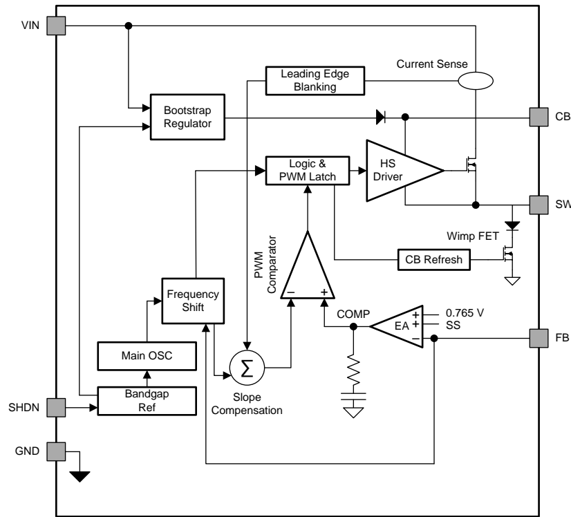
图 9. Functional Block Diagram of LMR16006
