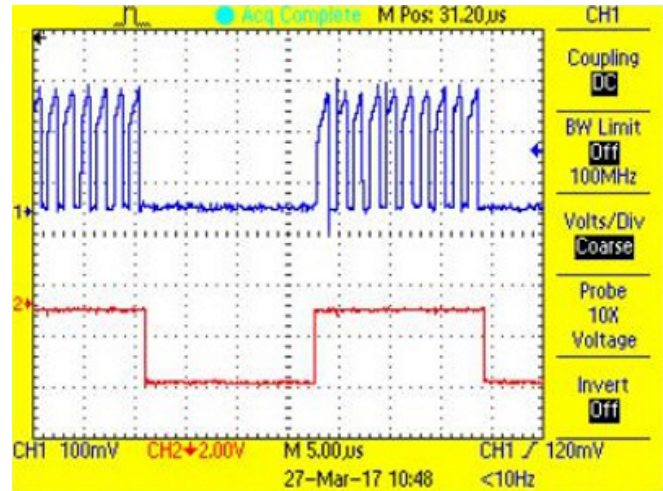
图 48. P-FET Current During On-Time and Shunt PWM Waveform for Red LED String at 50% Duty Cycle
