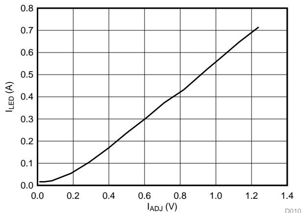
图 23. I_{LED} (A) versus I_{ADJ} (V) for Red LED String
