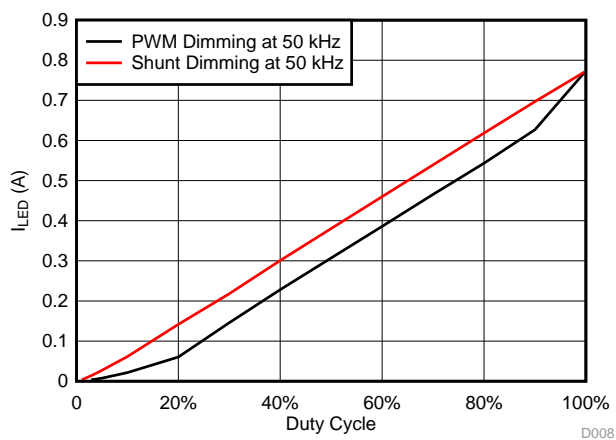
图 34. I_{LED} (A) versus Duty Cycle (%) for PWM or Shunt Dimming at 50 kHz for White LED String
