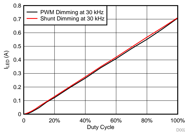
图 28. I LED (A) versus Duty Cycle (%) for PWM or Shunt Dimming at 30 kHz for Green LED String
