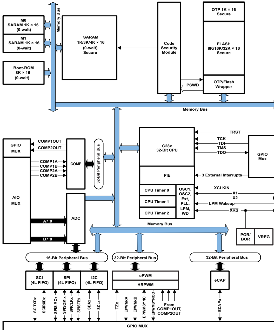
图 8. Functional Block Diagram of C2000
