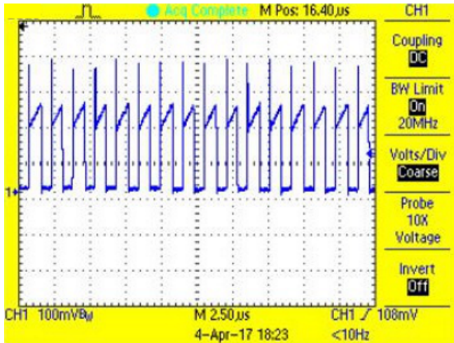
图 35. P-FET Current During On-Time at I_{ADJ} = 1.24\text{ V} for Red String
