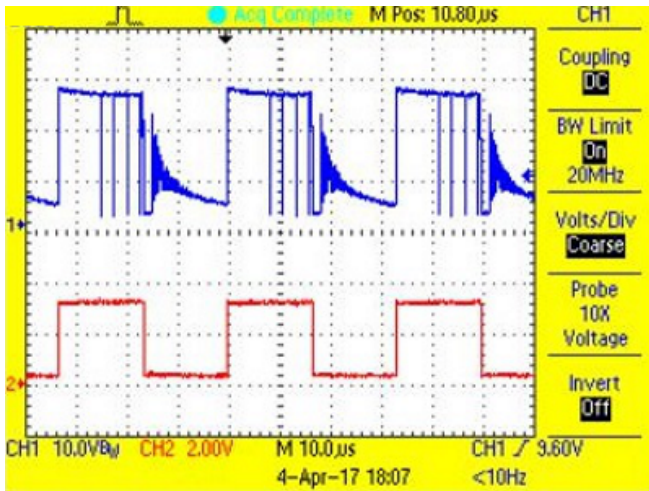
图 45. Switch Node and PWM Waveform for White LED String at 50% Duty Cycle
