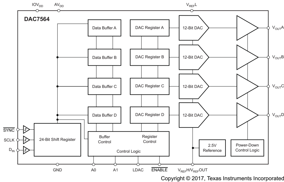
图 6. Functional Block Diagram of DAC7564
