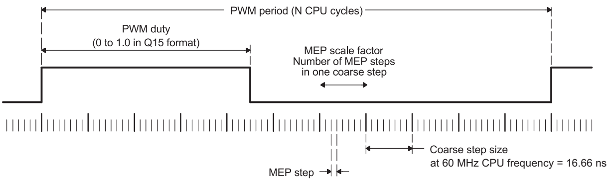
图 16. Conventional PWM and HRPWM Timing Diagram
