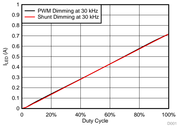
图 27. I_{LED} (A) versus Duty Cycle (%) for PWM or Shunt Dimming at 30 kHz for Red LED String
