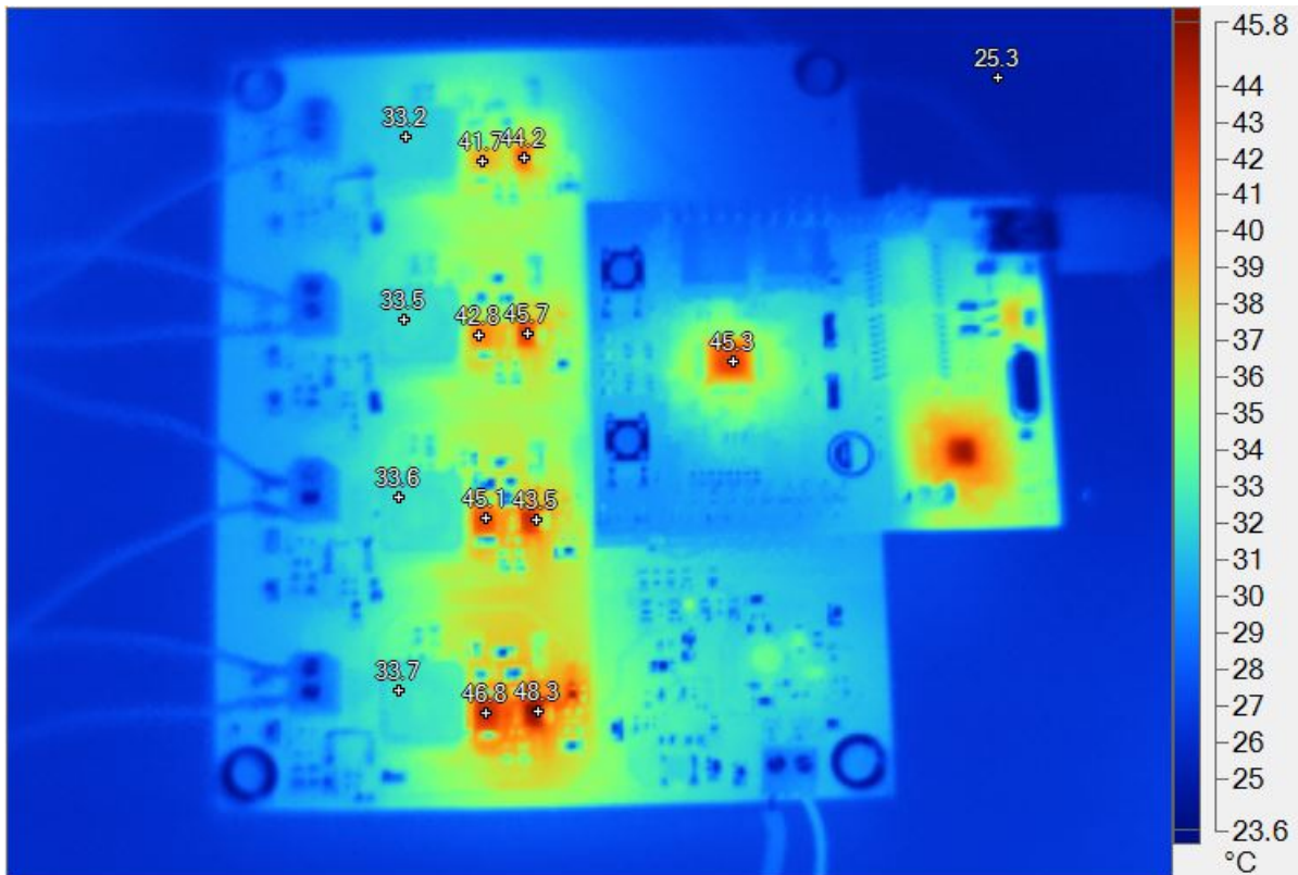
图 61. Thermal Image of Top Side of TIDA-01415 Board for Shunt Dimming at 2.9-A Total LED Current (100% Duty Cycle for All Strings)
