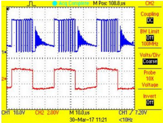
图 43. Switch Node and PWM Waveform for Blue LED String at 50% Duty Cycle
