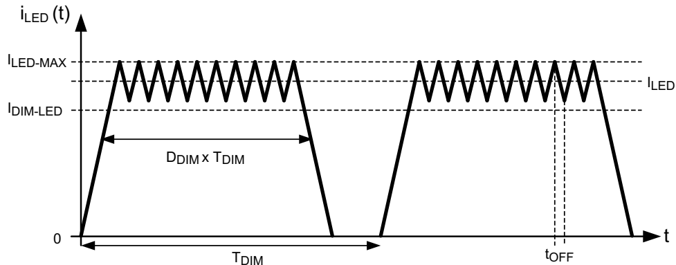
图 15. LED Current i_{LED}(t) During EN Pin PWM Dimming
