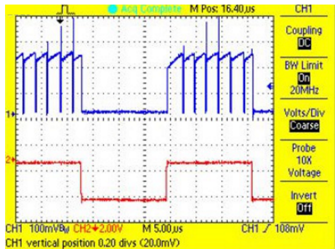
图 54. P-FET Current During On-Time and Shunt PWM Waveform for White LED String at 50% Duty Cycle
