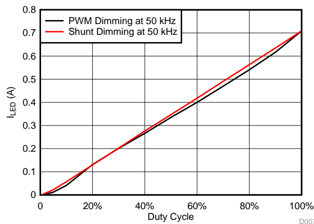
图 33. I LED (A) versus Duty Cycle (%) for PWM or Shunt Dimming at 50 kHz for Blue LED String
