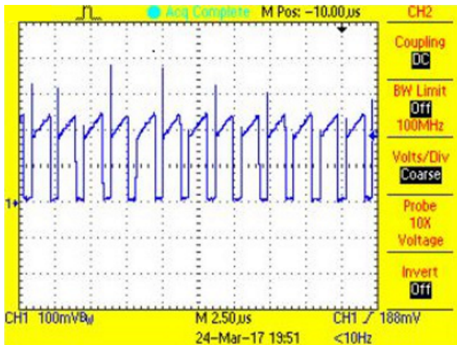
图 37. P-FET Current During On-Time at I_{ADJ} = 1.24\text{ V} for Blue String
