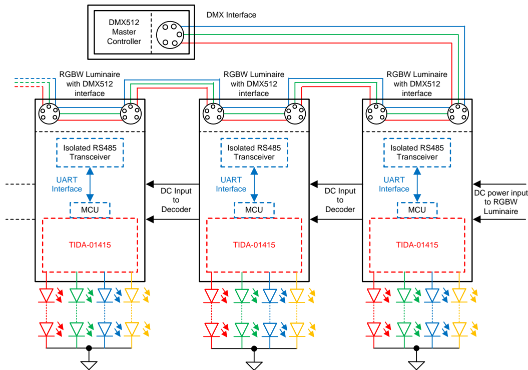
图 1. TIDA-01415 End Application in Stage Lighting
