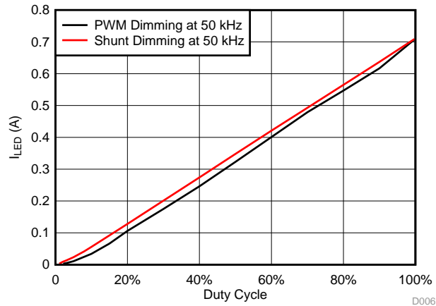
图 32. I LED (A) versus Duty Cycle (%) for PWM or Shunt Dimming at 50 kHz for Green LED String
