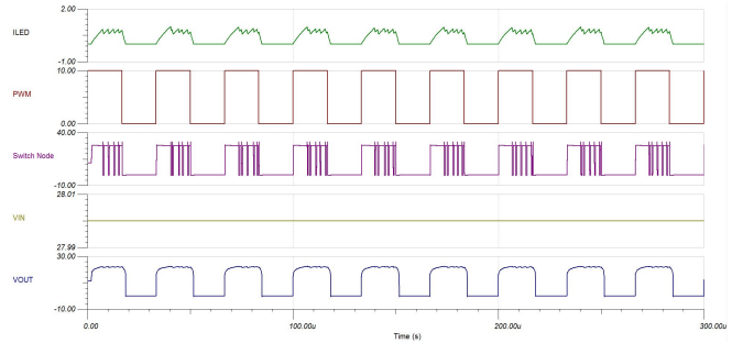
图 56. Simulation Results for PWM Dimming at 30 kHz
