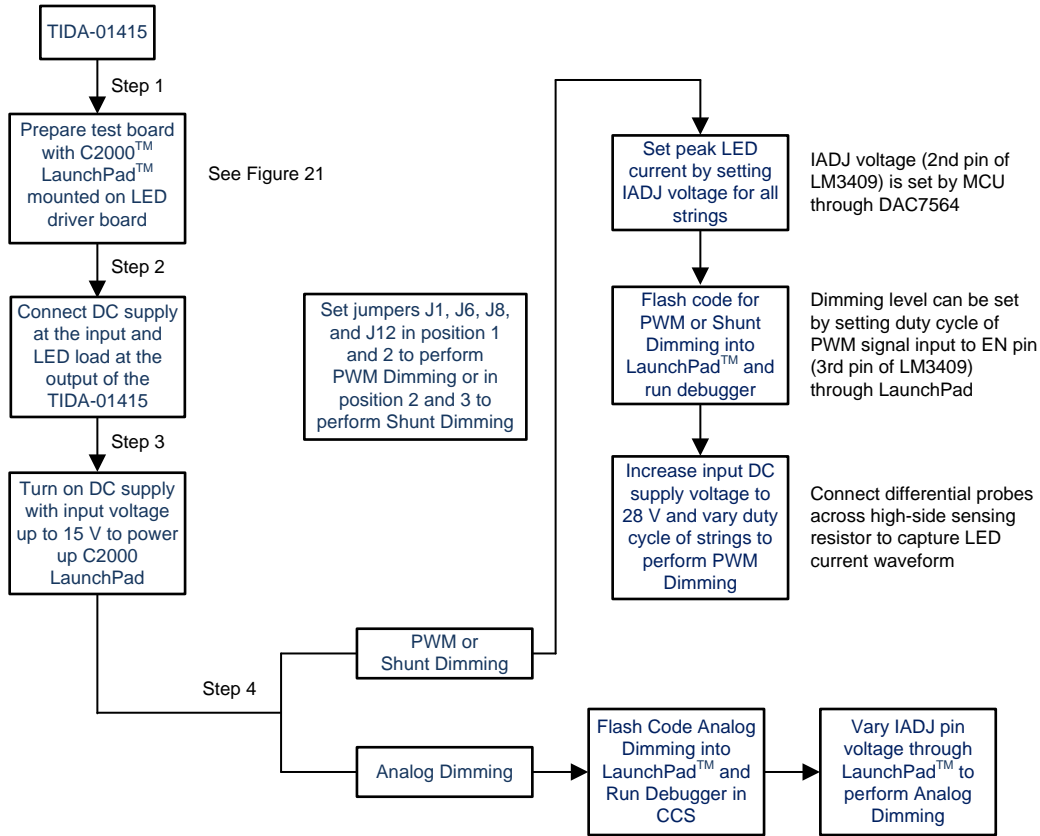
图 22. Test Flow to Perform Analog Dimming and PWM or Shunt Dimming Through TIDA-01415
