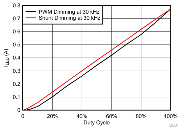
图 30. I LED (A) versus Duty Cycle (%) for PWM or Shunt Dimming at 30 kHz for White LED String
