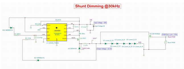
图 57. Simulation Circuit for Shunt Dimming at 30 kHz With LM3409
