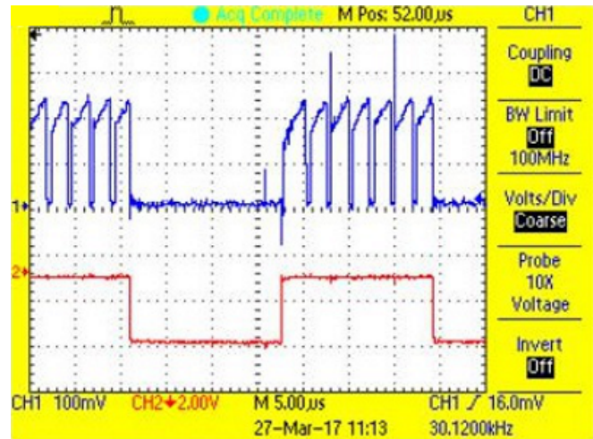
图 50. P-FET Current During On-Time and Shunt PWM Waveform for Green LED String at 50% Duty Cycle
