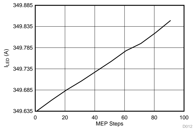
图 18. I_{LED} versus MEP Steps for Green LED String at 30-kHz Shunt Dimming Frequency
