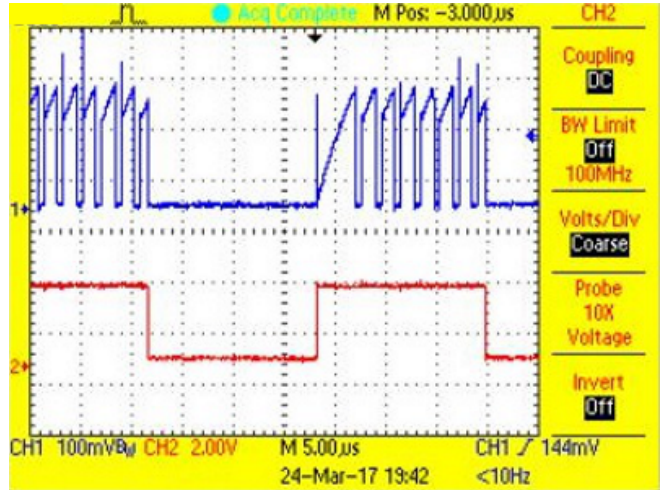
图 44. P-FET Current During On-Time and PWM Waveform for Blue LED String at 50% Duty Cycle
