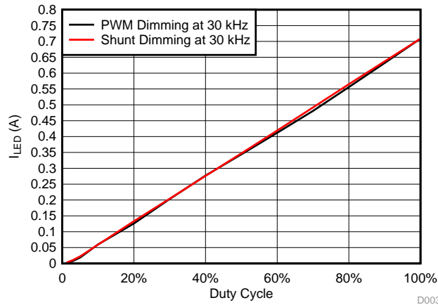
图 29. I LED (A) versus Duty Cycle (%) for PWM or Shunt Dimming at 30 kHz for Blue LED String
