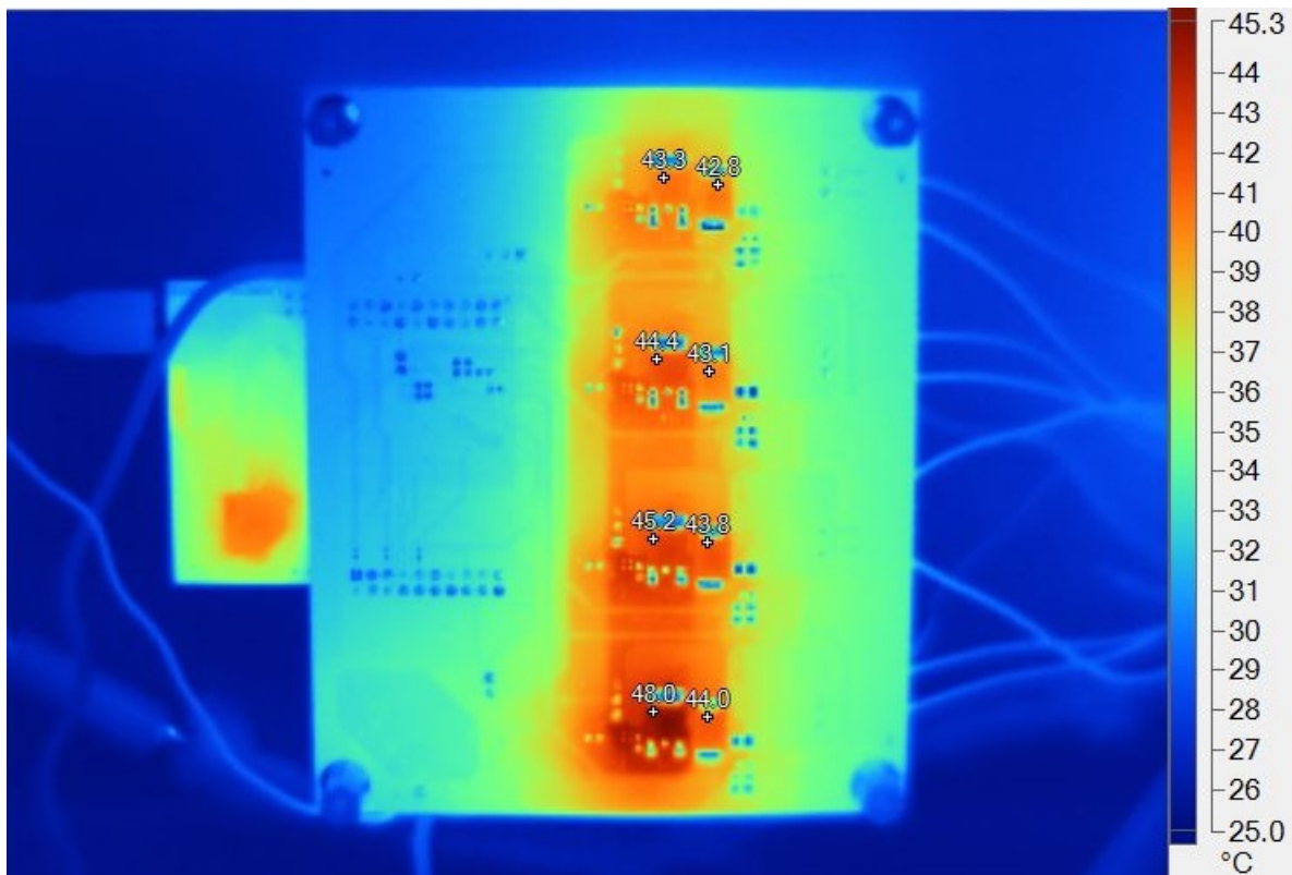
图 60. Thermal Image of Bottom Side of TIDA-01415 Board for PWM Dimming at 2.9-A Total LED Current (100% Duty Cycle for All Strings)
