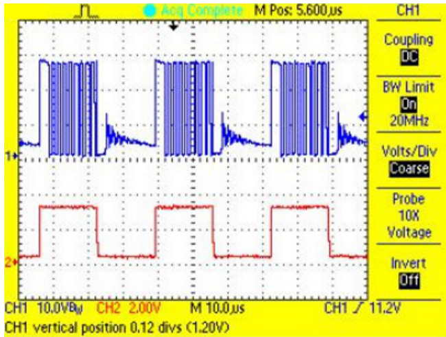
图 39. Switch Node and PWM Waveform for Red LED String at 50% Duty Cycle
