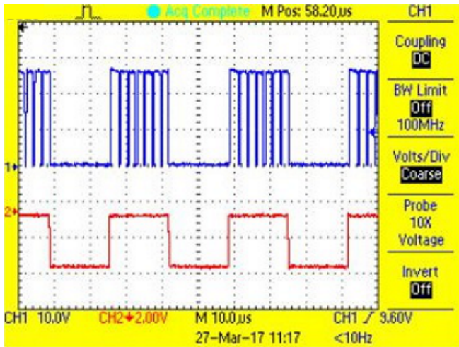
图 49. Switch Node and Shunt PWM Waveform for Green LED String at 50% Duty Cycle
