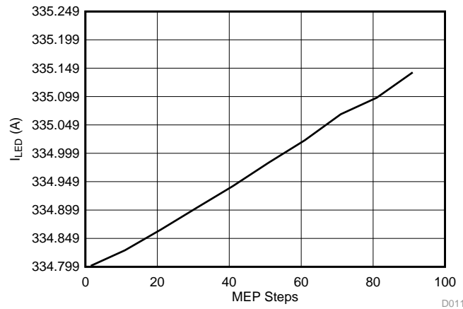
图 17. I_{LED} versus MEP Steps for Green LED String at 30-kHz PWM Dimming Frequency
