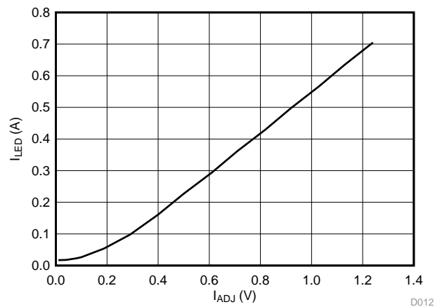
图 25. I_{LED} (A) versus I_{ADJ} (V) for Blue LED String
