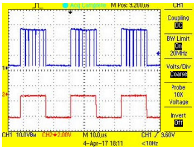
图 53. Switch Node and Shunt PWM Waveform for White LED String at 50% Duty Cycle
