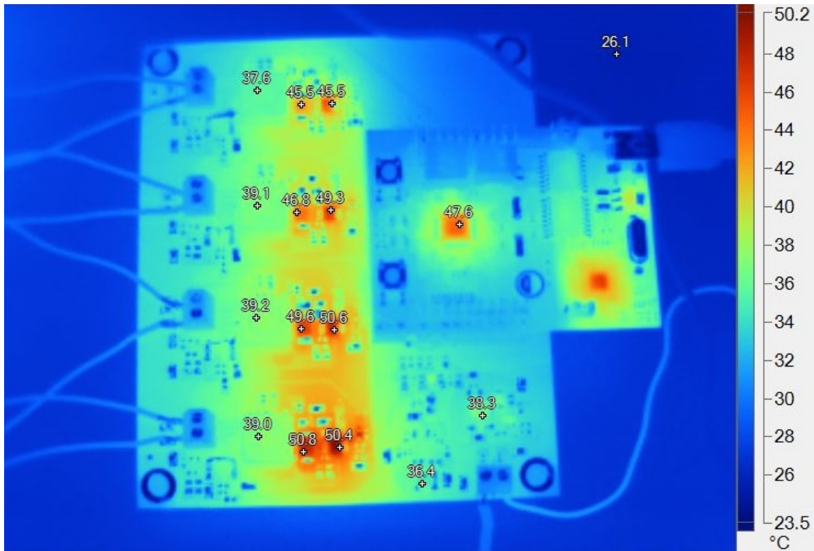
图 59. Thermal Image of Top Side of TIDA-01415 Board for PWM Dimming at 2.9-A Total LED Current (100% Duty Cycle for All Strings)
