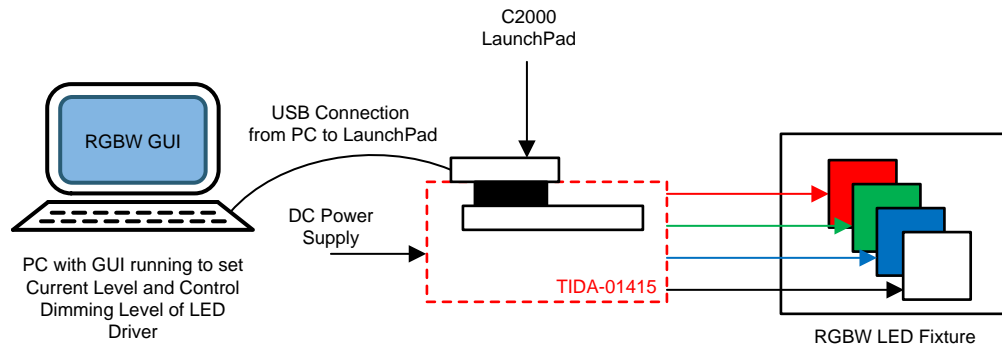
图 20. Hardware Interconnections of TIDA-01415
