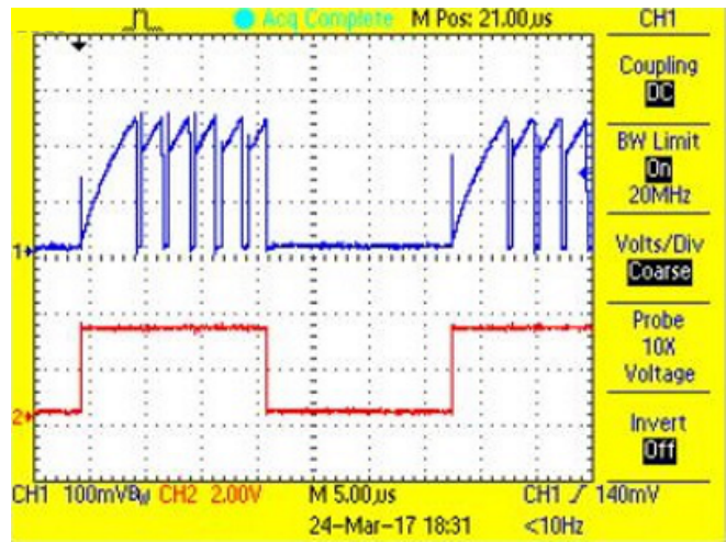
图 42. P-FET Current During On-Time and PWM Waveform for Green LED String at 50% Duty Cycle
