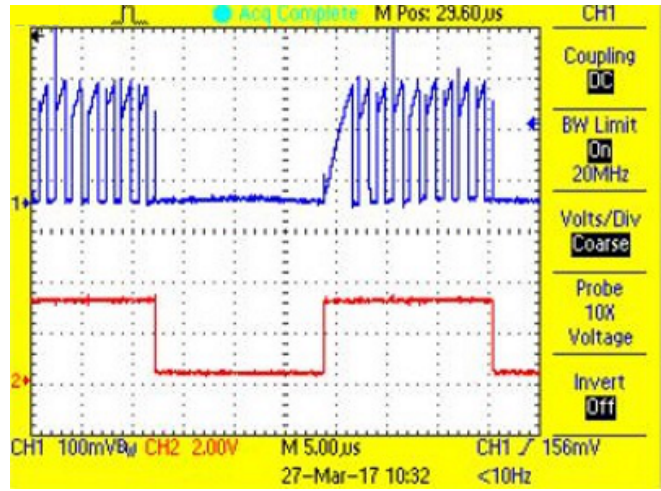
图 40. P-FET Current During On-Time and PWM Waveform for Red LED String at 50% Duty Cycle
