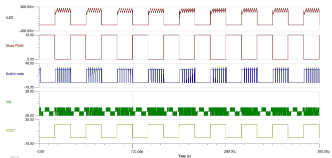
图 58. Simulation Results for Shunt Dimming at 30 kHz
