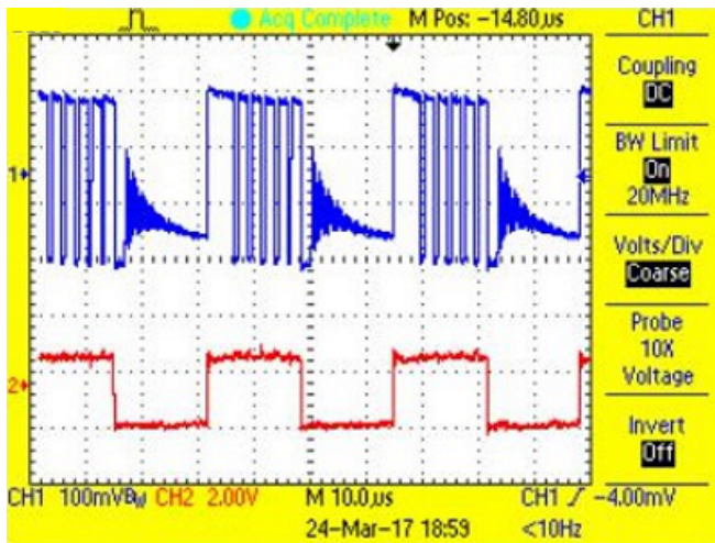
图 41. Switch Node and PWM Waveform for Green LED String at 50% Duty Cycle
