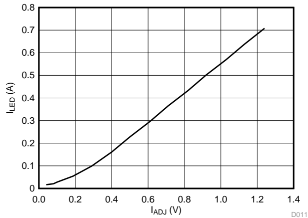
图 24. I_{LED} (A) versus I_{ADJ} (V) for Green LED String
