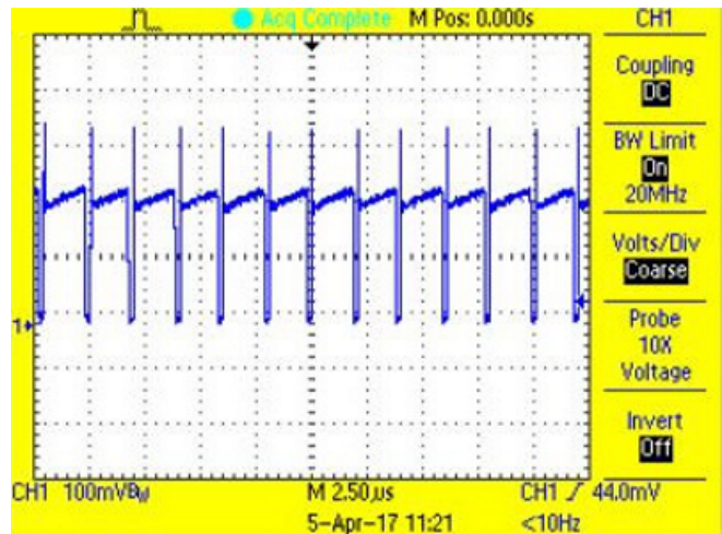
图 38. P-FET Current During On-Time at I_{ADJ} = 1.24\text{ V} for White String
