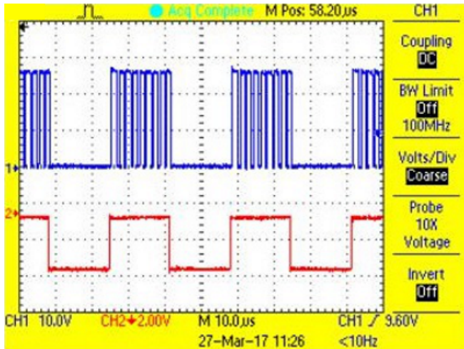
图 51. Switch Node and Shunt PWM Waveform for Blue LED String at 50% Duty Cycle
