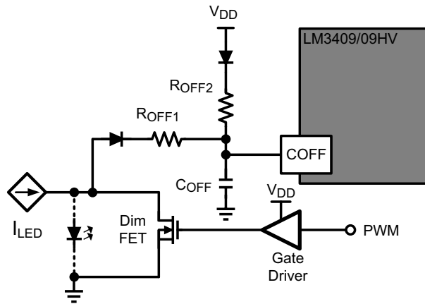
图 14. External Parallel FET Dimming Circuit
