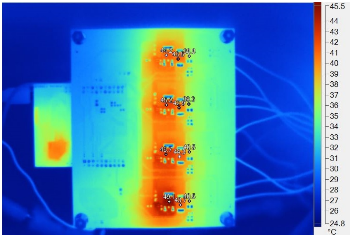
图 62. Thermal Image of Bottom Side of TIDA-01415 Board for Shunt Dimming at 2.9-A Total LED Current (100% Duty Cycle for All Strings)
