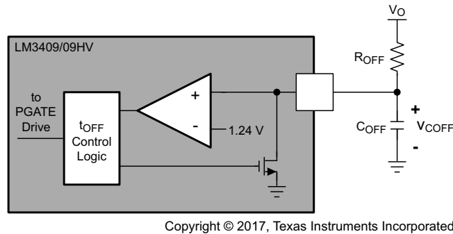
图 12. Off-Time Control Circuit
