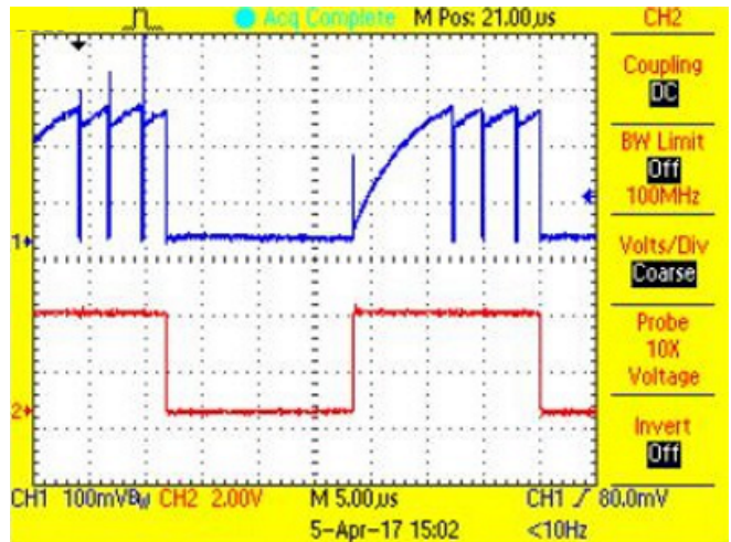
图 46. P-FET Current During On-Time and PWM Waveform for White LED String at 50% Duty Cycle
