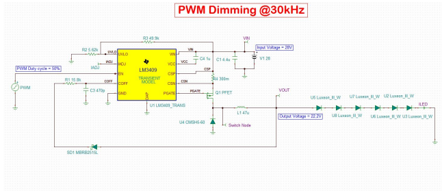
图 55. Simulation Circuit for PWM Dimming With LM3409
