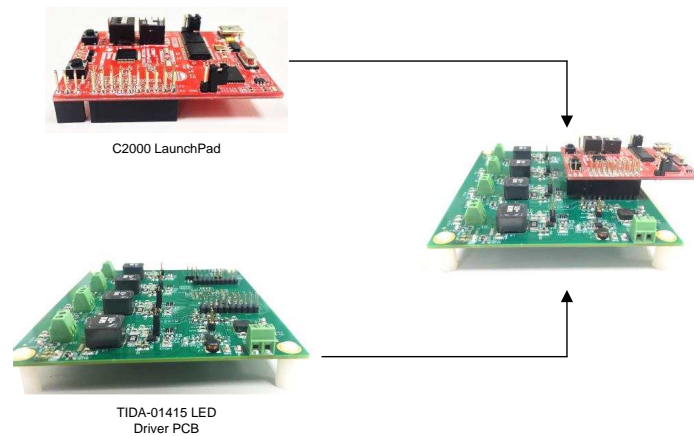
图 21. C2000 LaunchPad Mounted on TIDA-01415 LED Driver Board
