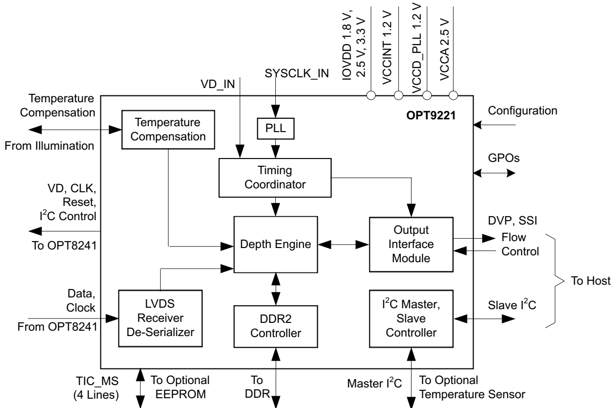
图 3. OPT9221 Functional Block Diagram
