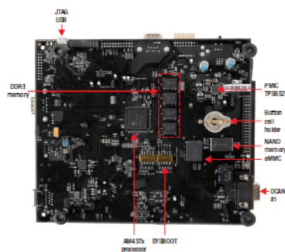
图 8. AM437x GP EVM Bottom View
