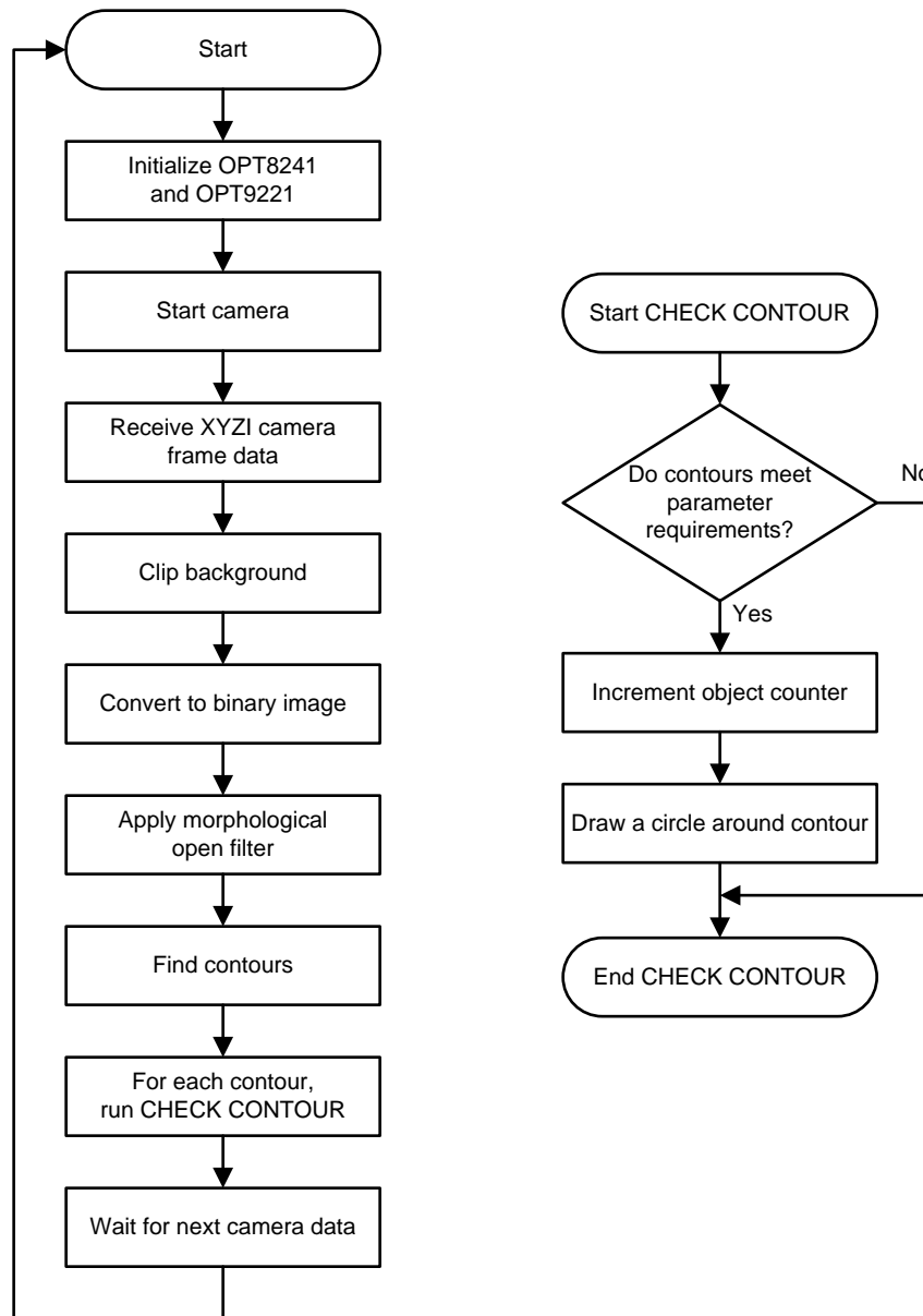
图 20. Simple People Tracking Algorithm Flow Chart
