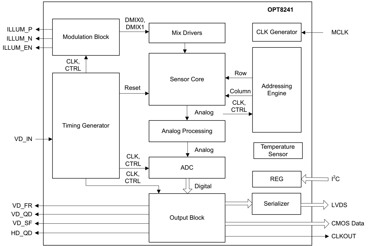
图 2. OPT8241 Functional Block Diagram
