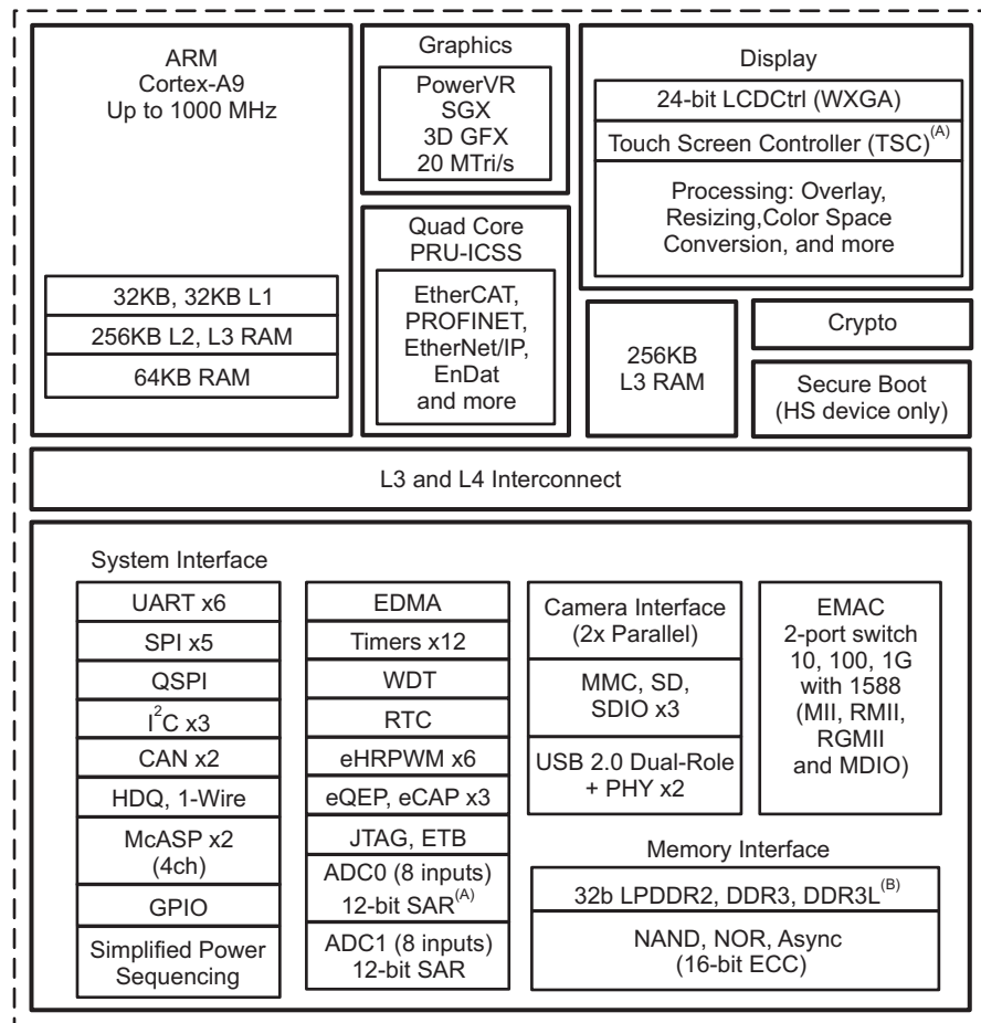
图 4. AM437x Functional Block Diagram
