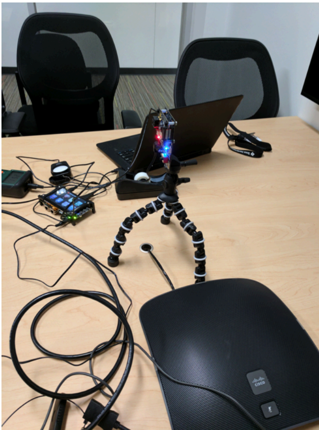
图 23. OPT8241 CDK and AM437x GP EVM With Tripod
