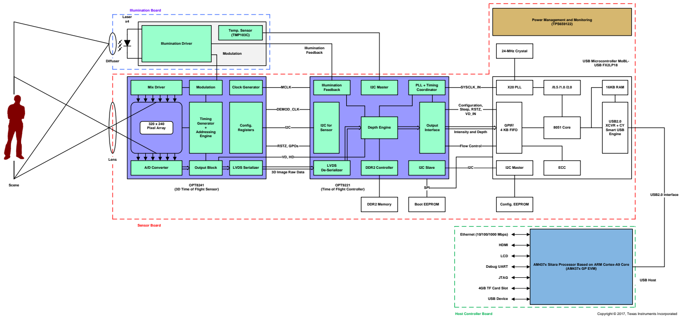
图 1. Block Diagram of TIDA-01436
