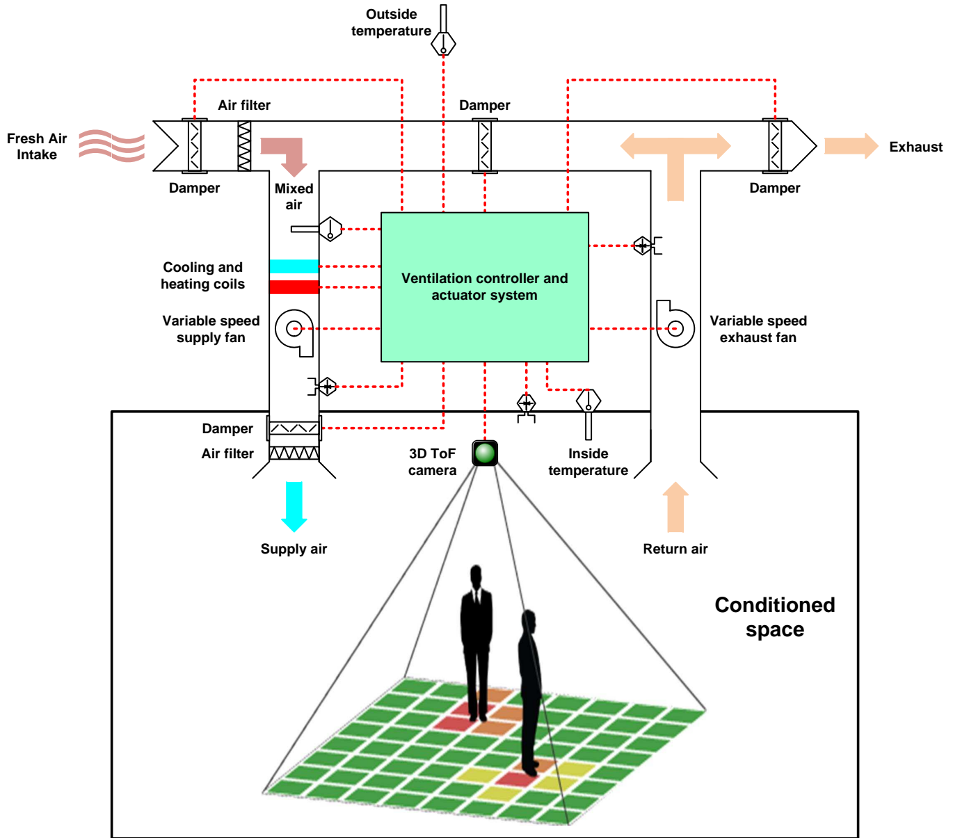
图 9. 3D ToF Camera Based DCV System
