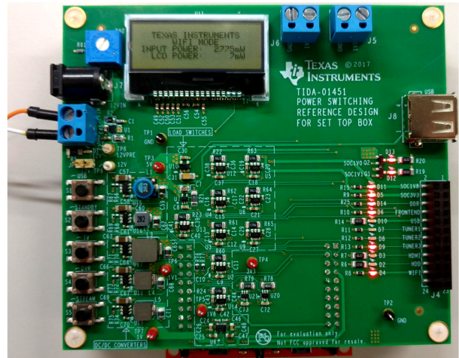
图 15. Standby Button LEDs (All LEDs OFF Except USB)
