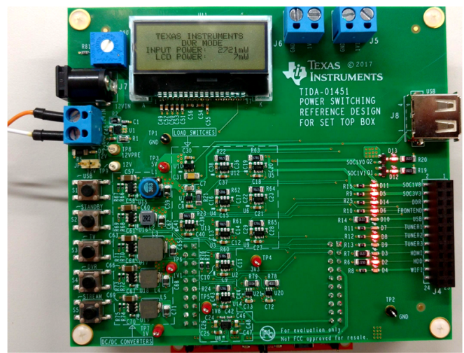
图 13. DVR Button LEDs (HDD, Tuner2, Front End, SOC+DDR)
