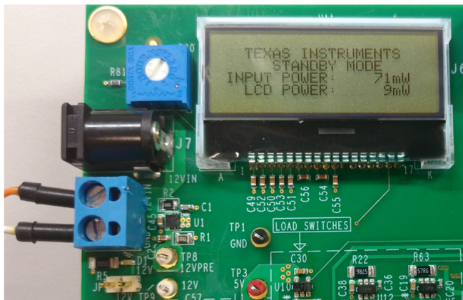
图 16. LCD at Lowest Brightness
