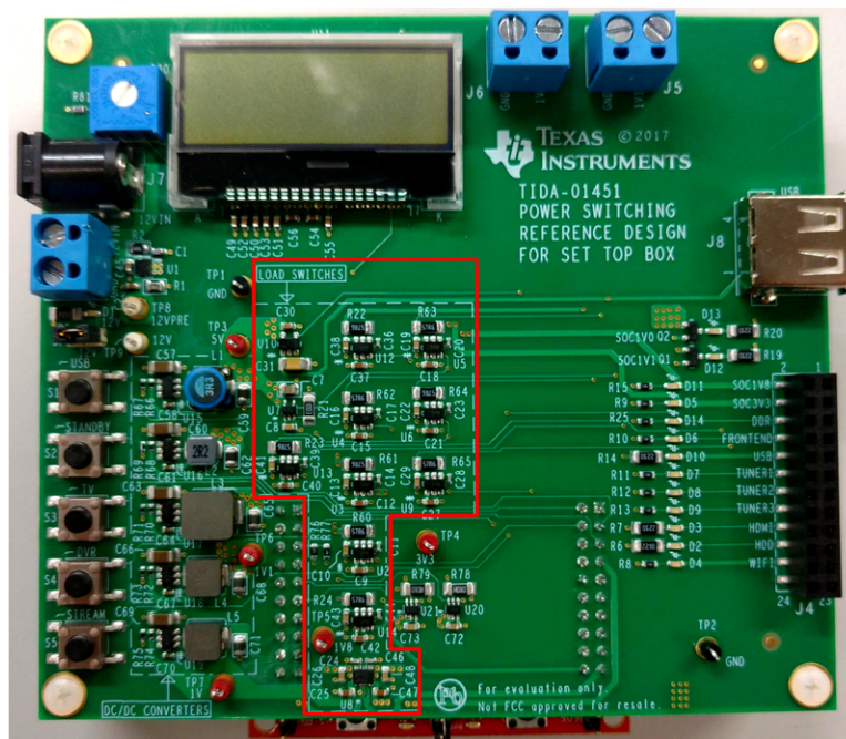
图 2. "LOAD SWITCHES" Area
