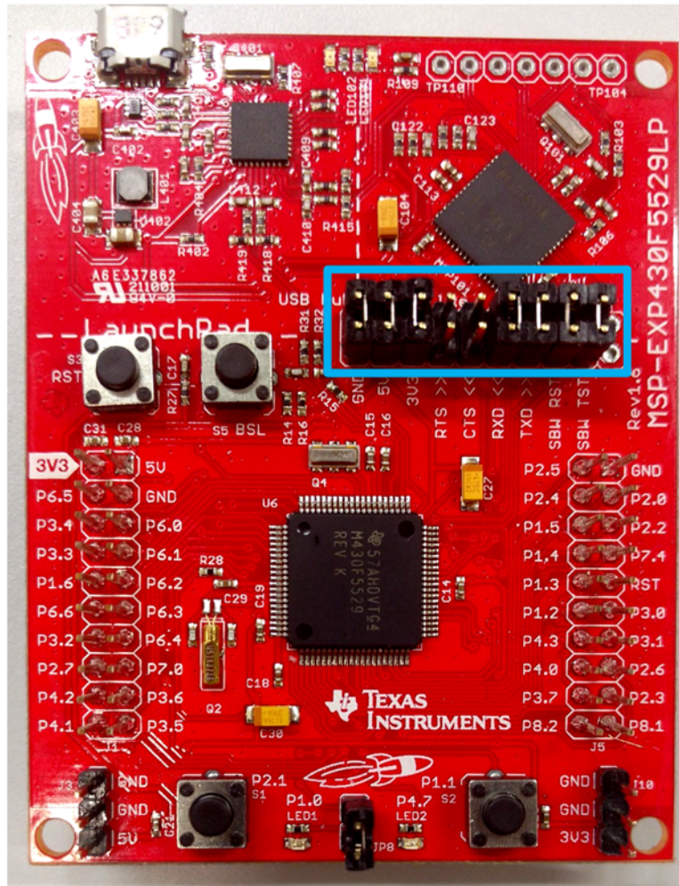
图 5. MSP430™ LaunchPad™ Jumpers to Remove
