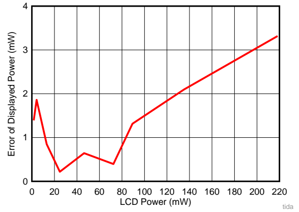
图 22. LCD Power Accuracy
