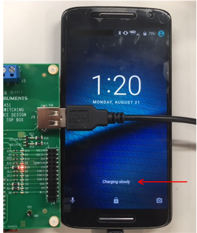
图 11. Phone Charging on Connector
