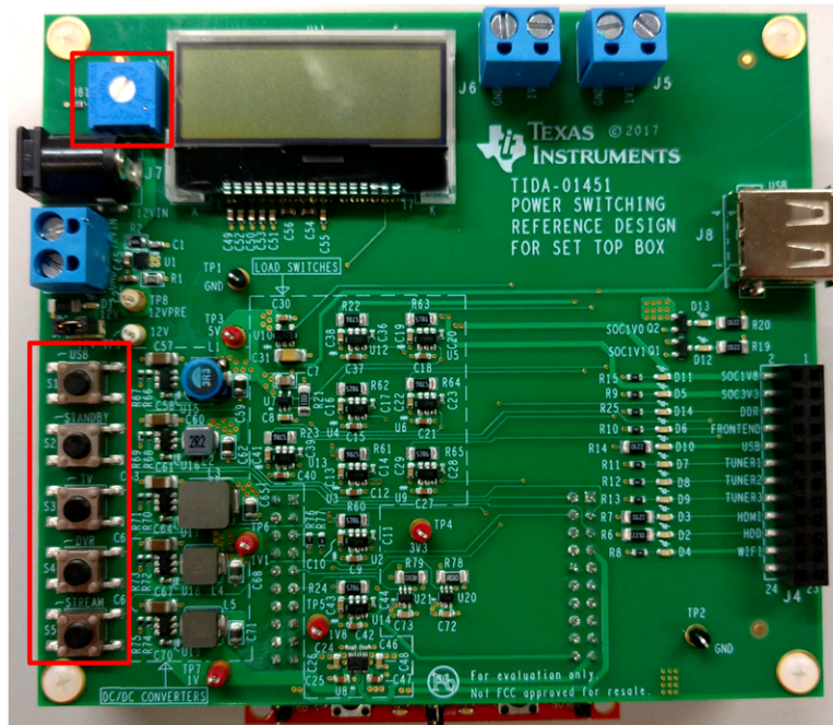
图 7. Board Image With Buttons and Potentiometer Highlighted
