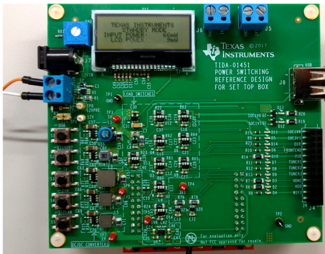
图 8. Full Board 12 V IN With LCD ON
