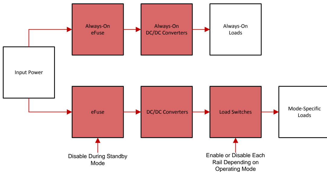
图 4. Separate Always-On Power Tree for Additional Power Savings
