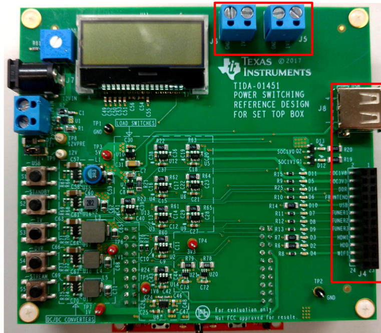
图 19. Board Image With Outputs Highlighted
