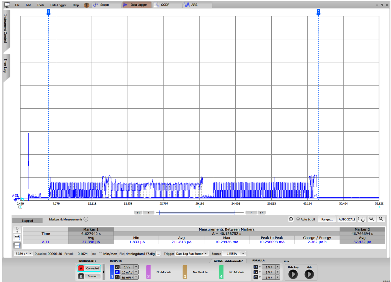
图 28. CC2640R2F Current Consumption During Provisioning
