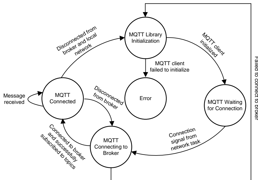
图 8. MQTT Thread Main Loop
