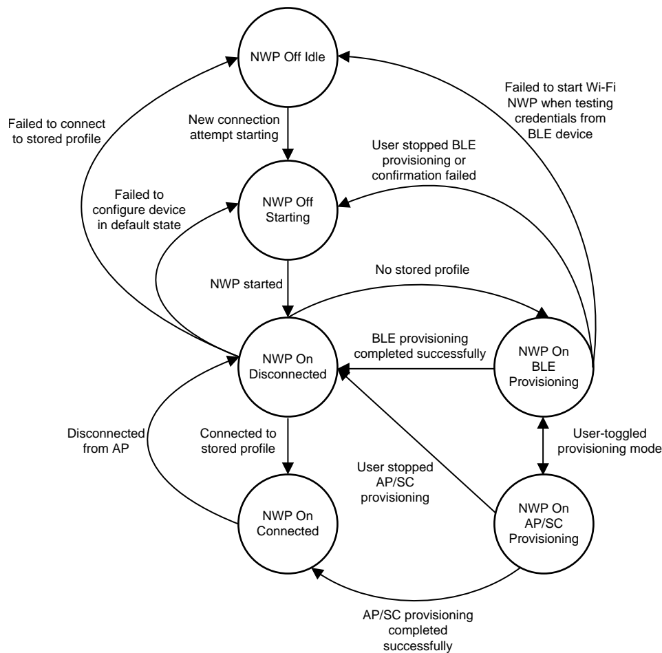
图 5. Network-Connection Management-Thread Flow Diagram
