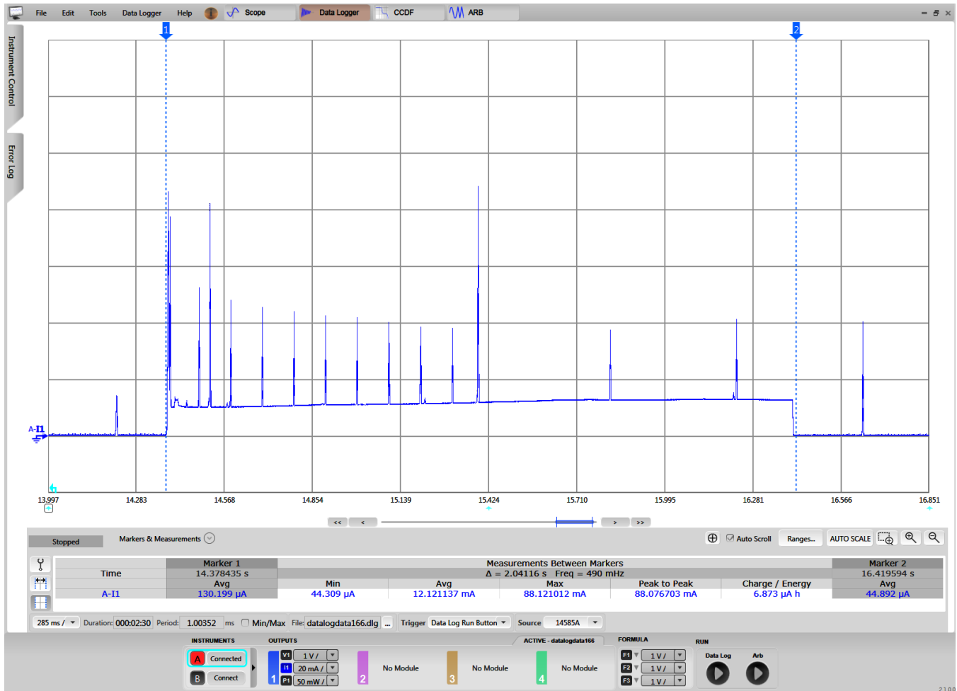
图 26. CC3220 Current Consumption During Lock and Unlock Cycle
