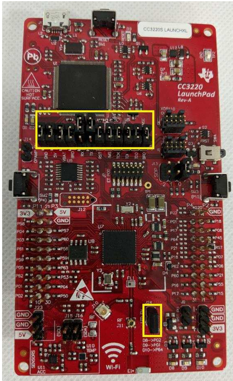
图 11. CC3220S-LAUNCHXL Jumper Configuration
