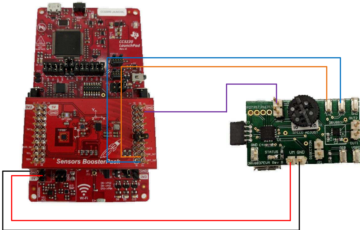
图 16. Jumper Wire Placement to Connect DRV8837EVM to System
