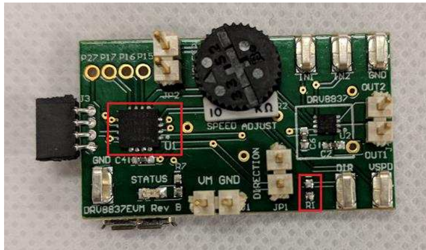
图 24. Front of DRV8837EVM With Highlighted Components To Remove
