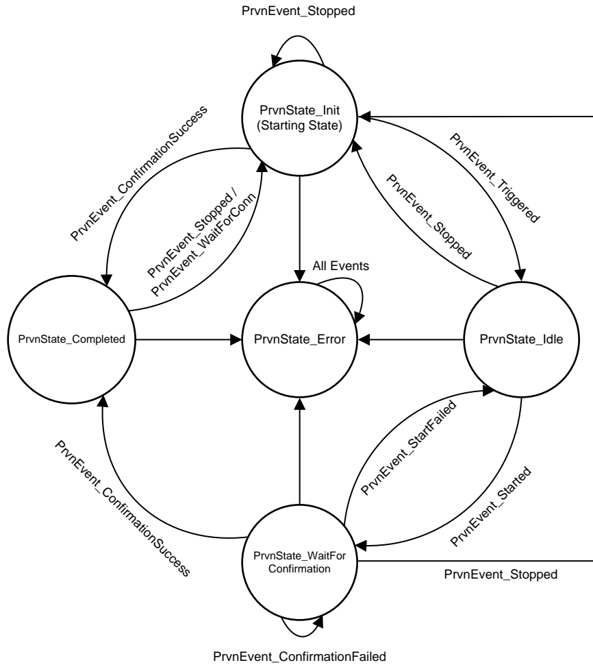
图 6. Provisioning Task State Machine
