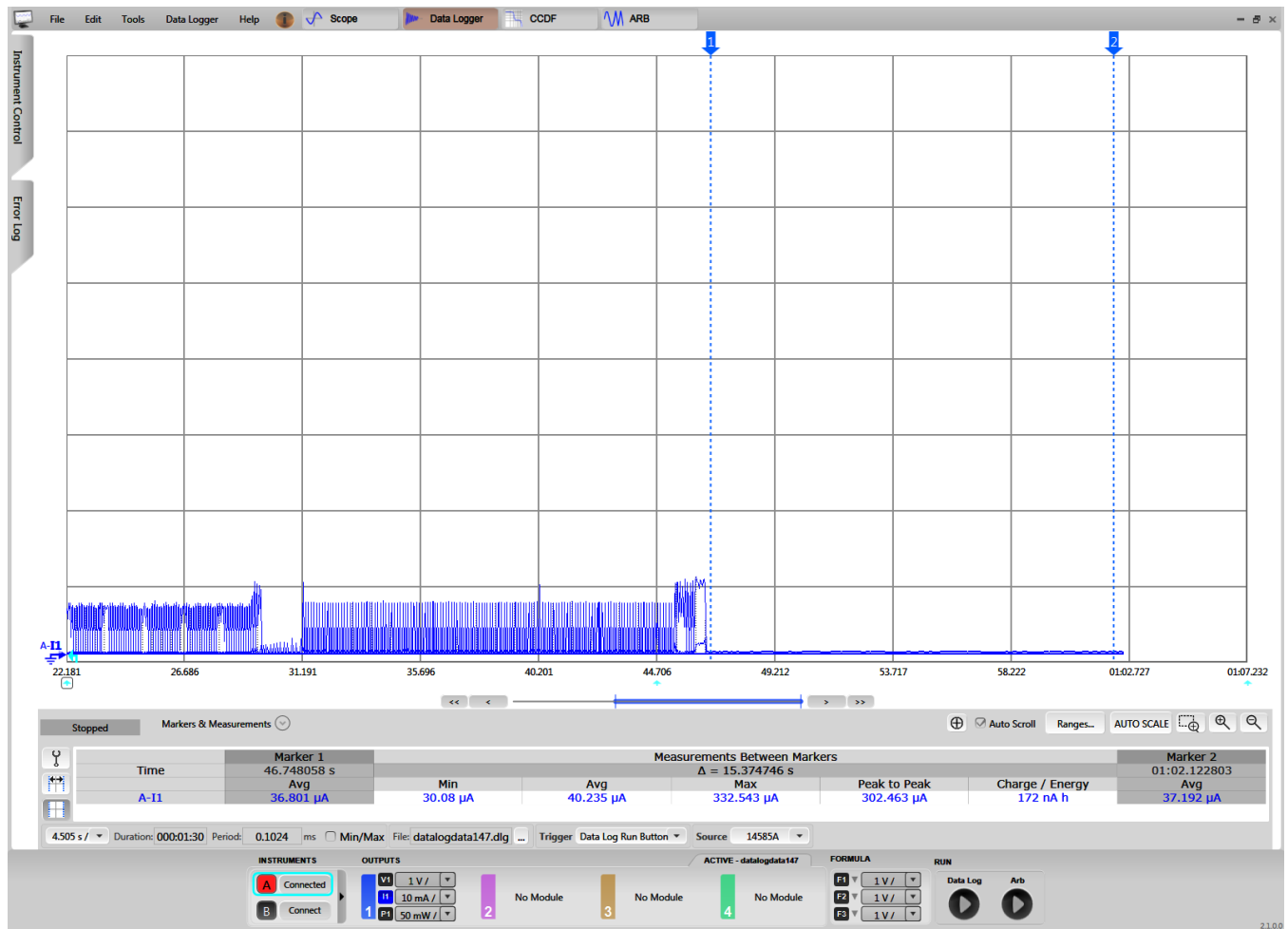
图 29. CC2640R2F Current Consumption While Idle
