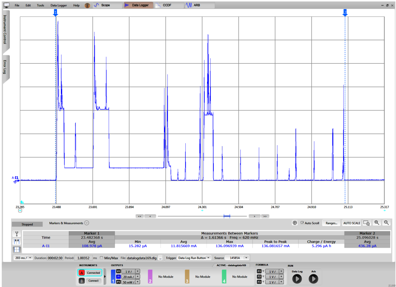
图 27. CC3220 Current Consumption During Lock Status Request
