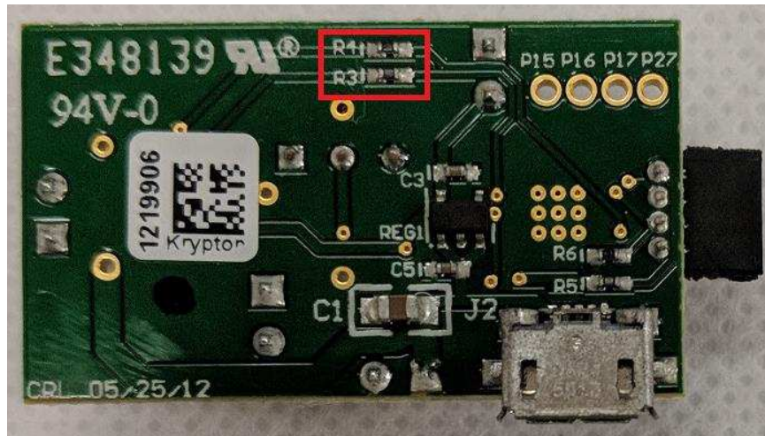
图 13. R3 and R4 Location on Back of DRV8837EVM
