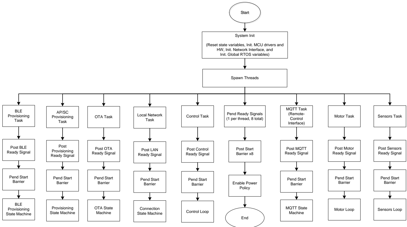
图 4. Overall Software Flow Diagram
