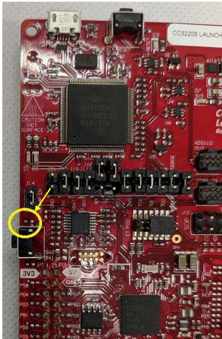
图 22. R141 Location on CC3220S LaunchPad™
