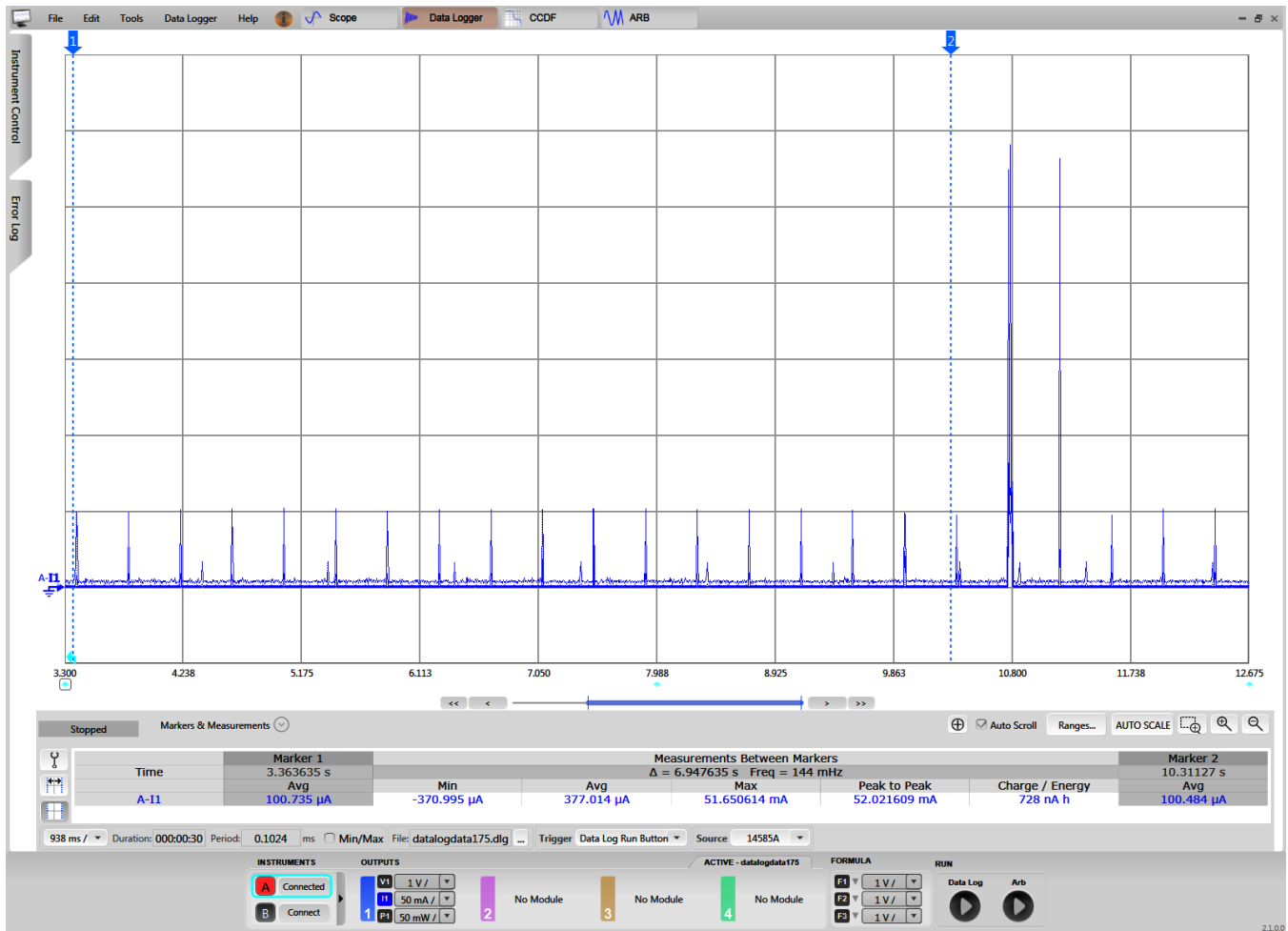
图 25. CC3220S Current Consumption Versus Time While in Idle Connected Mode With 400-ms LSI
