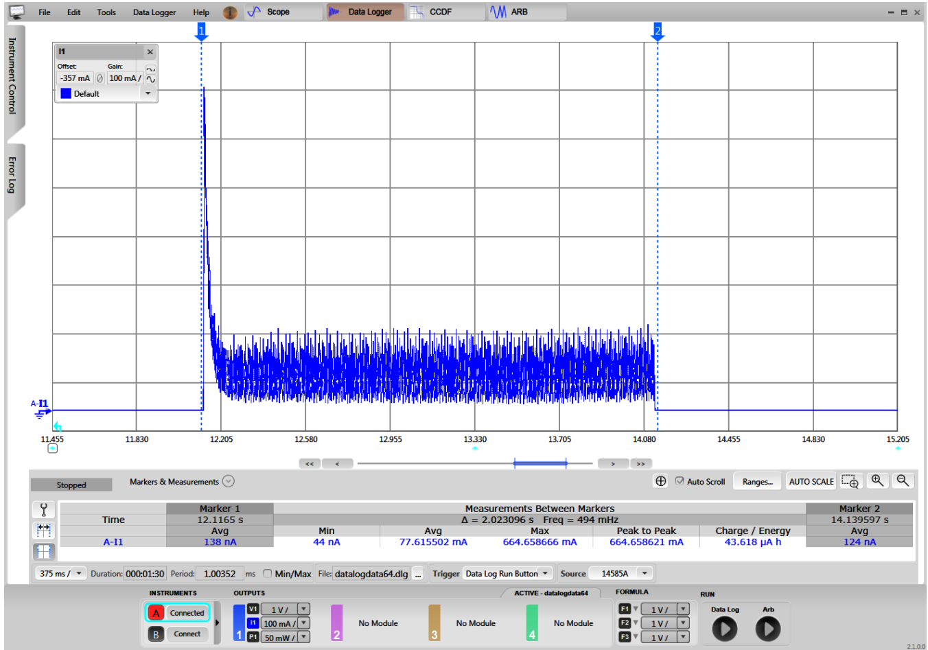
图 30. DRV8837 Current During Lock Event
