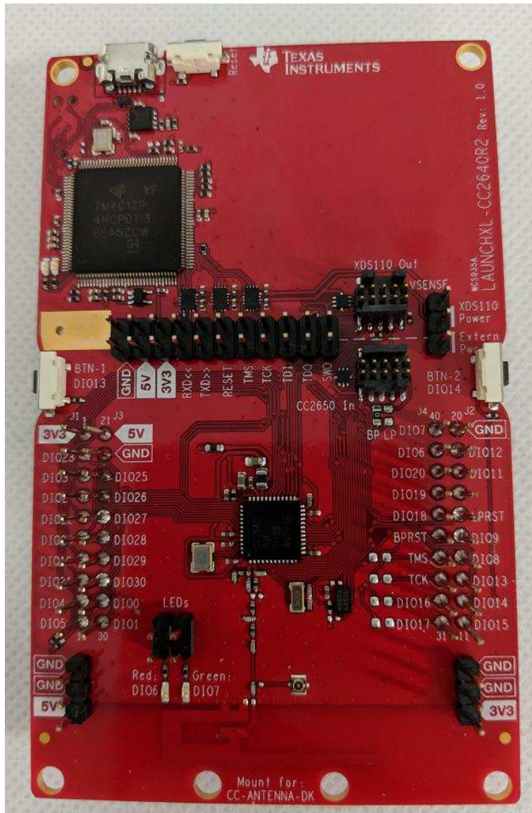
图 12. CC2640R2F LaunchPad™ Configuration
