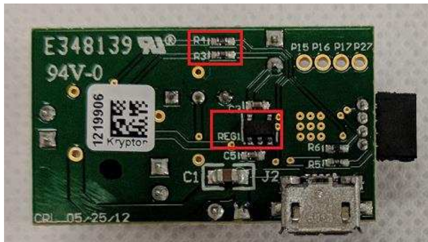
图 23. Back of DRV8837EVM With Components To Remove Highlighted
