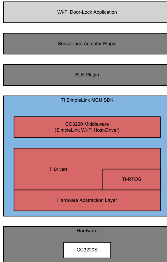
图 3. Wi-Fi, Door-Lock Software Block Diagram
