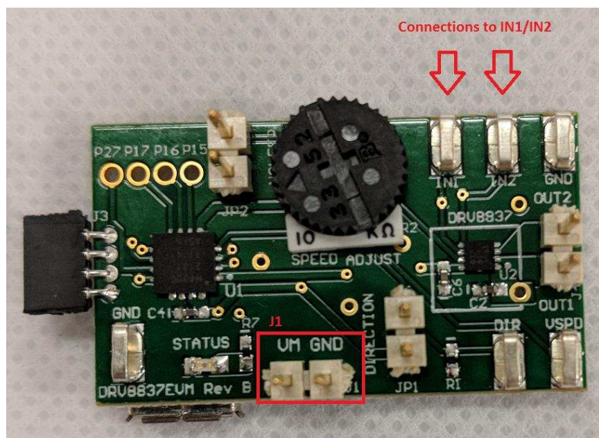
图 14. J1 and IN1/IN2 Highlighted on Front of DRV8837EVM
