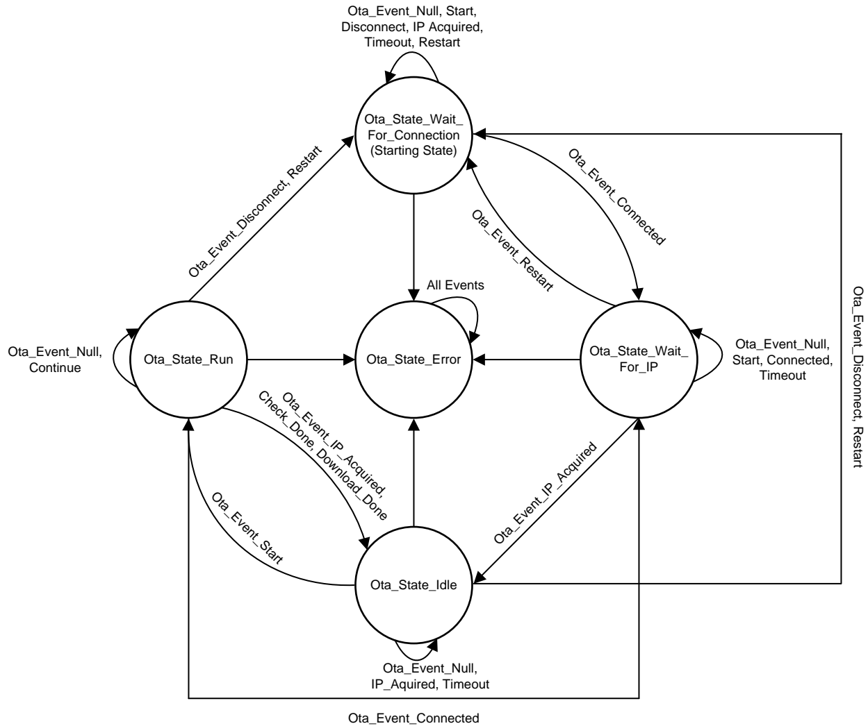
图 10. OTA Task State Machine
