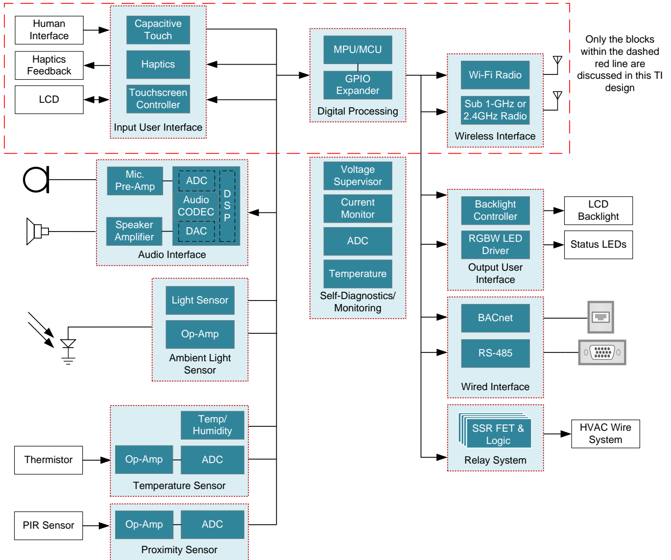
图 2. Smart Thermostat HMI Block Diagram
