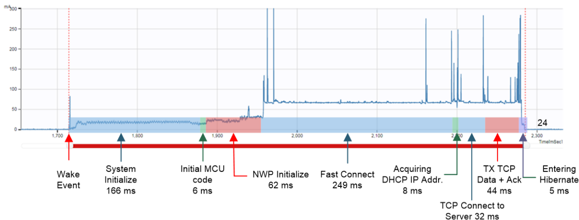
图 14. Current Consumption vs Timing in Intermittently-Connected Mode
