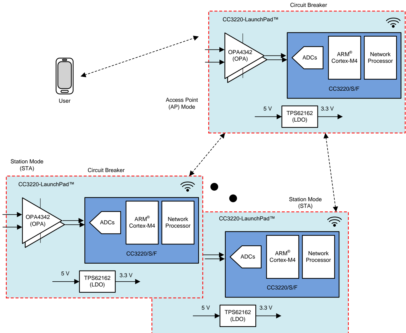
图 6. SimpleLink™ AP Architecture
