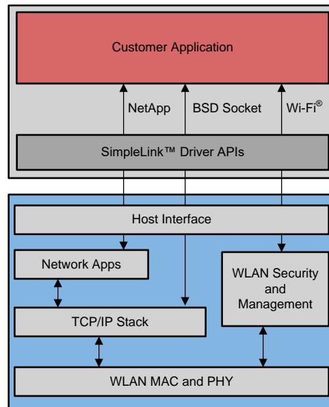
图 4. CC3200x Embedded Software Overview
