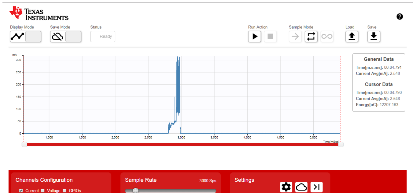
图 12. Power Profile in Intermittently-Connected Mode (5-s Interval)
