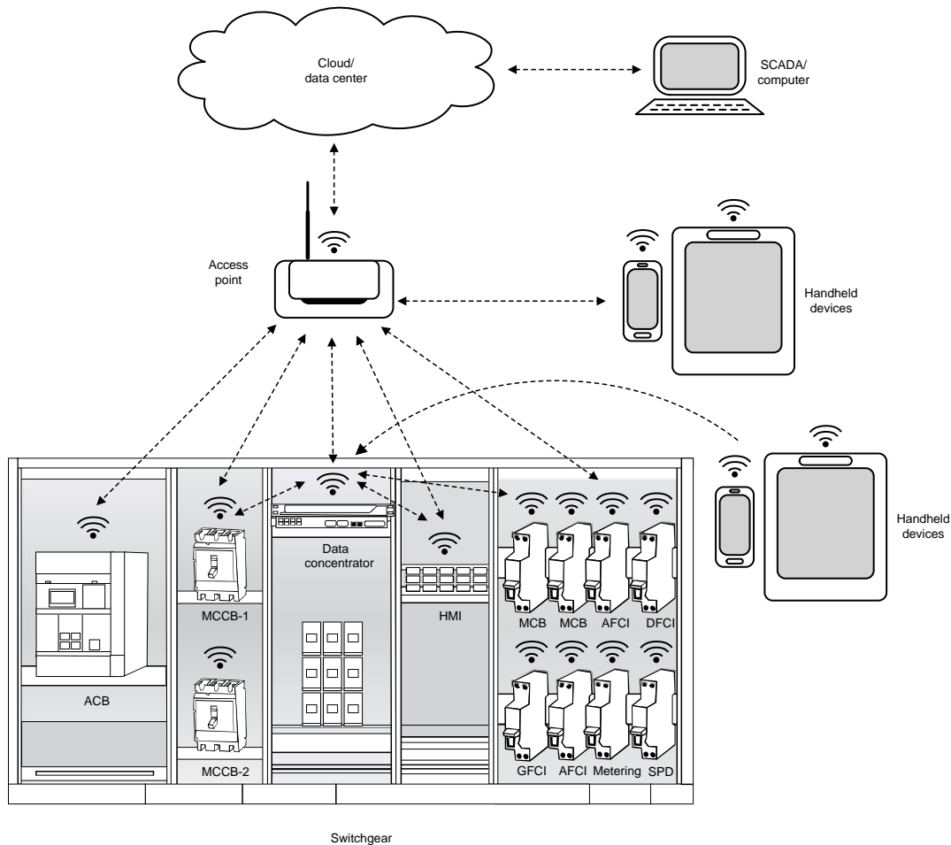
图 1. Connected Circuit Breakers
