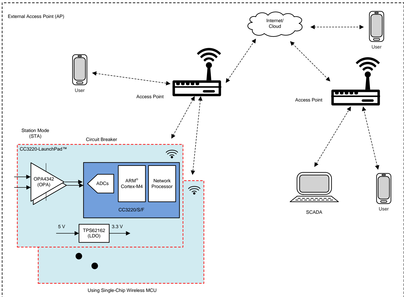
图 5. Wi-Fi® Connectivity Through External Access Point
