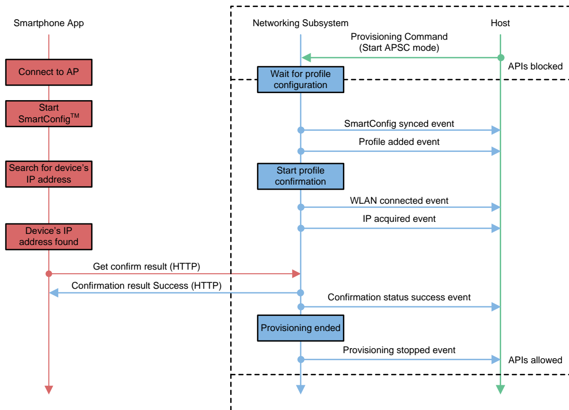
图 7. Timing Diagram for Successful SmartConfig™ Provisioning
