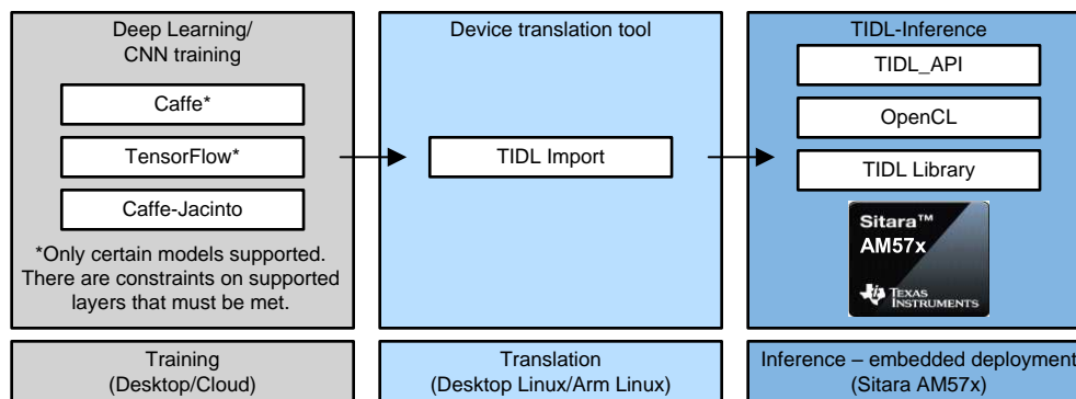
图 6. TIDL Development Flow
