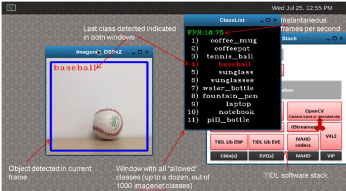
图 14. Additional Objects Detected
