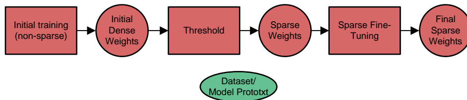
图 7. Caffe Jacinto-Based Sparse Training
