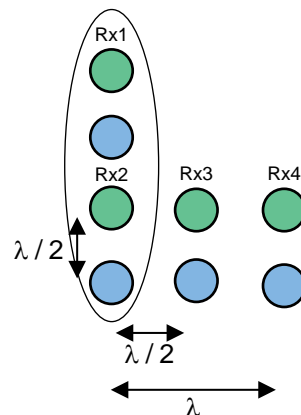
图 5. Virtual Antenna Array for Range-Elevation-Angle Heat-Map Calculation
