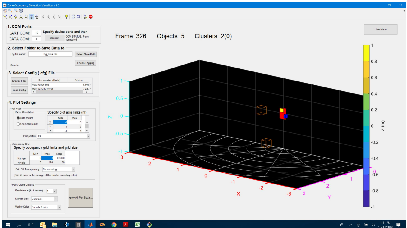
图 11. Horizontal Concrete Block and Plastic Reflector - 3D View
