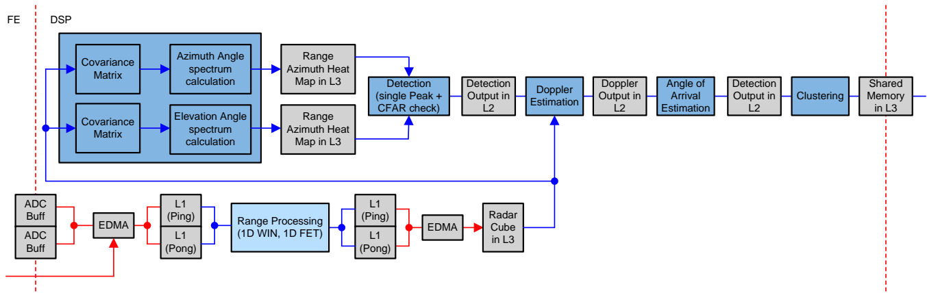
图 4. System Process Chain
