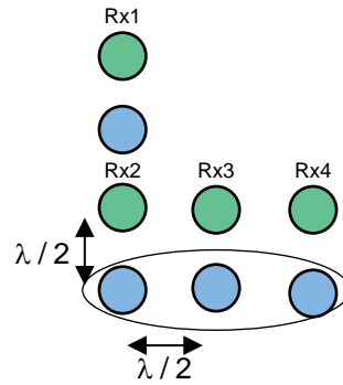
图 6. Virtual Antenna Array for Range-Azimuth-Angle Heat-Map Calculation
