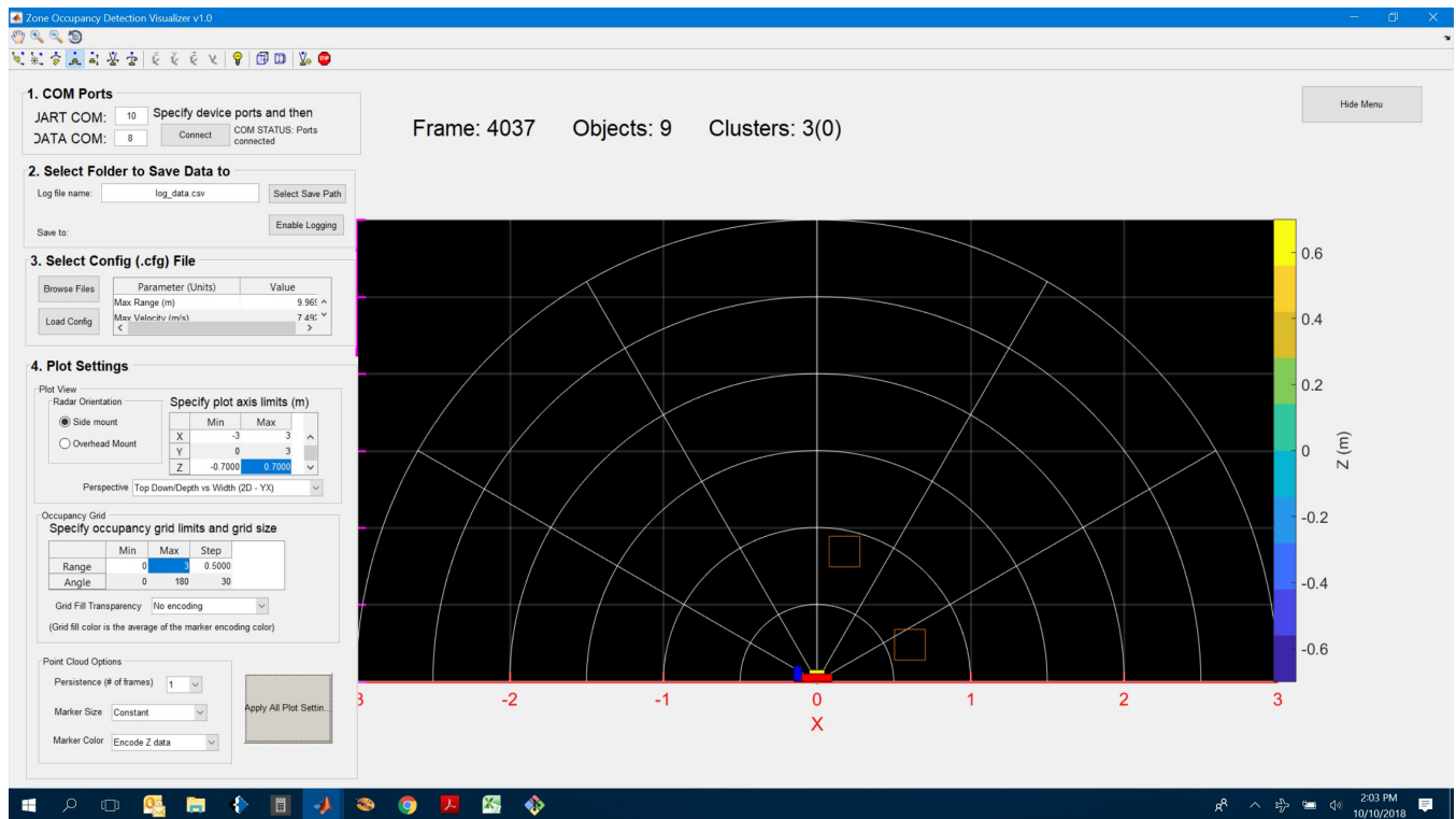
图 10. Horizontal Concrete Block and Plastic Reflector - 2D View
