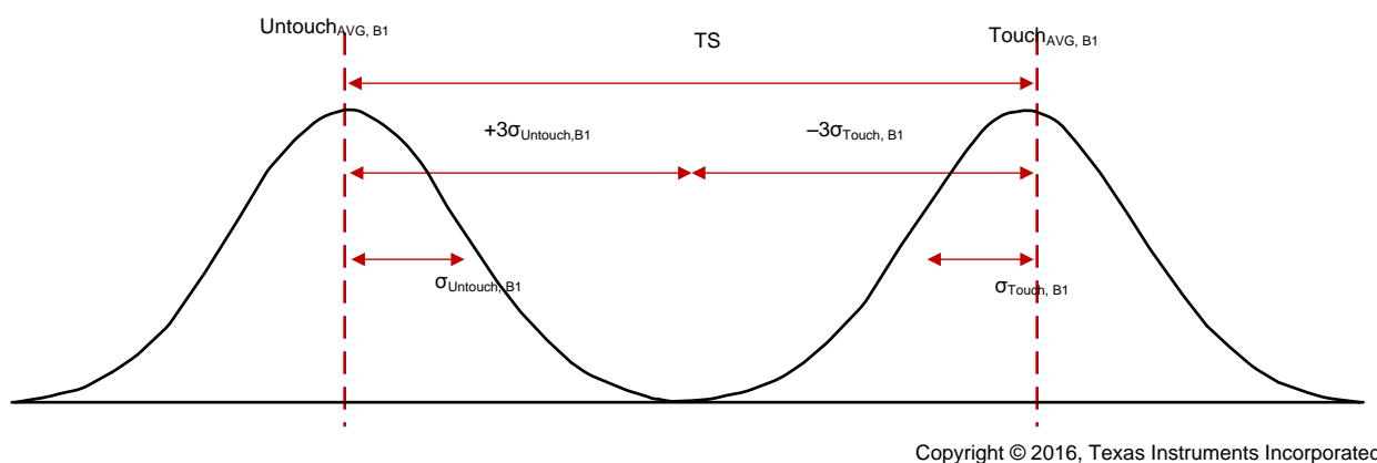
图 16. Event Distribution (SNR) With and Without Touch
