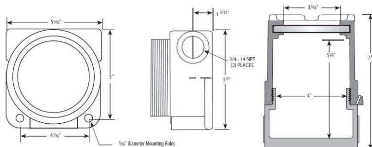
图 3. Explosion-Proof Enclosure
