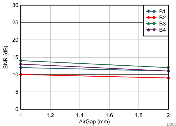
图 22. Finger Touch With Gloves—SNR
