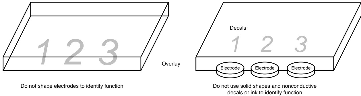
图 11. Button Shape Examples, Dos and Don'ts
