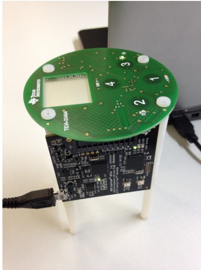
图 14. TIDA-00494 Connected to the PC, Ready for Data Acquisition and Debugging
