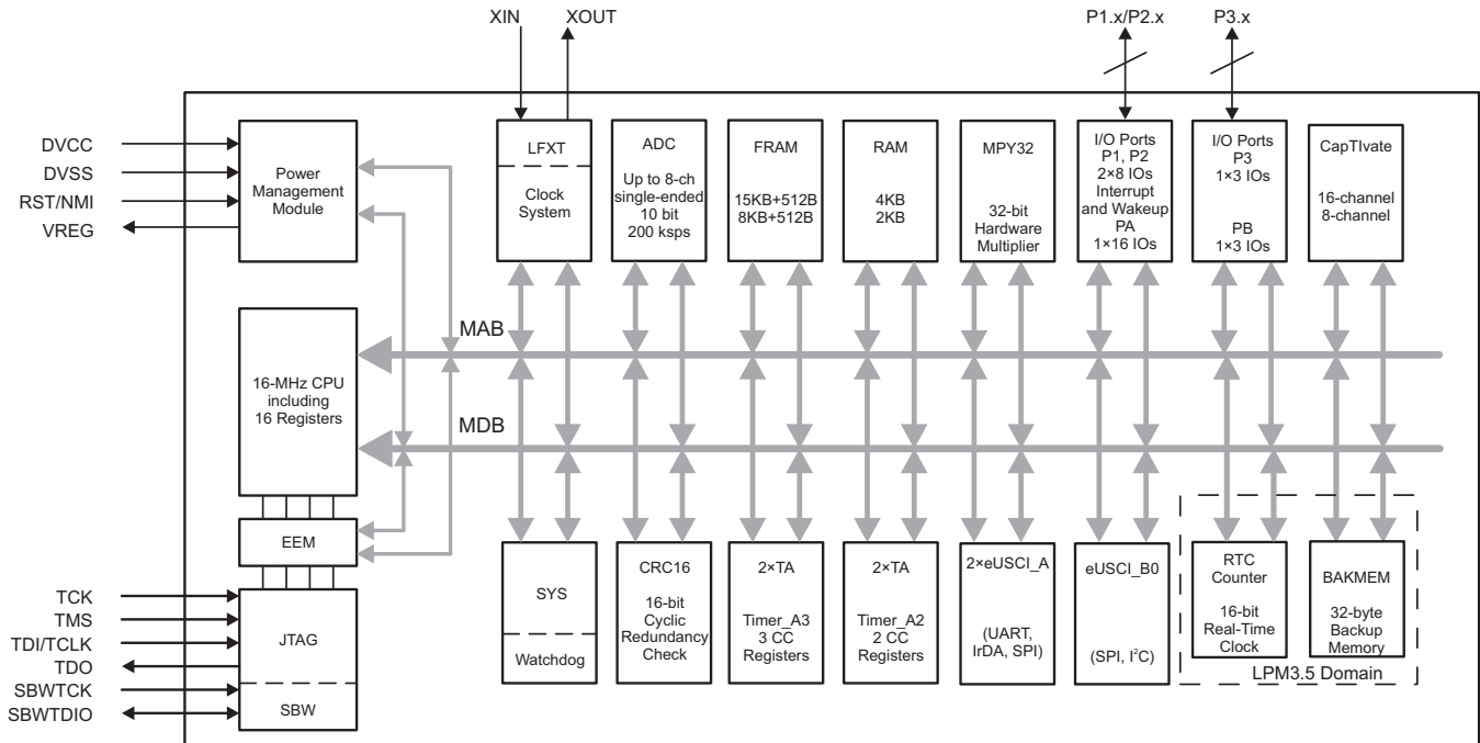
图 2. MSP430FR2633 Functional Block Diagram
