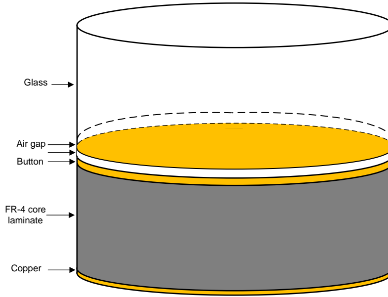
图 5. Application Stackup
