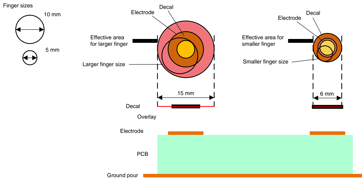
图 10. Effective Area Example for Electrode Smaller Than Decal
