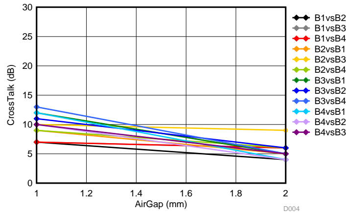
图 23. Finger Touch With Gloves—Crosstalk
