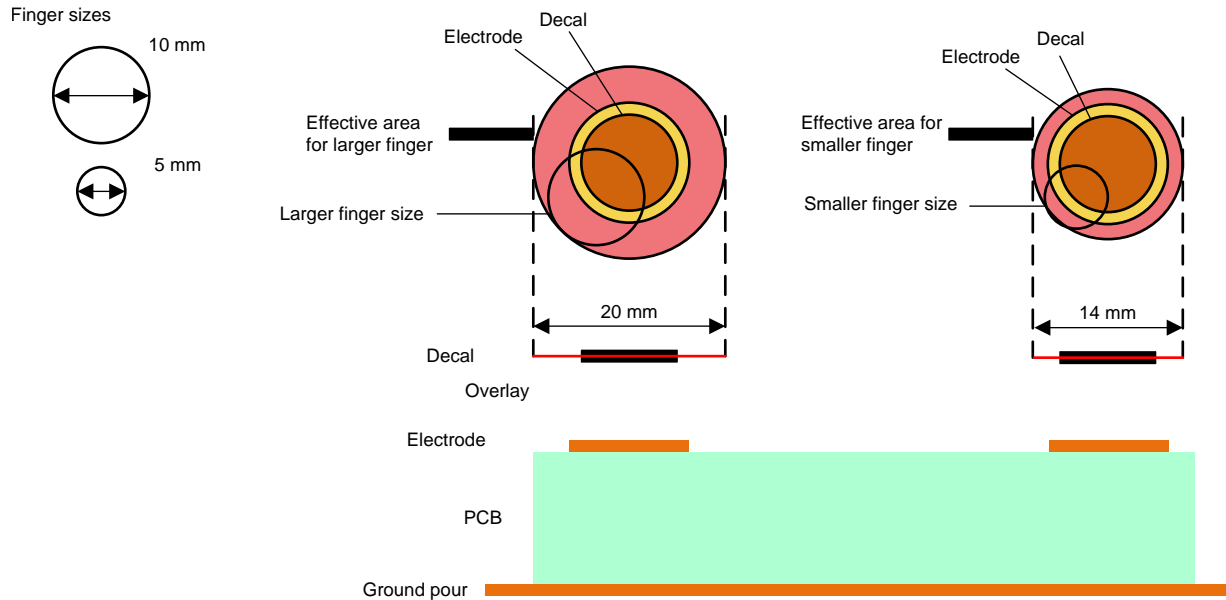
图 9. Effective Area Example for Electrodes Larger Than Decal
