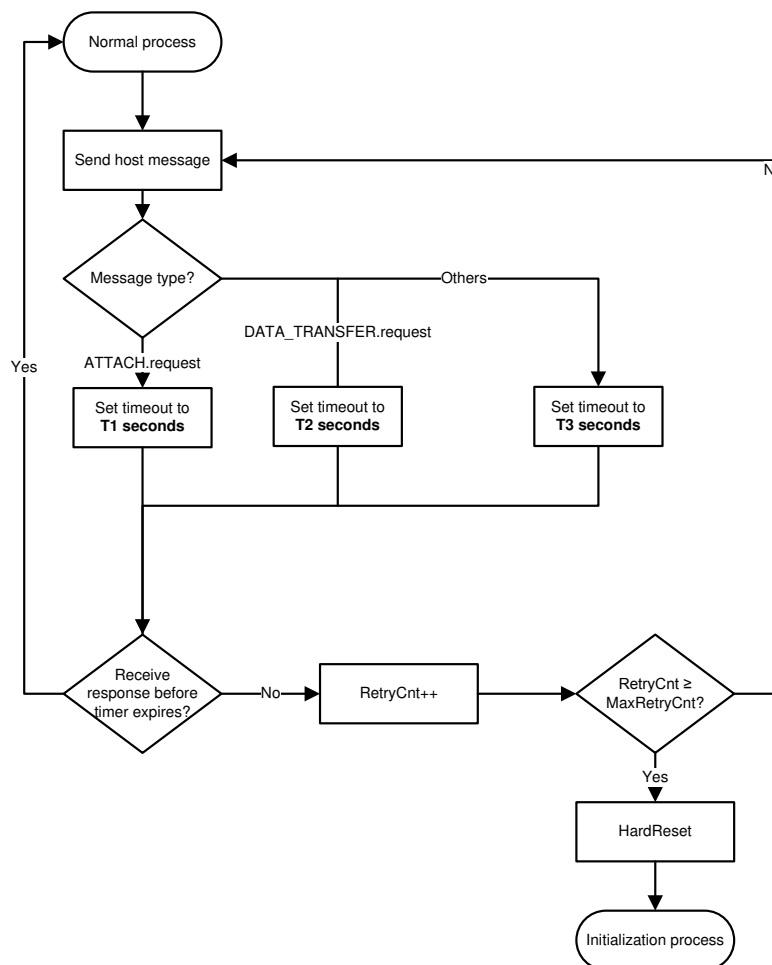
图 16. Recovery and Timeout Mechanism
