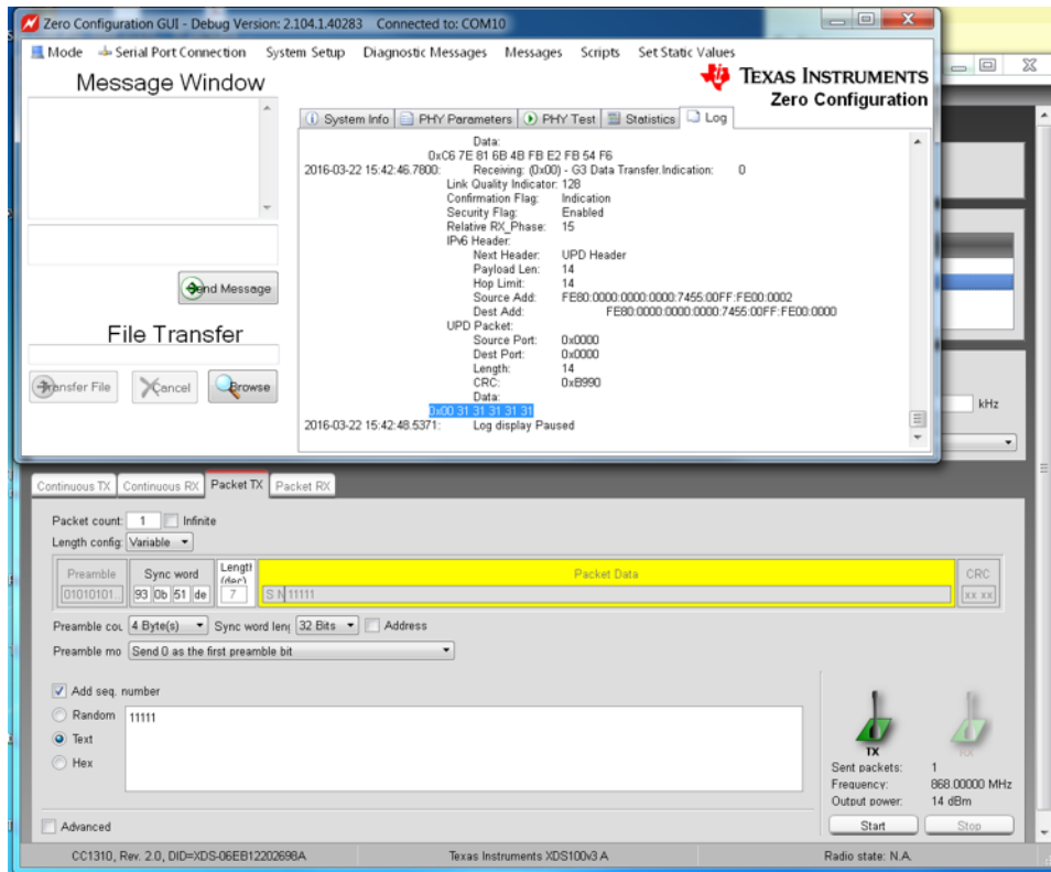
图 29. RF-to-PLC Repeater
