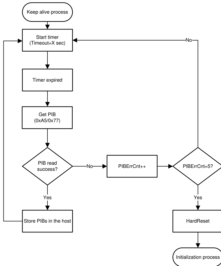
图 15. Keep-Alive Mechanism
