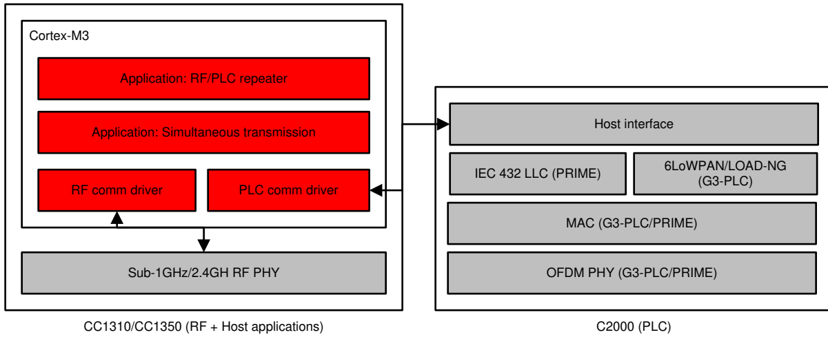
图 1. System Architecture (RF With PLC Full-Stack)
