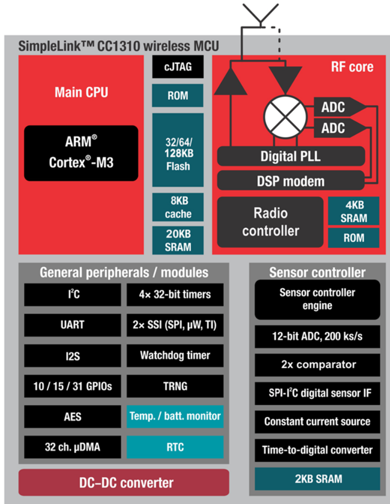
图 4. CC1310 Functional Block Diagram[1]
