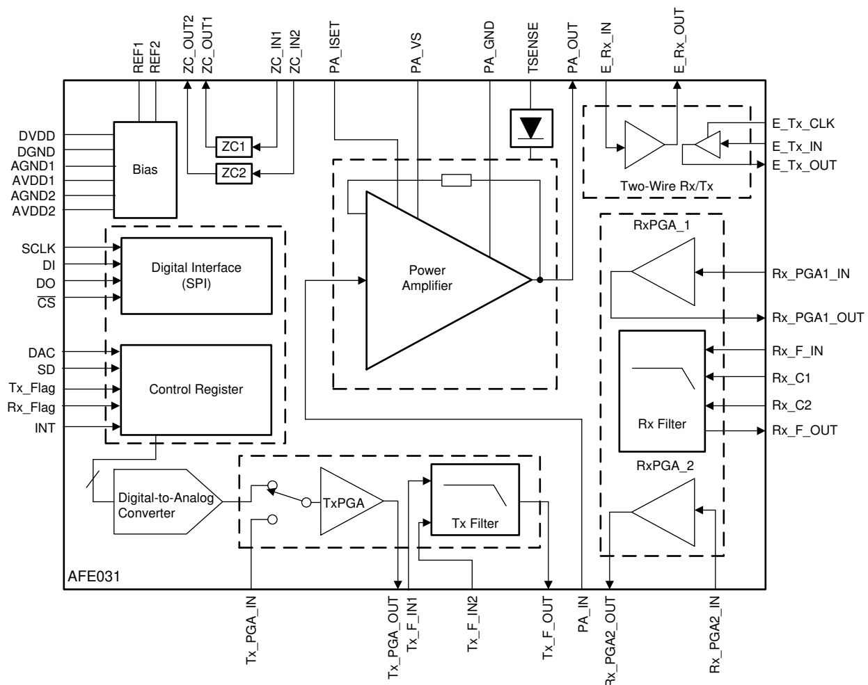
图 6. AFE031 Functional Block Diagram[3]
