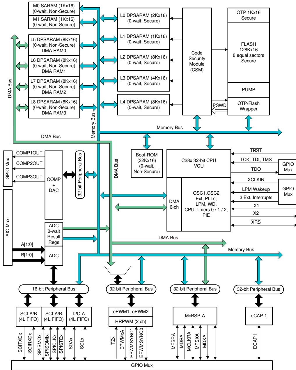
图 5. TMS320F28PLC84 Functional Block Diagram[2]
