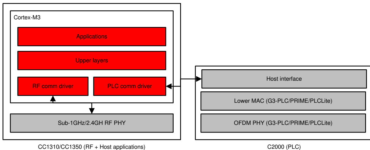
图 2. System Architecture (RF With PLC Lower-MAC Stack)
