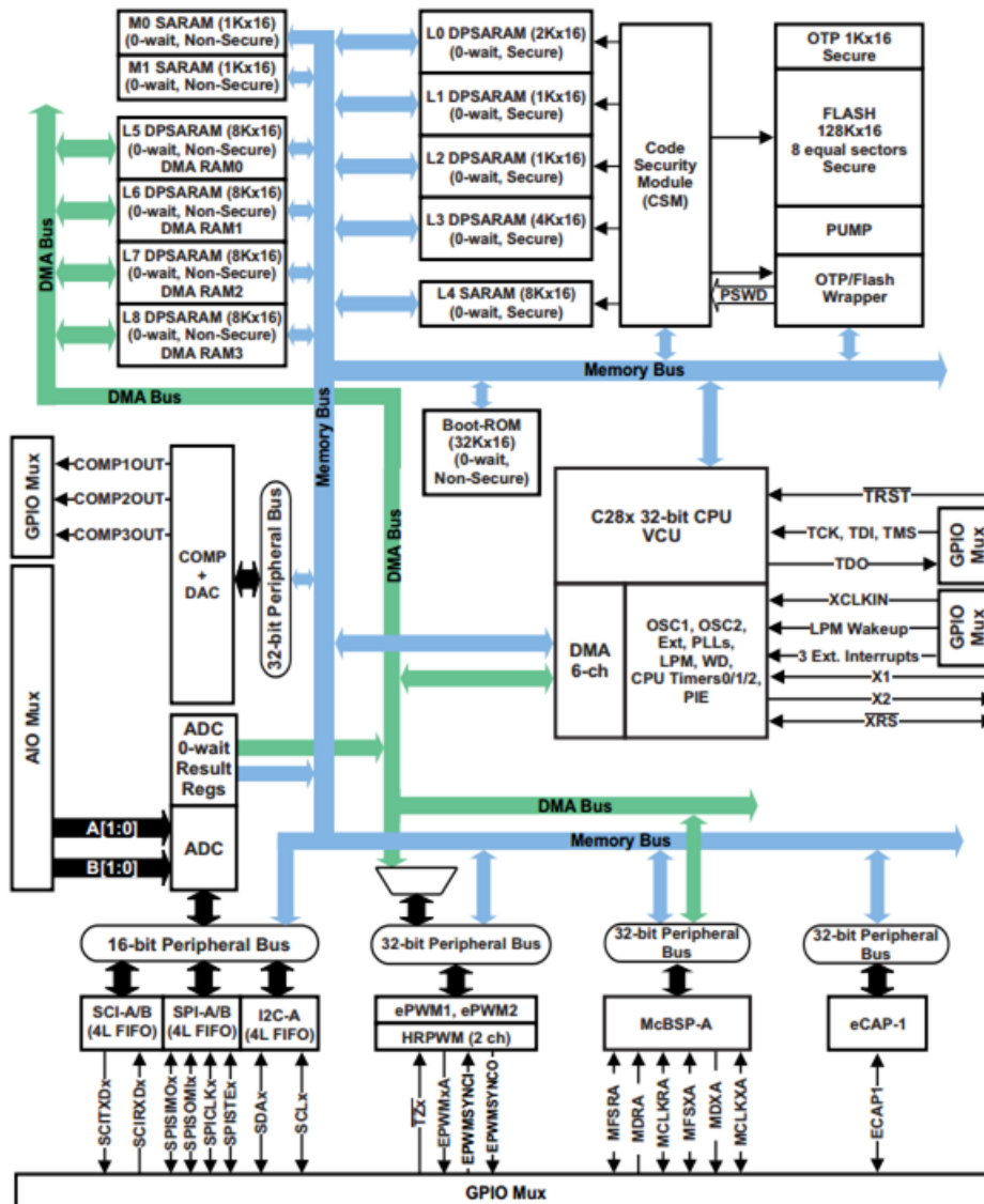
图 4. TMS320F28PLC Functional Block Diagram
