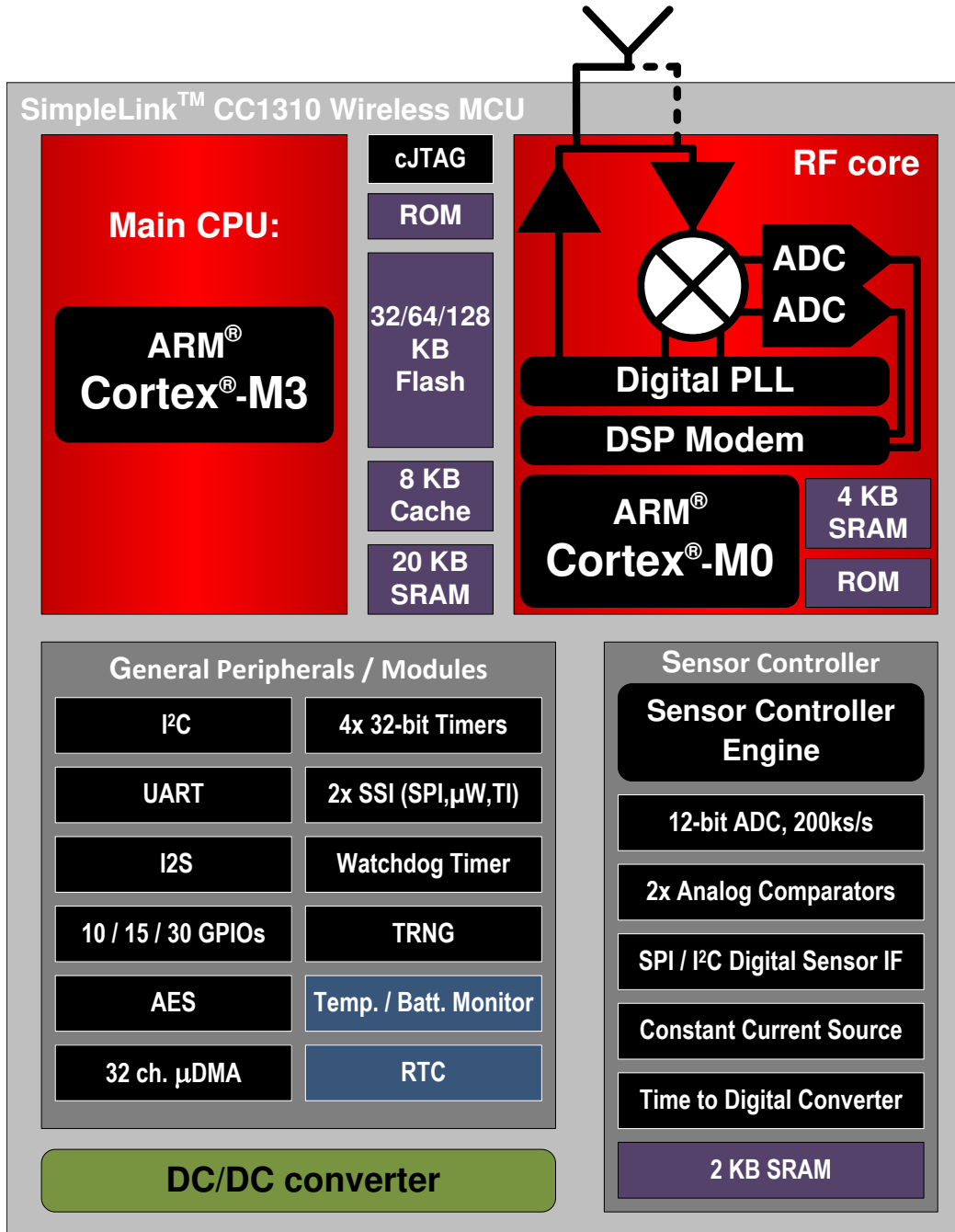
图 3. CC1310 Functional Block Diagram
