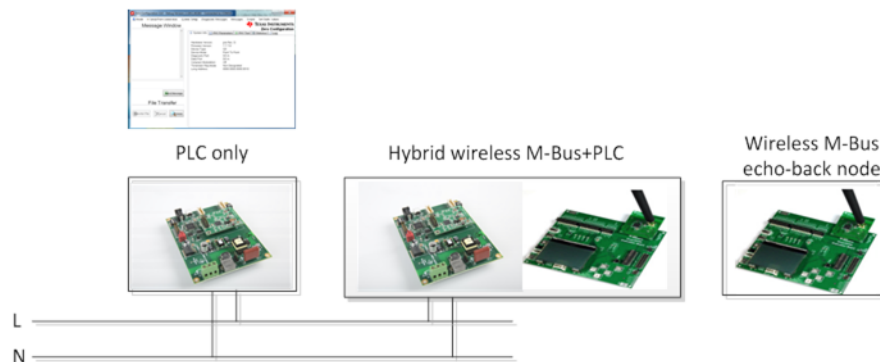
图 15. Hybrid Wireless M-Bus/PLC Test Setup
