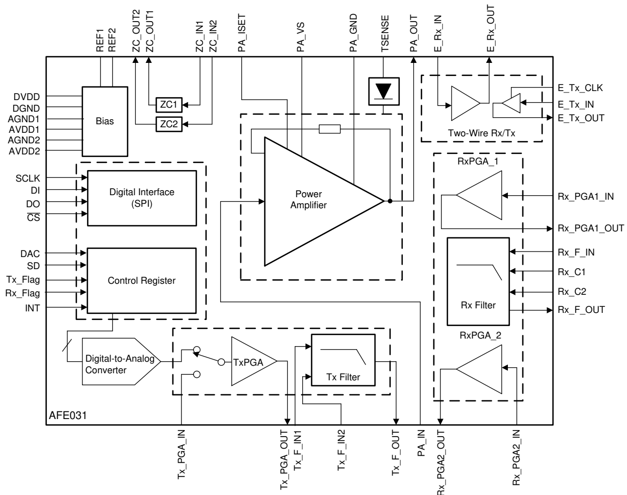
图 5. AFE031 Functional Block Diagram
