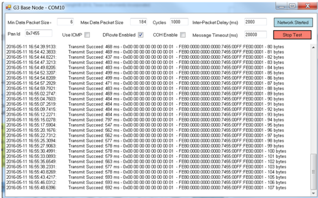
图 23. Hybrid Wireless M-Bus and PLC Echo-Back Test Result
