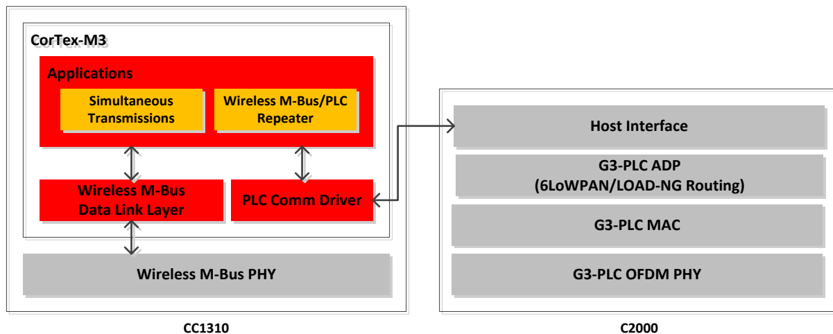
图 1. System Architecture (Wireless M-Bus With PLC)
