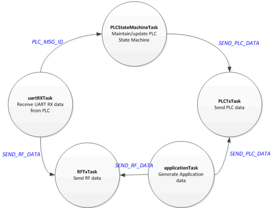
图 13. Hybrid WMBUS/PLC Example Software Architecture
