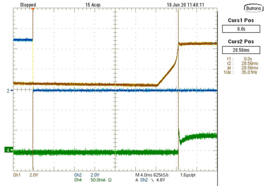
图 3-12. Daytime Running Light Turn-on Delay
