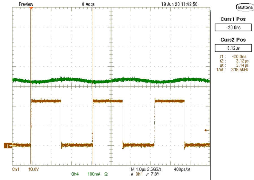
图 3-13. Daytime Running Light Switch Node and Output Current
