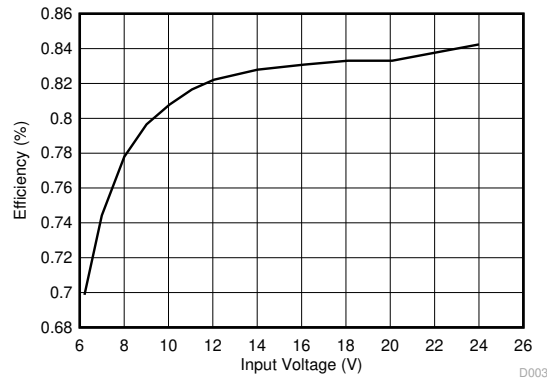
图 3-20. Efficiency Turn Indicator and Daytime Running Light
