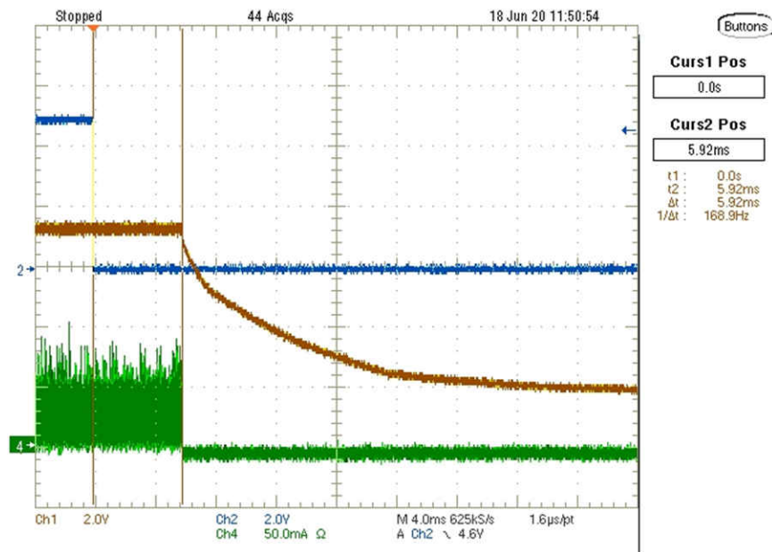
图 3-9. Turn Indicator Turn Off Delay
