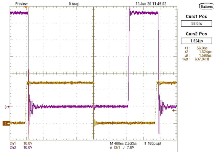
图 3-17. TPS92682-Q1 Boost and SEPIC Interleaving
