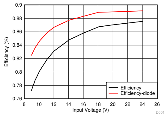
图 3-18. TIDA-050040 Full Load Efficiency
