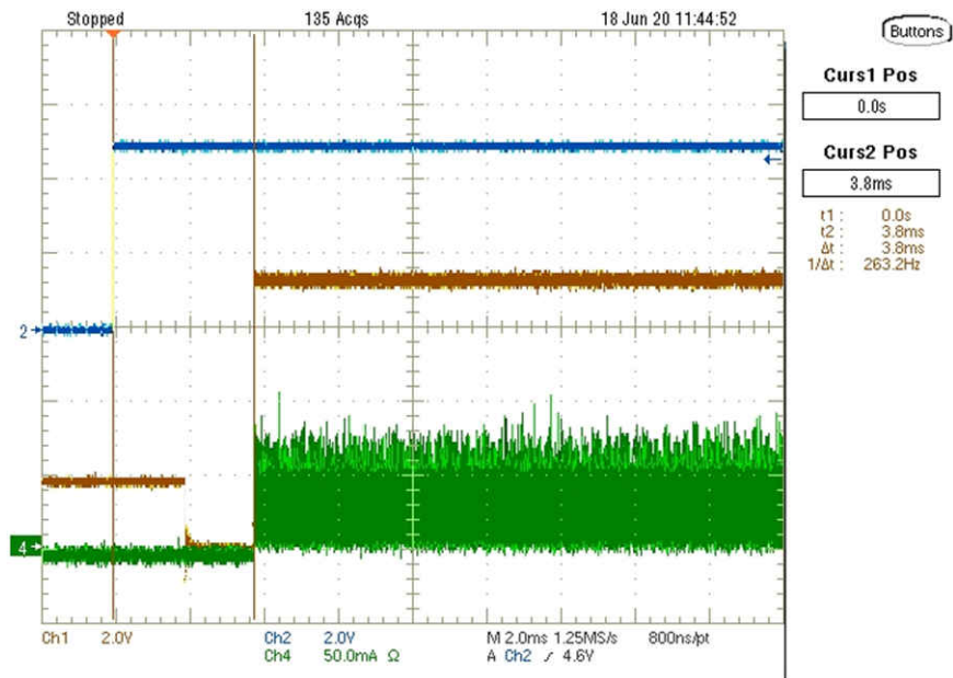
图 3-8. Turn Indicator Turn on Delay
