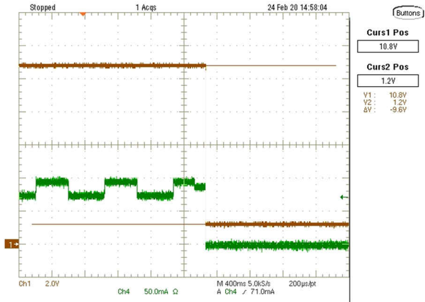
图 3-15. Highbeam/Lowbeam Fault Indicator
