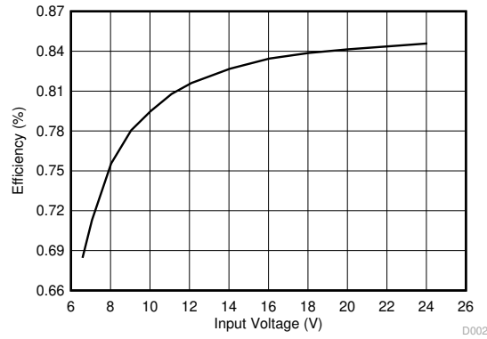
图 3-19. Efficiency Highbeam/Lowbeam
