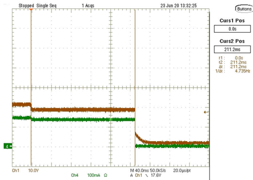
图 3-14. Highbeam/Lowbeam LED Short
