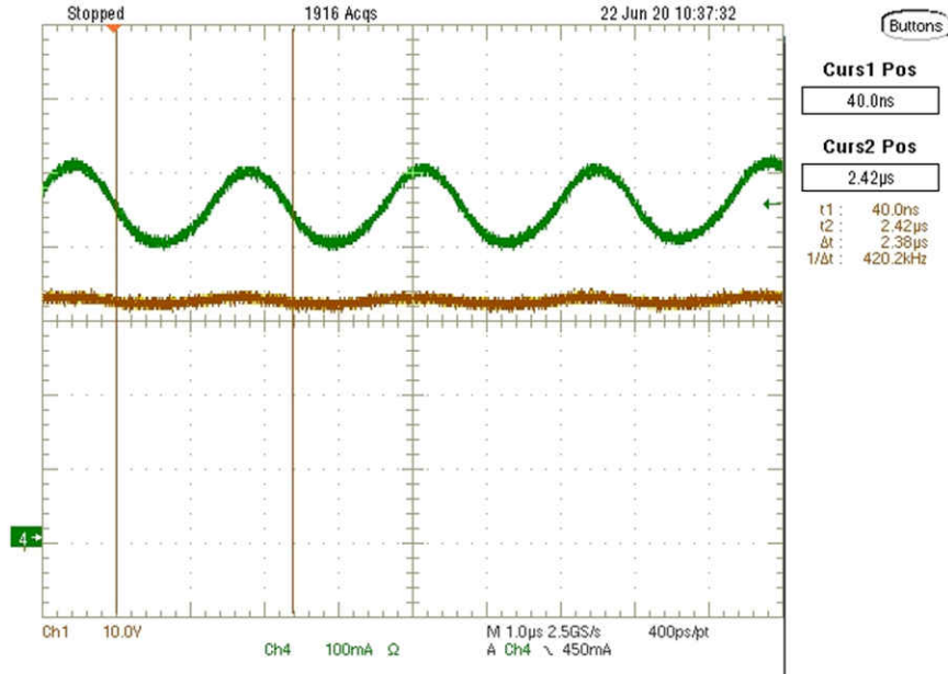
图 3-11. Turn Indicator Output Voltage and Current
