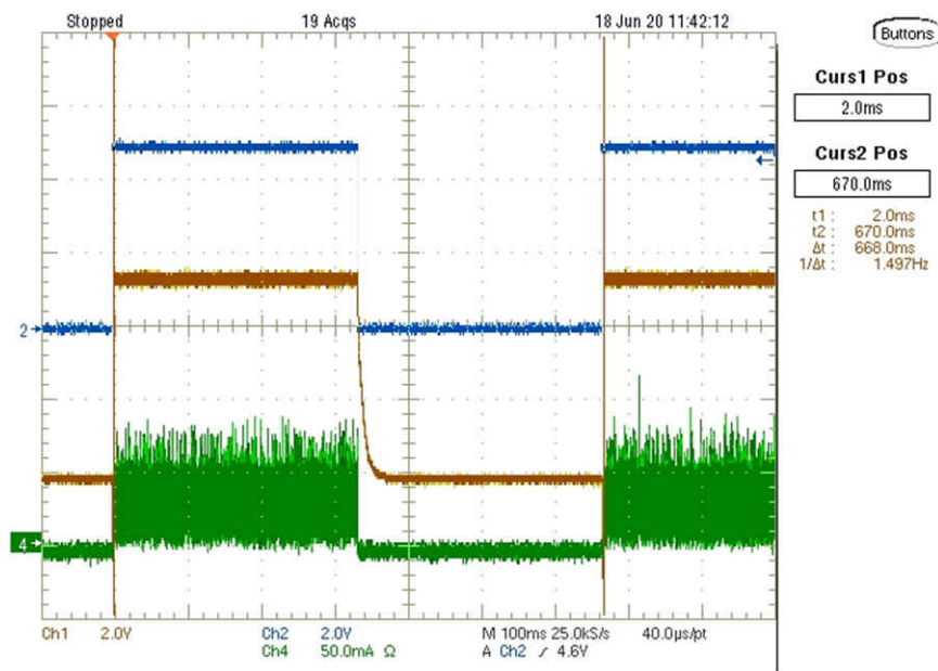
图 3-10. Turn Indicator 1.5 Hz Operation
