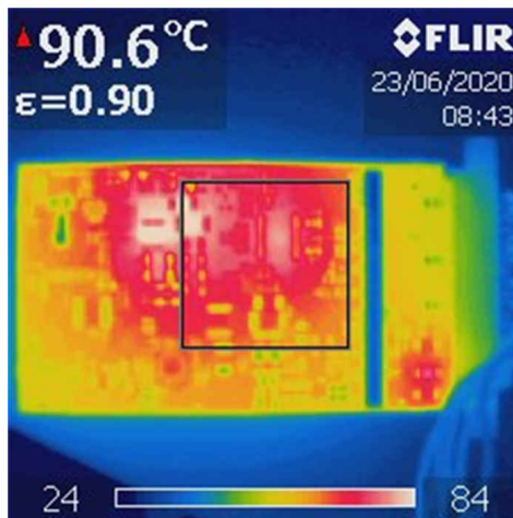
图 3-25. Top Side Thermal Image Highbeam/Lowbeam at 30W, Turn Indicator at 7.5W average
