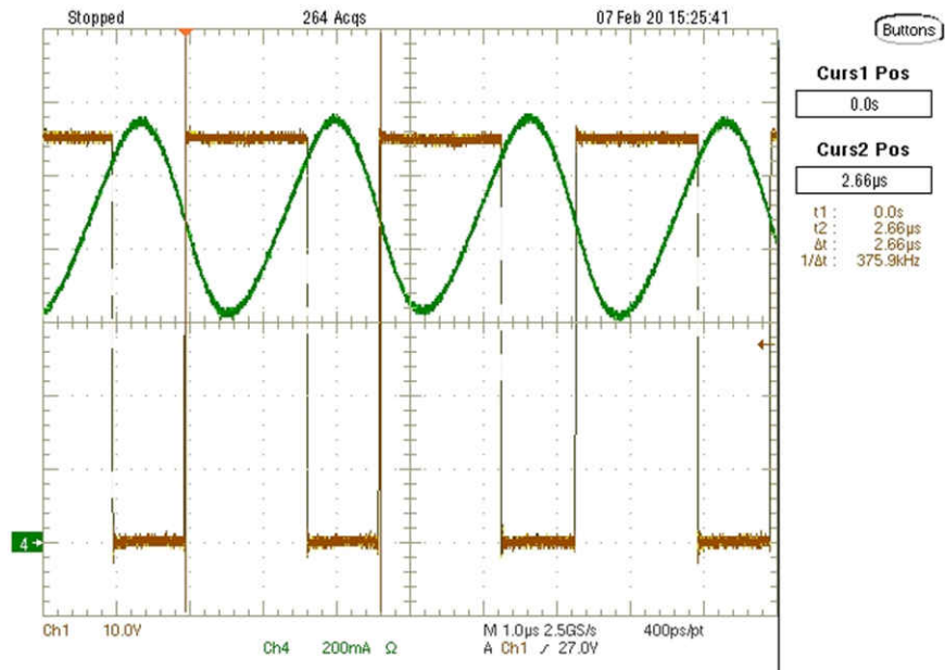
图 3-7. Highbeam/Lowbeam Switch Node and Ripple Current
