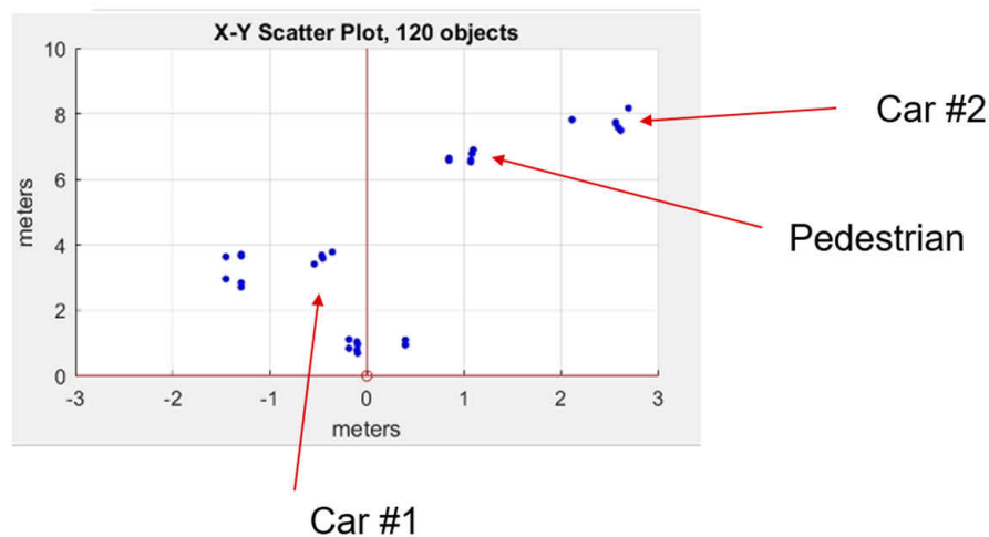
图 3-5. Detection Point Cloud of Pedestrian Standing in Empty Parking Space
