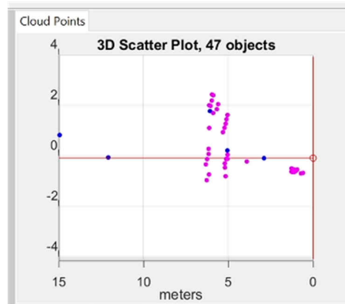
图 3-3. Detection Point Cloud of Traffic Sign Pole – Elevation View
