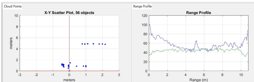
图 3-10. Detection Point Cloud of Parking Block
