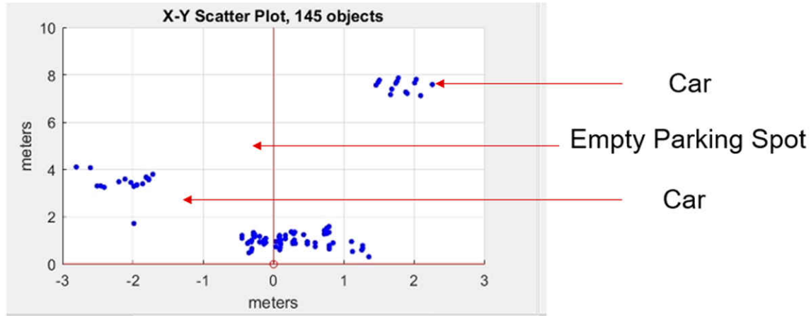
图 3-8. Detection Point Cloud of Empty Parking Space
