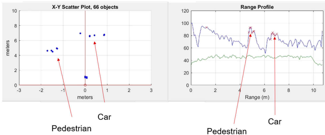
图 3-7. Point Cloud for Static Detection
