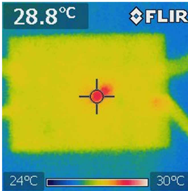
图 5-12. 热性能，强制 PWM ( V_{IN} = 12V , V_{OUT} = 3.3V , I_{OUT} = 300mA , F_{SW} = 2.5MHz )
