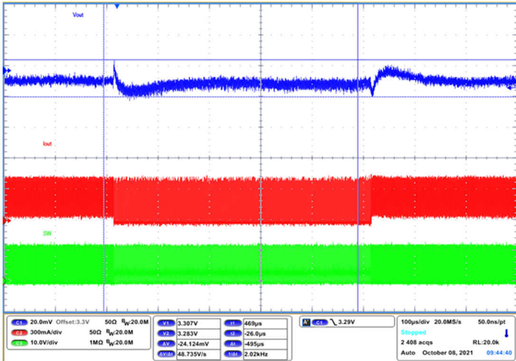
图 5-11. 负载瞬态，强制 PWM VSET ( V_{IN} = 12V , V_{OUT} = 3.3V , I_{OUT} = 100mA - 300mA , 压摆率 = 1A/\mu s )
