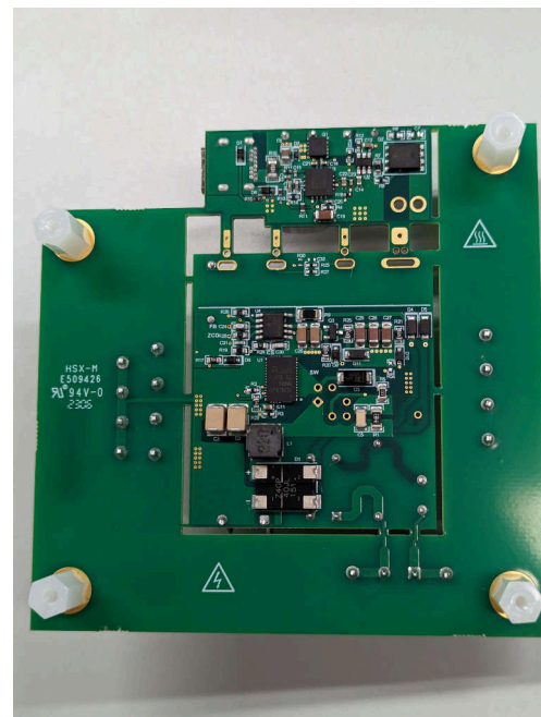
LMG3624EVM-081 (底视图)
