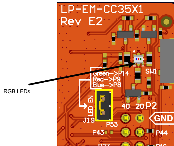
图 2-17. RGB LED
