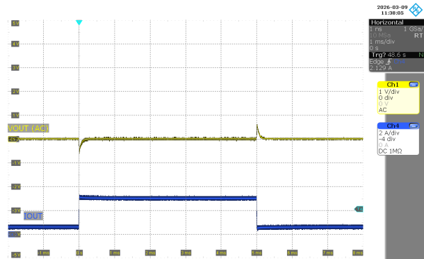
图 3-18. 负载阶跃 ( V_{IN} = 20V , V_{OUT} = 28V , I_{OUT} = 0.8A - 3A )
