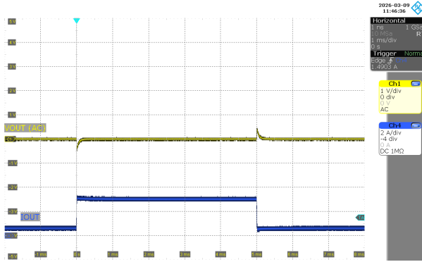
图 3-15. 负载阶跃 ( V_{IN} = 12V , V_{OUT} = 5V , I_{OUT} = 0.5A - 3A )
