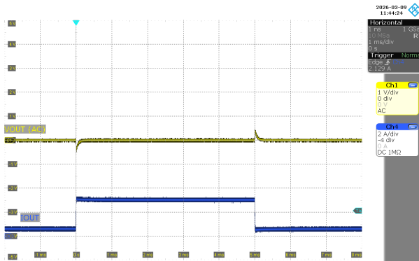
图 3-17. 负载阶跃 ( V_{IN} = 20V , V_{OUT} = 5V , I_{OUT} = 0.8A - 3A )
