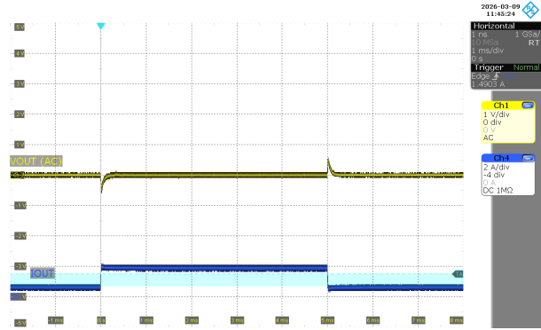
图 3-16. 负载阶跃 ( V_{IN} = 12V , V_{OUT} = 28V , I_{OUT} = 0.8A - 1.8A )
