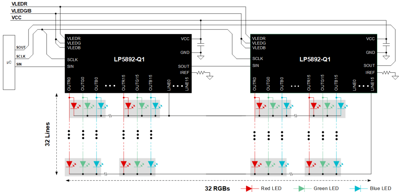
図 7-1. LP5892-Q1 with Dual Devices Stackable Connection
