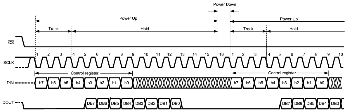
ADC082S021 Operational Timing Diagram
