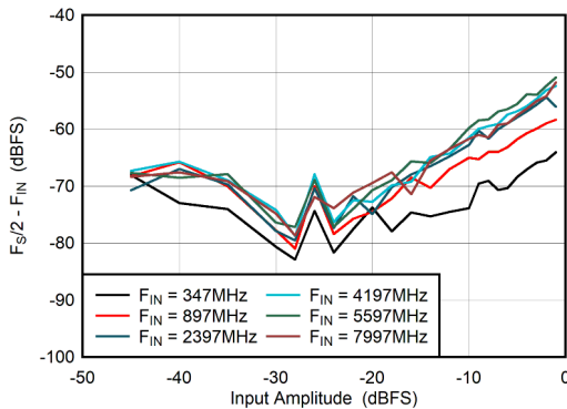
6-65. DES Mode: F_S/2 - F_{IN} vs Input Amplitude
