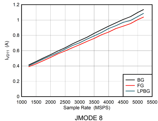
6-116. Dual Channel Mode: I_{VD11} vs Sample Rate
