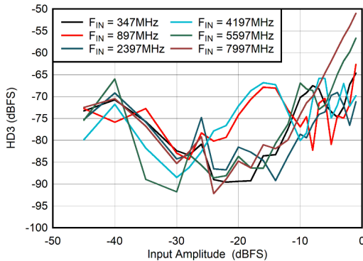
6-63. DES Mode: HD3 vs Input Amplitude
