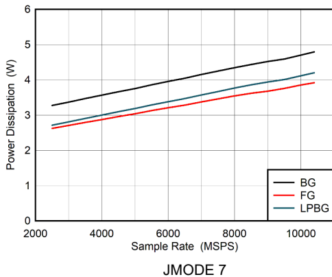
6-113. DES Mode: Power Dissipation vs Sample Rate
