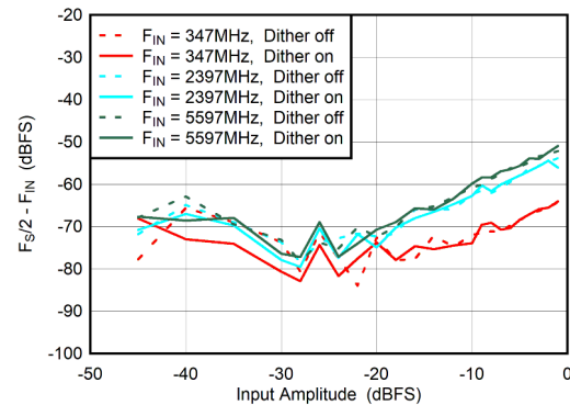
6-66. DES Mode: F_S/2 - F_{IN} vs Input Amplitude and Dither
