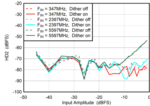
6-62. DES Mode: HD2 vs Input Amplitude and Dither
