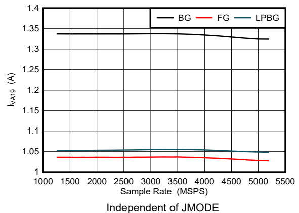
6-114. Dual Channel Mode: I_{VA19} vs Sample Rate
