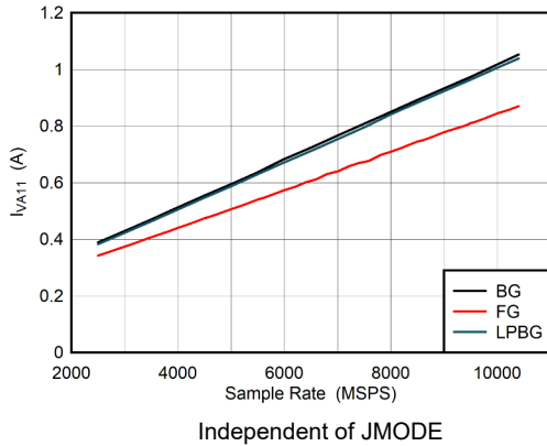
6-111. DES Mode: I_{VA11} vs Sample Rate
