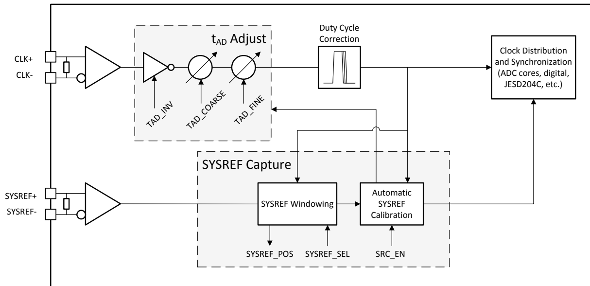
7-2. Clocking Subsystem
