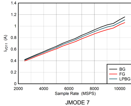
6-112. DES Mode: I_{VD11} vs Sample Rate
