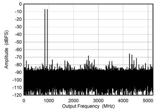
6-12. DES Mode: Two Tone FFT at 897 MHz
