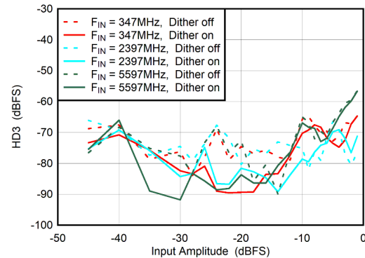
6-64. DES Mode: HD3 vs Input Amplitude and Dither
