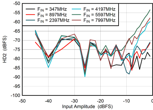
6-61. DES Mode: HD2 vs Input Amplitude
