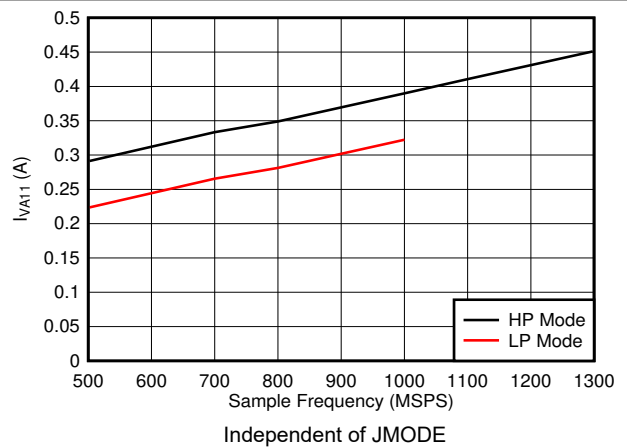
5-96. Dual Channel, I_{VA11} vs FS
