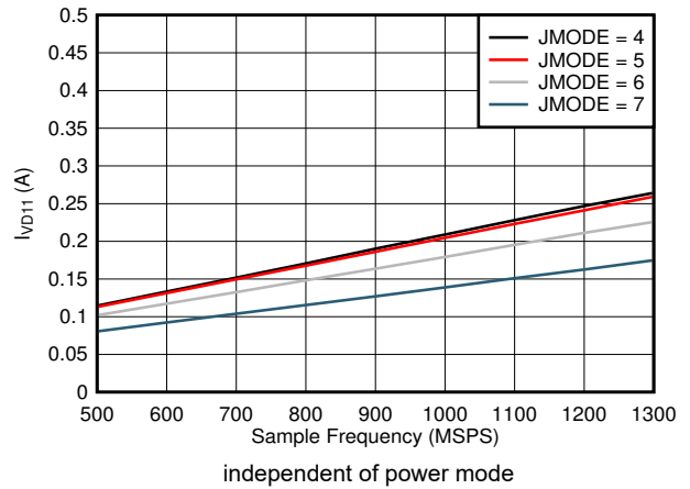
5-108. Single Channel, I_{VD11} vs FS and JMODE 4
