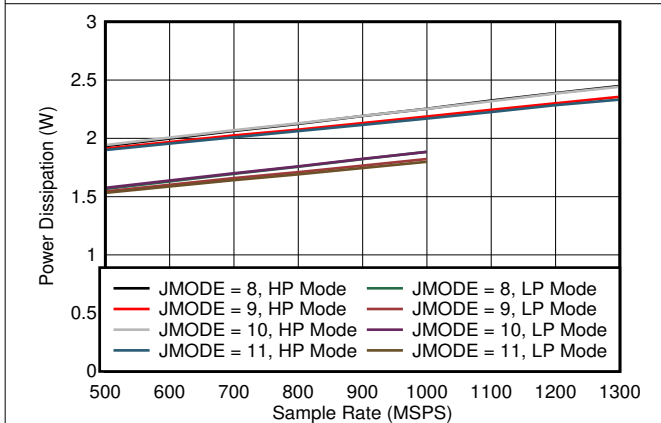
5-83. Quad Channel, Power Dissipation vs FS for JMODES 8 - 11
