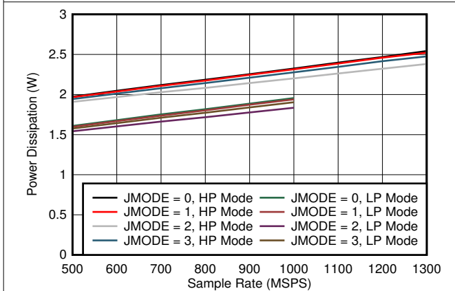
5-81. Quad Channel, Power Dissipation vs FS for JMODES 0 - 3
