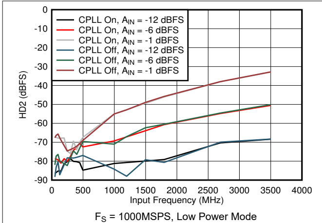
5-79. HD2 vs Input Frequency, CPLL and Input Amplitude
