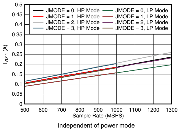
5-107. Single Channel, I_{VD11} vs FS and JMODE 0
