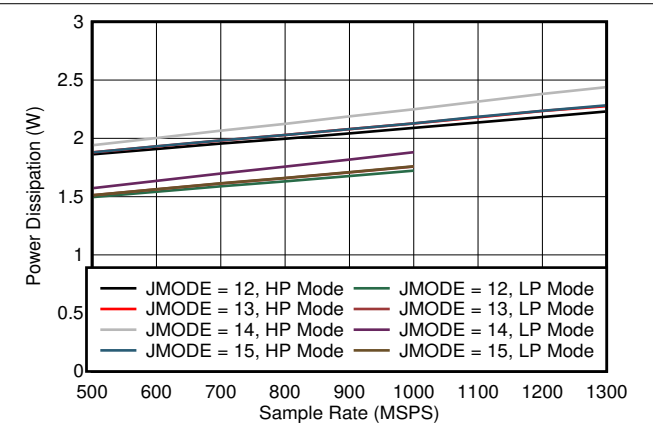
5-84. Quad Channel, Power Dissipation vs FS for JMODES 12 - 15
