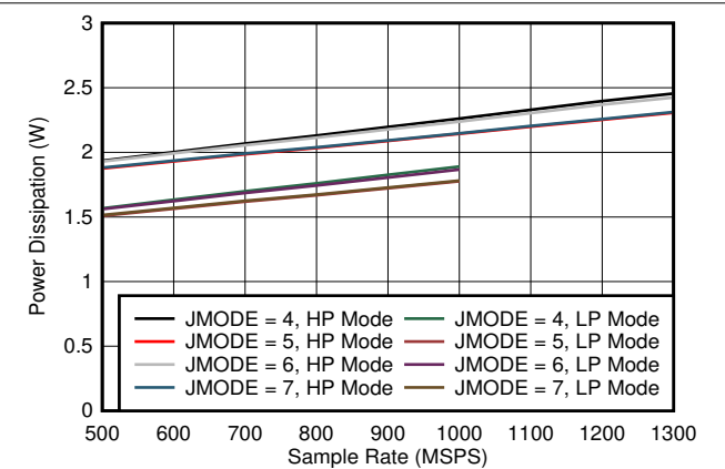
5-82. Quad Channel, Power Dissipation vs FS for JMODES 4 - 7
