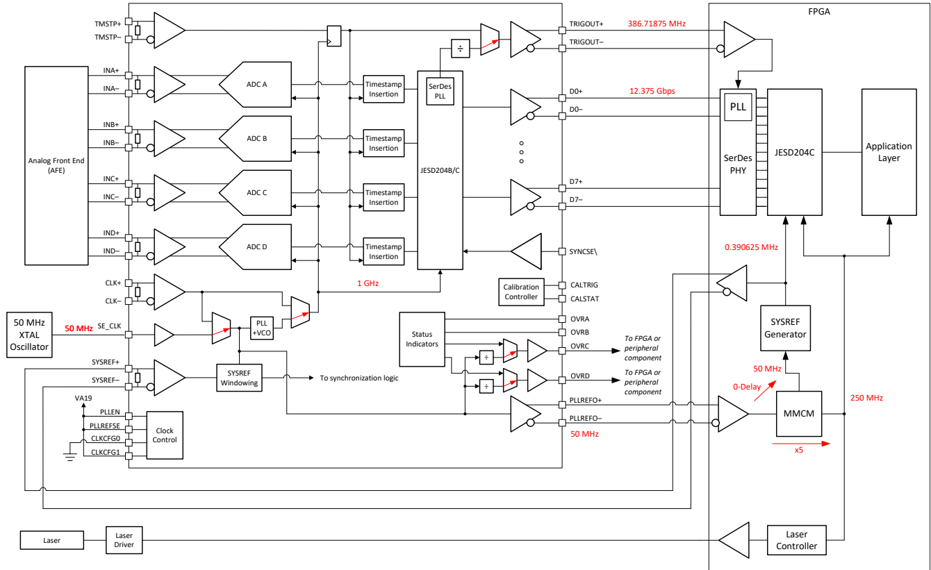
図 7-1. Typical Configuration for a LiDAR Digitizer
