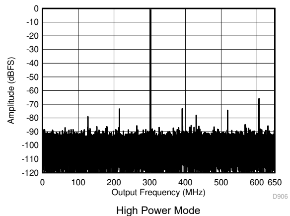
5-6. Single Tone FFT at 997 MHz and -1 dBFS
