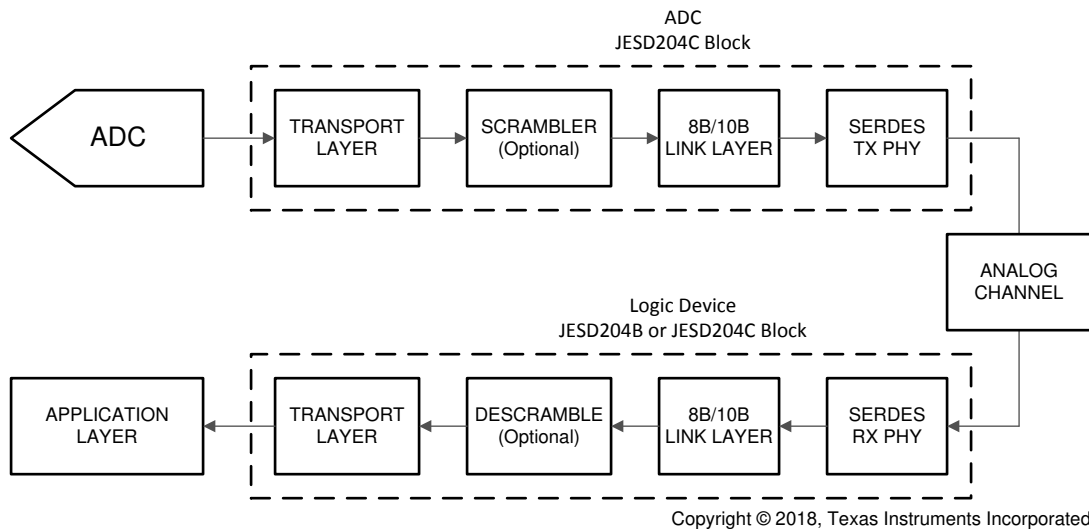
6-7. Simplified 8B/10B Encoded JESD204C Interface Diagram
