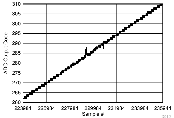
図 5-128. Background Calibration Core Transition (AC Signal Zoomed)
