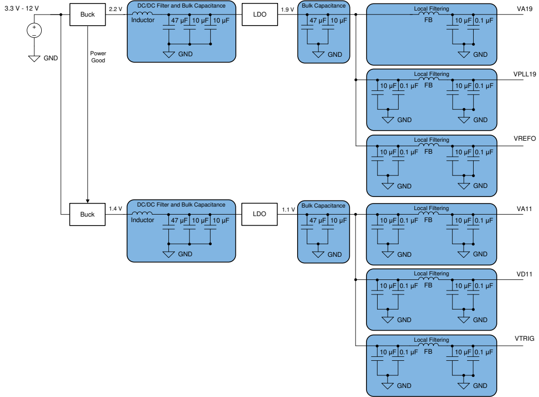
図 7-4. LDO Linear Regulator Approach Example
