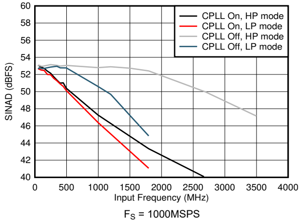
5-67. SINAD vs Input Frequency and CPLL
