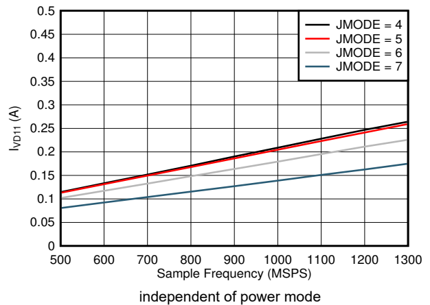
5-108. Single Channel, I_{VD11} vs FS and JMODE 4
