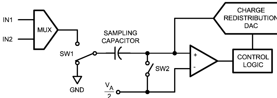
FIGURE 2. ADC102S021 in Hold Mode
