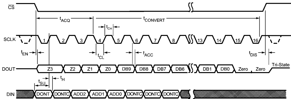
ADC102S021 Serial Timing Diagram
