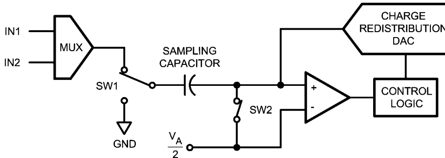
FIGURE 1. ADC102S021 in Track Mode
