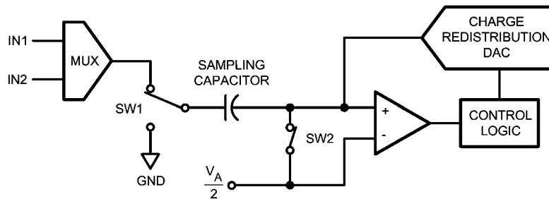
FIGURE 1. ADC102S051 in Track Mode
