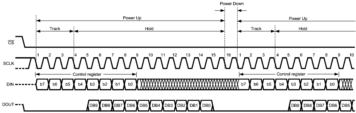
ADC102S051 Operational Timing Diagram
