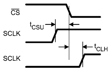
SCLK and CS Timing Parameters
