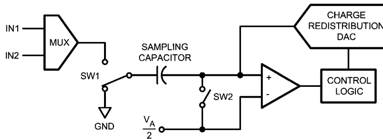
FIGURE 2. ADC102S051 in Hold Mode
