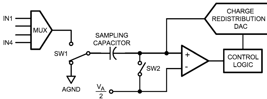
FIGURE 2. ADC104S051 in Hold Mode
