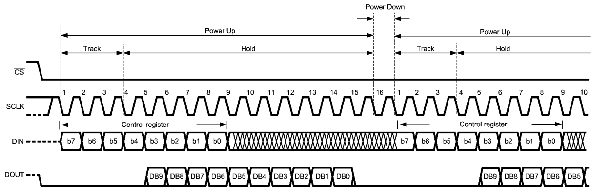
ADC104S051 Operational Timing Diagram
