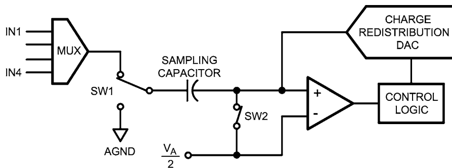
FIGURE 1. ADC104S051 in Track Mode
