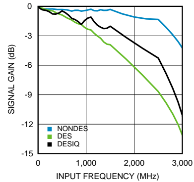
Figure 58. Full Power Bandwidth (ADC12D1600)
