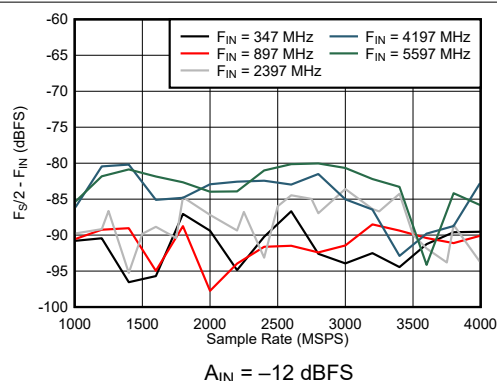
Figure 6-54. Dual Channel Mode: F_{\text{S}}/2 - F_{\text{IN}} vs Sample Rate and Input Frequency
