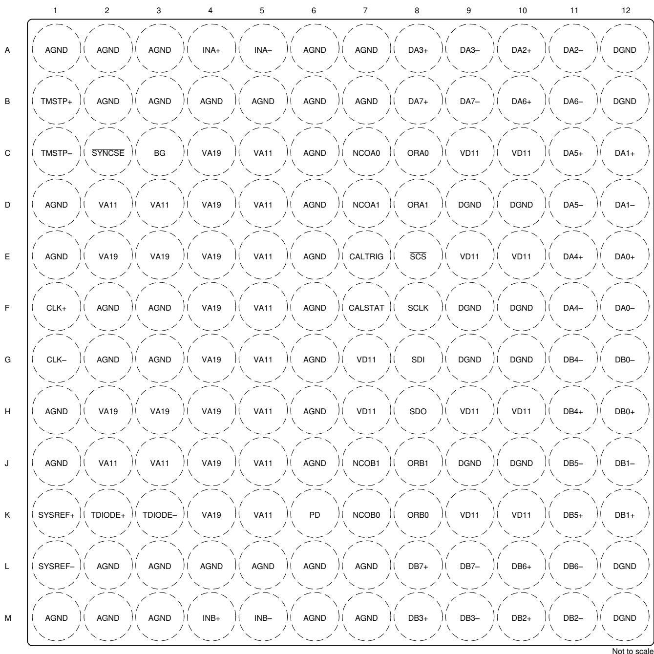
図 5-1. AAV Package, 144-Ball Flip Chip BGA, Top View
