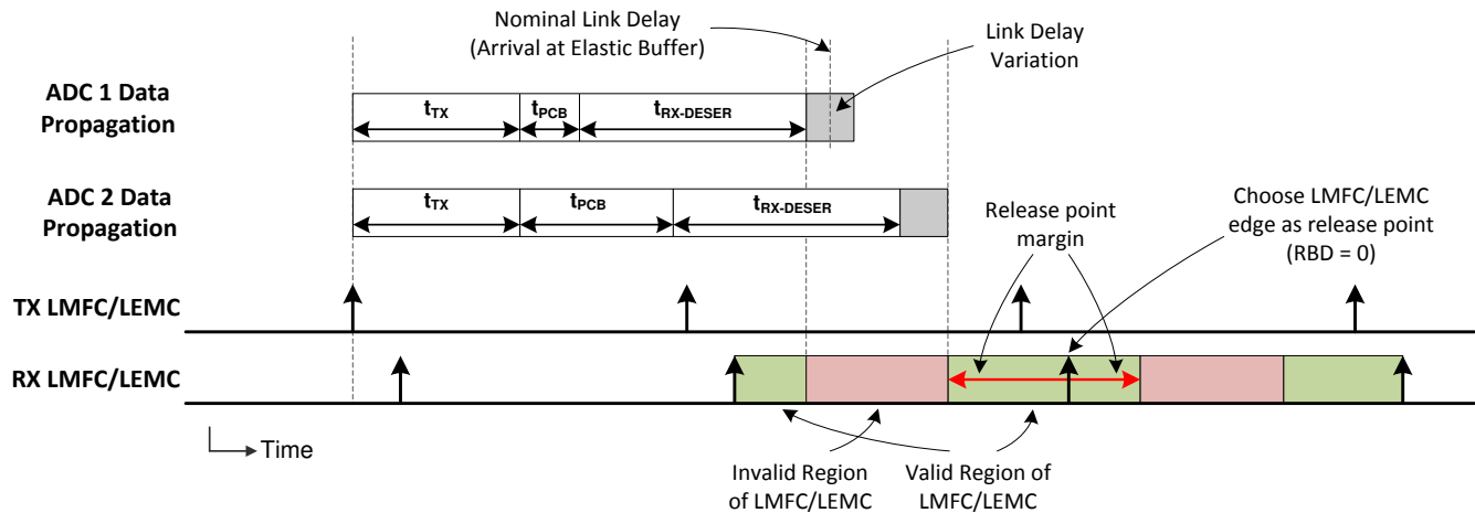
7-23. LMFC/LEMFC Valid Region Definition for Elastic Buffer Release Point Selection
