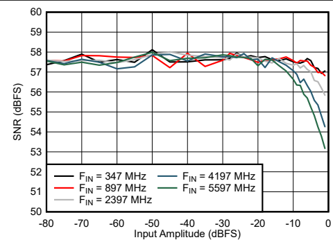
図 6-67. Dual Channel Mode: SNR vs Input Amplitude and Frequency
