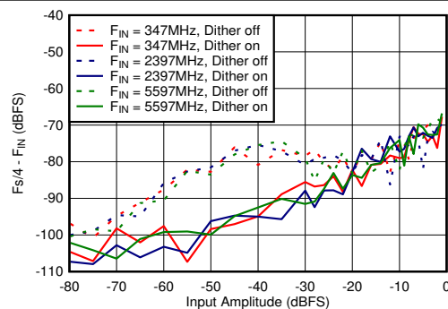
5-72. DES Mode: F_s/4 - F_{IN} vs Input Amplitude and Dither
