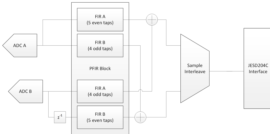
☒ 6-7. Alternate I/Q Correction-Type Filter Block Diagram
