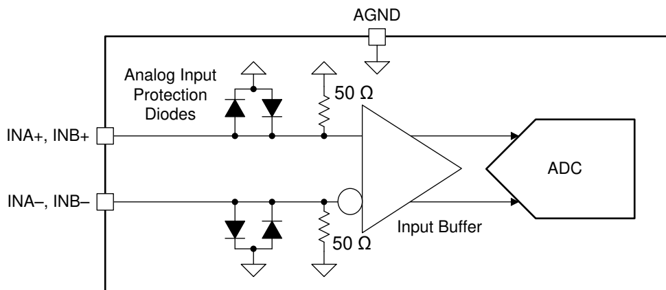
図 6-1. ADC12DJ5200-EP Analog Input Internal Termination and Protection Diagram
