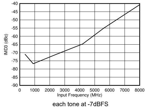
5-106. Dual Channel Mode: IMD3 vs Input Frequency
