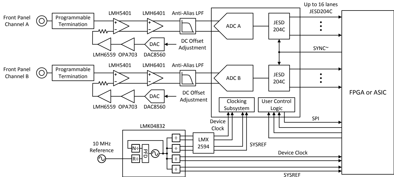
FIG 7-2. Typical Configuration for Reconfigurable Oscilloscope
