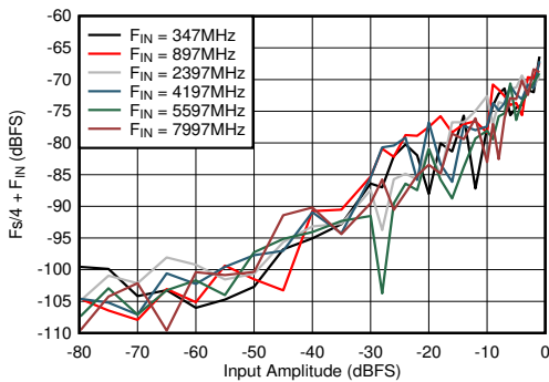
5-69. DES Mode: F_s/4 + F_{IN} vs Input Amplitude and Frequency
