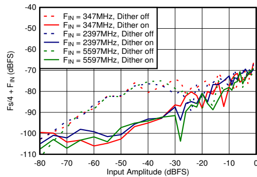
5-70. DES Mode: F_s/4 + F_{IN} vs Input Amplitude and Dither
