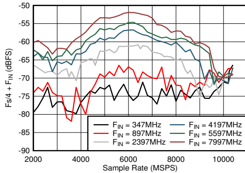
5-43. DES Mode: F_s/4 + F_{IN} vs Sample Rate and Input Frequency
