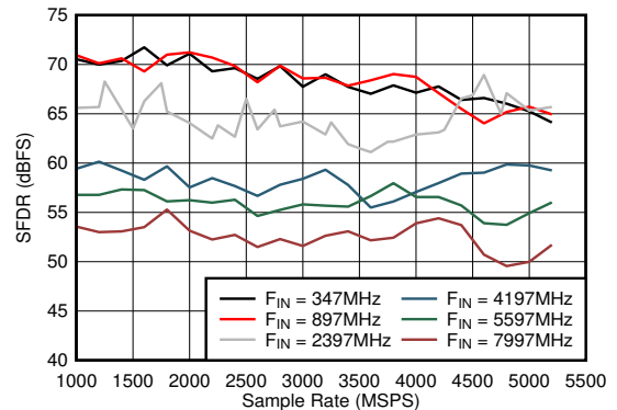
5-48. Dual Channel Mode: SFDR vs Sample Rate and Input Frequency A_{IN} = -1\text{ dBFS}
