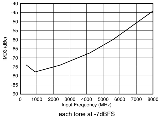
5-101. DES Mode: IMD3 vs Input Frequency
