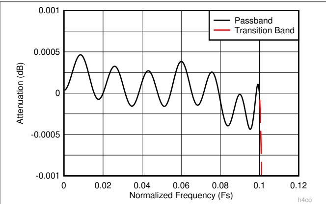
6-12. Decimate-by-4 Composite Zoomed Pass-Band Response
