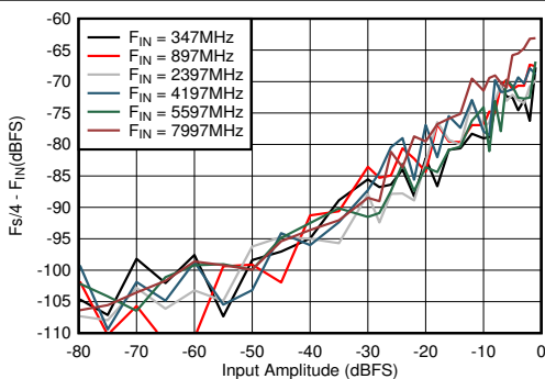
5-71. DES Mode: F_s/4 - F_{IN} vs Input Amplitude and Frequency
