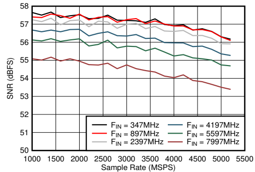
5-46. Dual Channel Mode: SNR vs Sample Rate and Input Frequency A_{IN} = -6\text{ dBFS}
