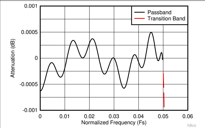
6-14. Decimate-by-8 Composite Zoomed Pass-Band Response
