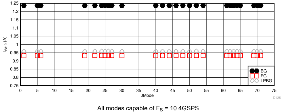
5-111. DES Mode: I_{VA19} vs JMODE at 10.4GSPS
