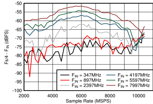
5-44. DES Mode: F_s/4 - F_{IN} vs Sample Rate and Input Frequency
