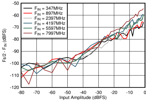
5-67. DES Mode: F_s/2 - F_{IN} vs Input Amplitude and Frequency
