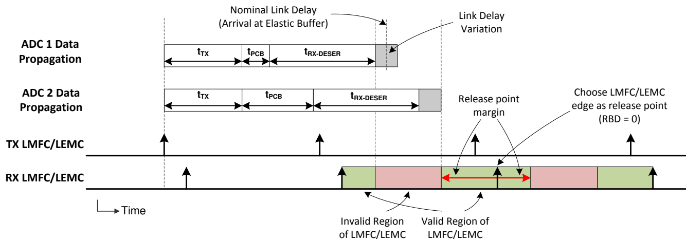
❏ 6-23. LMFC/LEMFC Valid Region Definition for Elastic Buffer Release Point Selection
