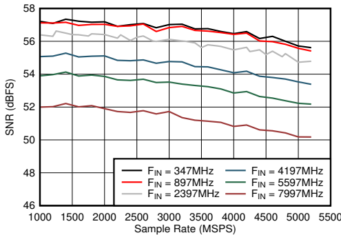
5-45. Dual Channel Mode: SNR vs Sample Rate and Input Frequency A_{IN} = -1\text{ dBFS}
