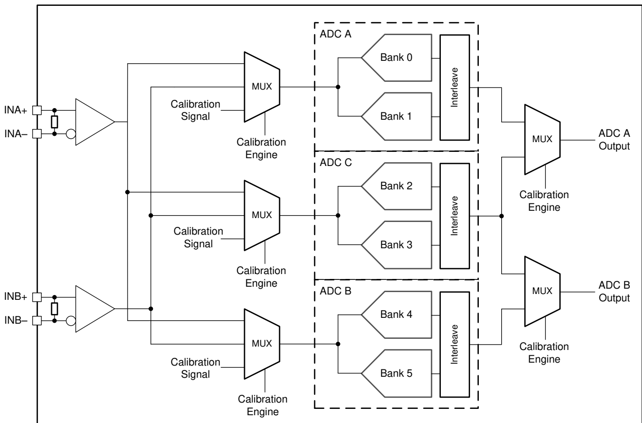
図 6-25. ADC12DJ5200-EP Calibration System Block Diagram
