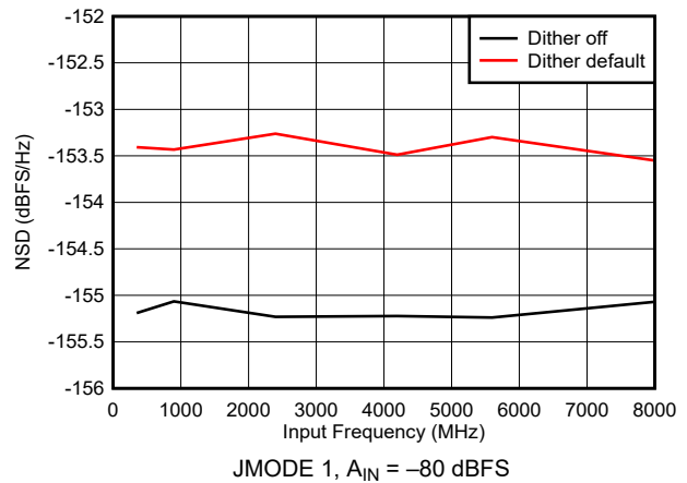
图 5-36. DES Mode: NSD vs Input Frequency
