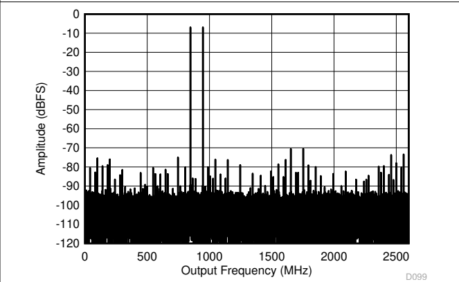
5-22. Dual Channel Mode: Single Tone FFT at 7997 MHz
