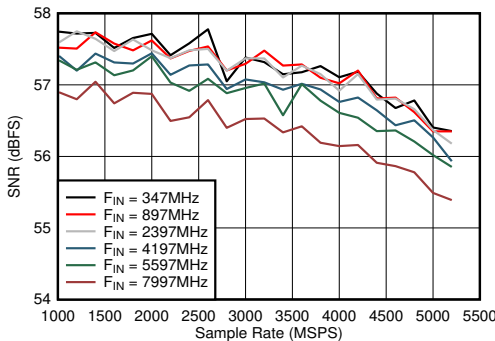
5-47. Dual Channel Mode: SNR vs Sample Rate and Input Frequency A_{IN} = -12\text{ dBFS}
