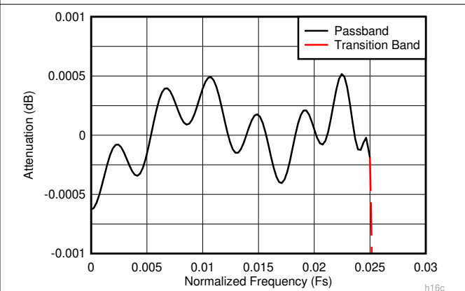
6-16. Decimate-by-16 Composite Zoomed Pass-Band Response
