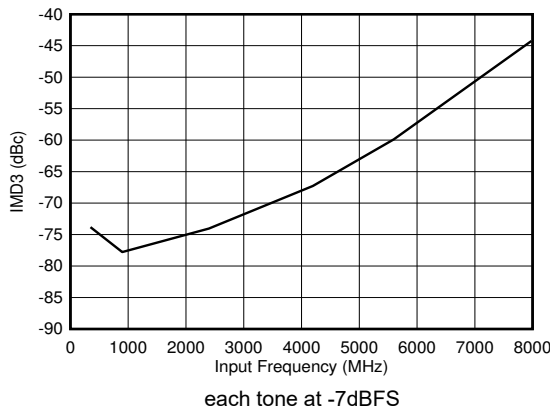
6-101. DES Mode: IMD3 vs Input Frequency
