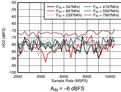
6-37. DES Mode: HD2 vs Sample Rate and Input Frequency
