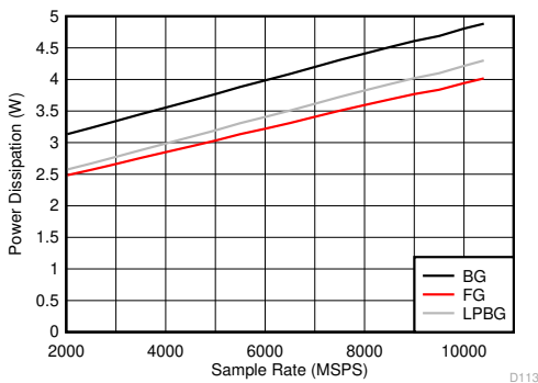
6-129. DES Mode: Power Dissipation vs Sample Rate
