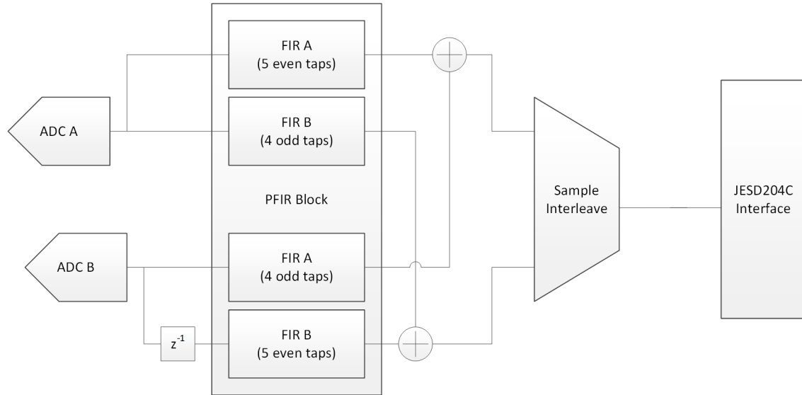
FIG 7-7. Alternate I/Q Correction-Type Filter Block Diagram
