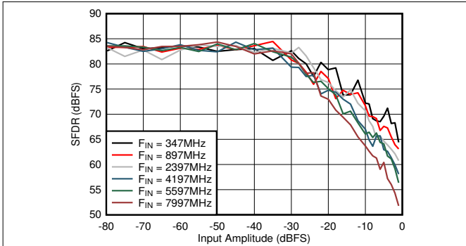
Figure 6-61. DES Mode: SFDR vs Input Amplitude and Frequency
