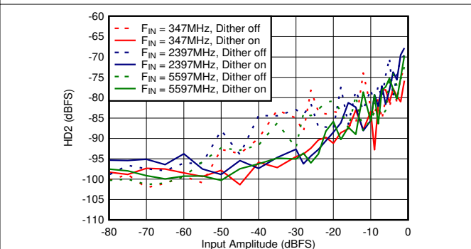
Figure 6-64. DES Mode: HD2 vs Input Amplitude and Dither
