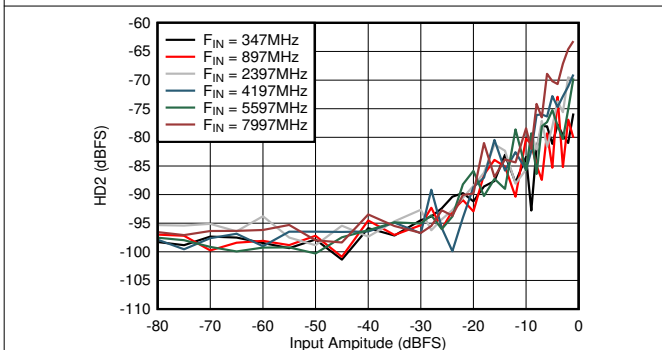
Figure 6-63. DES Mode: HD2 vs Input Amplitude and Frequency
