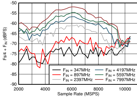
6-43. DES Mode: F_s/4 + F_{\text{IN}} vs Sample Rate and Input Frequency
