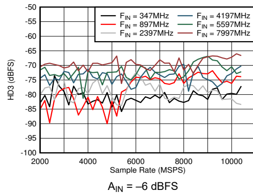
6-40. DES Mode: HD3 vs Sample Rate and Input Frequency
