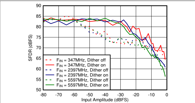
Figure 6-62. DES Mode: SFDR vs Input Amplitude and Dither
