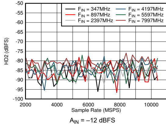
6-38. DES Mode: HD2 vs Sample Rate and Input Frequency
