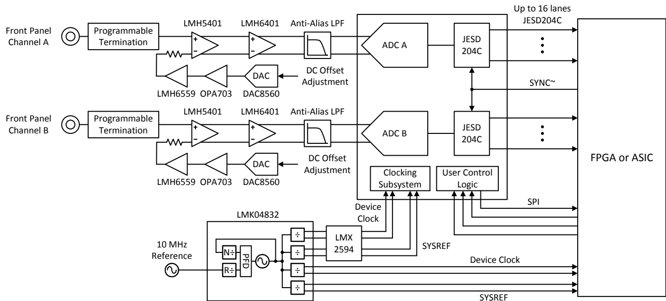
FIG 8-2. Typical Configuration for Reconfigurable Oscilloscope
