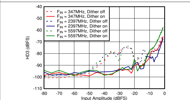
Figure 6-66. DES Mode: HD3 vs Input Amplitude and Dither
