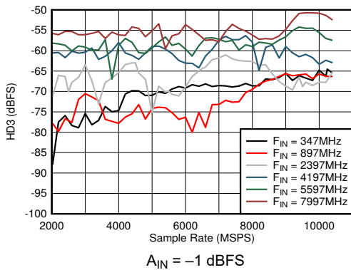
6-39. DES Mode: HD3 vs Sample Rate and Input Frequency
