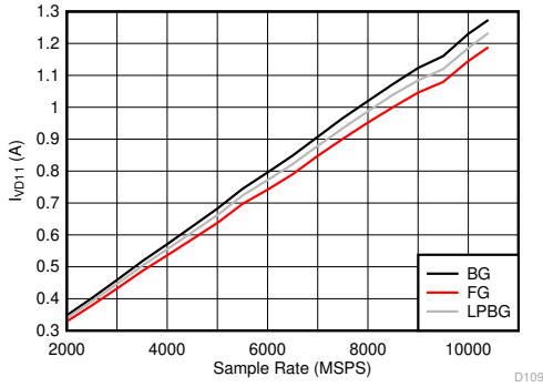
6-127. DES Mode: I_{VD11} vs Sample Rate
