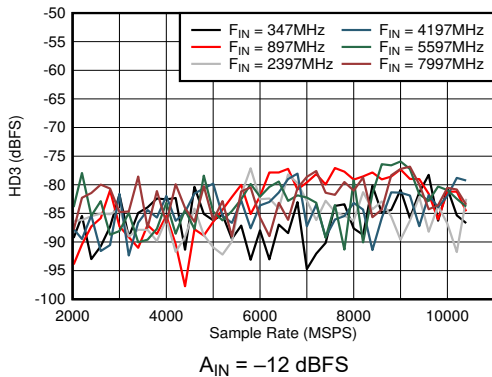
6-41. DES Mode: HD3 vs Sample Rate and Input Frequency
