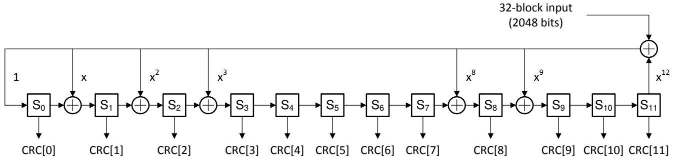
7-21. CRC-12 Parity Bit Generator
