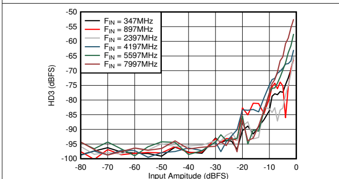
Figure 6-65. DES Mode: HD3 vs Input Amplitude and Frequency
