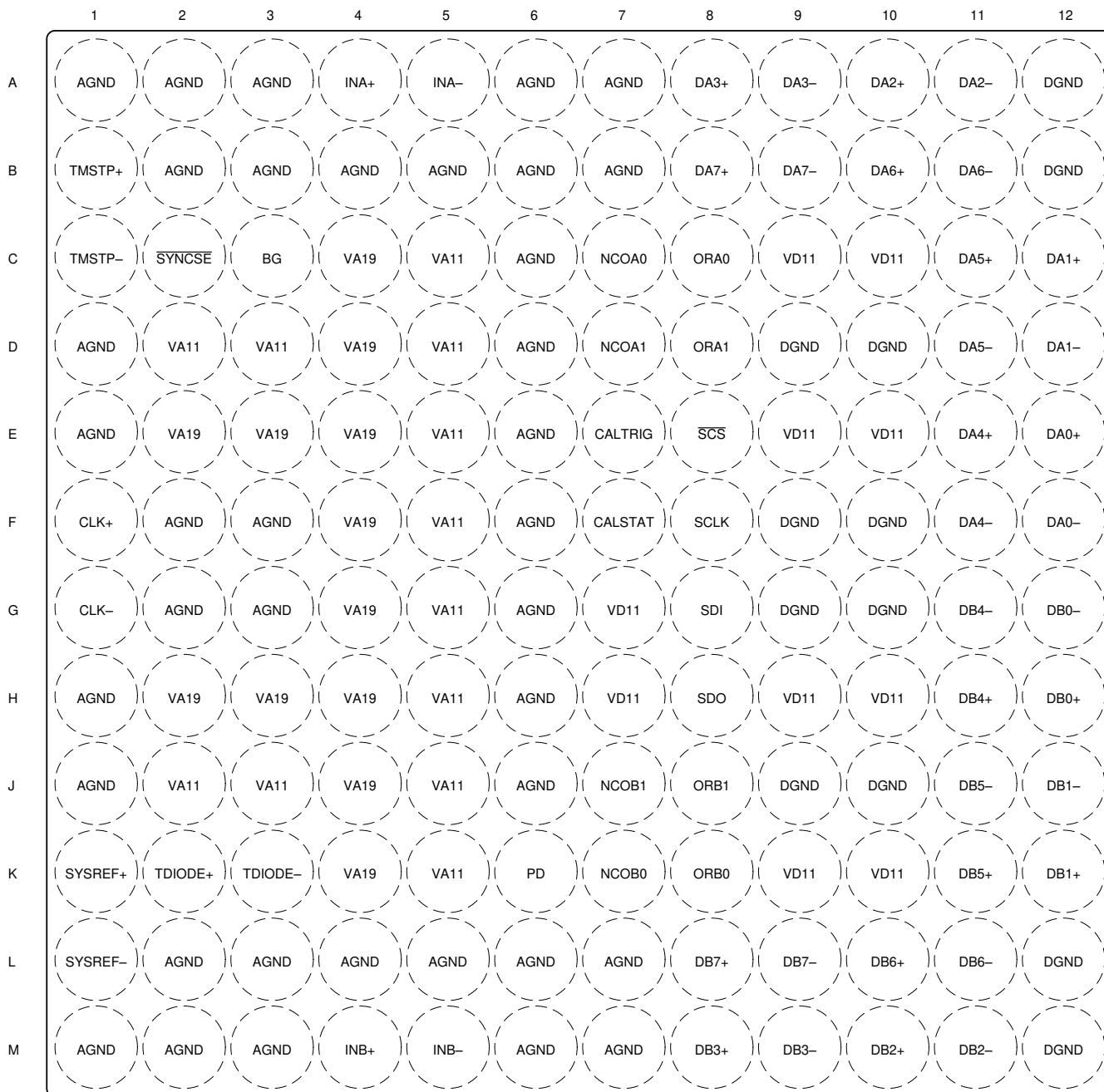
5-1. ALR Package, 144-Ball Flip Chip BGA Top View
