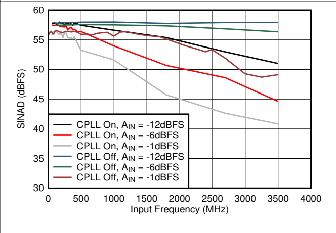
Figure 5-50. SINAD vs A_{IN} and C-PLL
