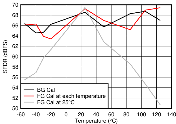
5-65. SFDR vs Temperature
