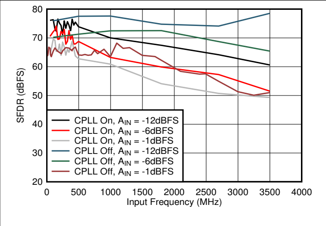
Figure 5-48. SFDR vs A_{IN} and C-PLL
