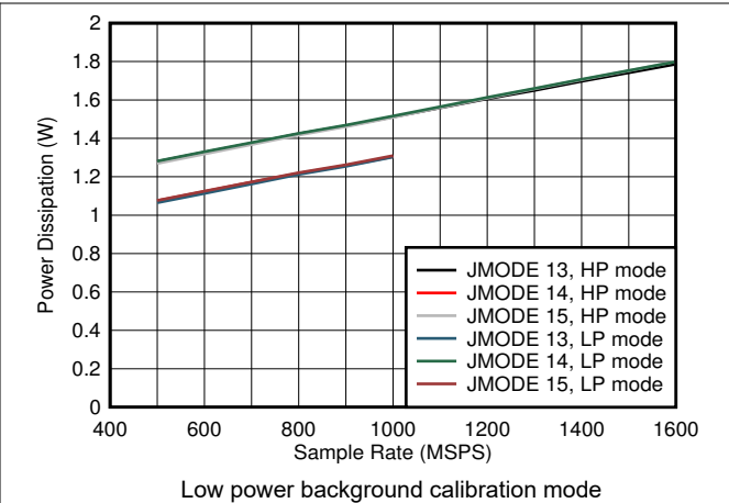
5-92. Dual Channel, Power Dissipation vs F_S and JMODE 13 - 15
