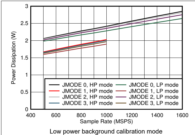
5-79. Quad Channel, Power Dissipation vs F_S and JMODES 0 - 3
