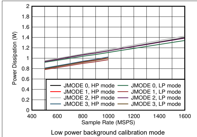
5-99. Single Channel, Power Dissipation vs F_S and JMODE 0 - 3
