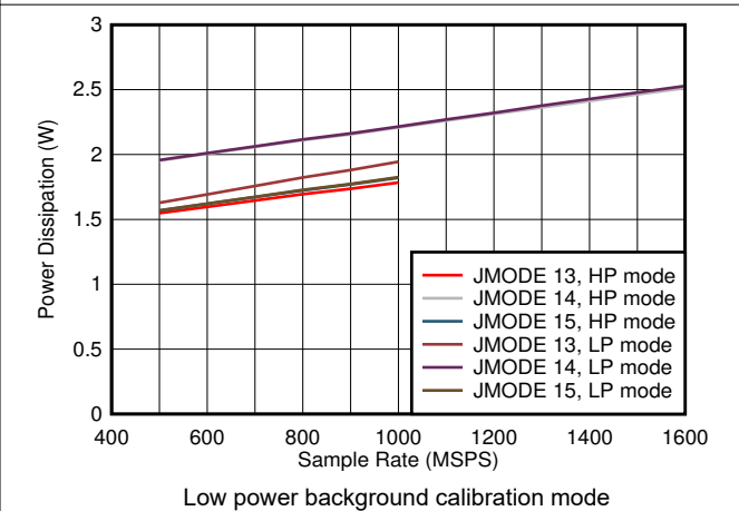
5-82. Quad Channel, Power Dissipation vs F_S and JMODE 13 - 15
