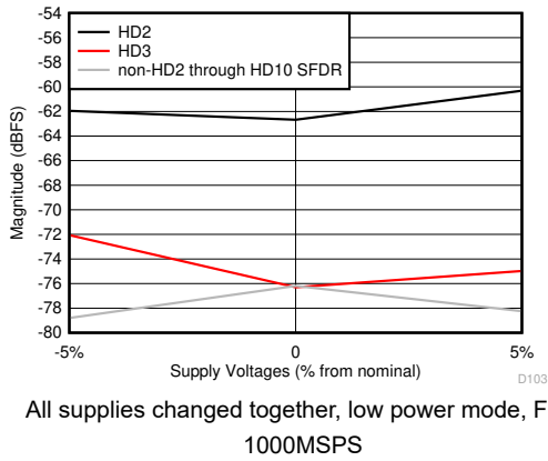
5-63. HD2, HD3 and Worst non-HD Spur vs Supply Voltage
