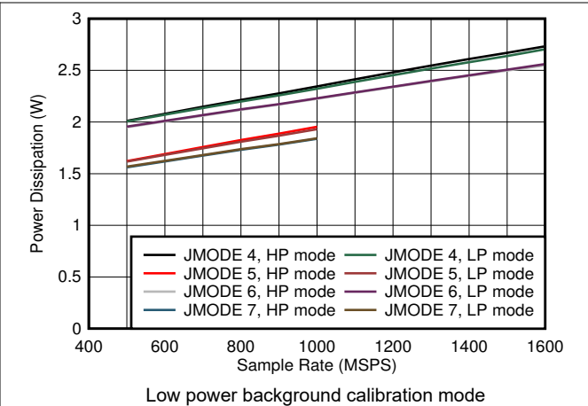
5-80. Quad Channel, Power Dissipation vs F_S and JMODE 4 - 7
