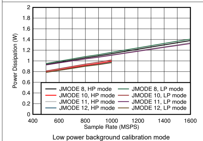
5-101. Single Channel, Power Dissipation vs F_S and JMODE 8 - 12
