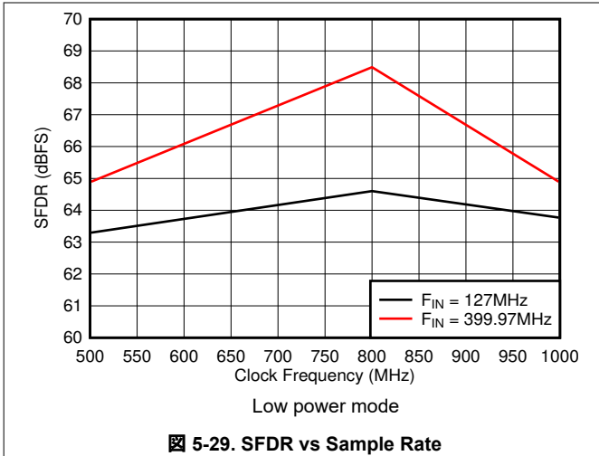
5-29. SFDR vs Sample Rate
