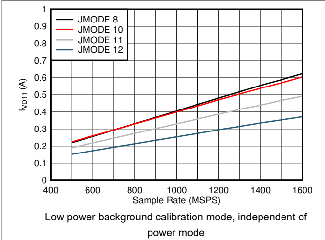
图 5-87. Quad Channel, I_{VD11} vs F_S and JMODE 8 - 12
