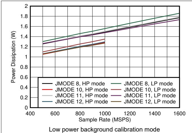
5-91. Dual Channel, Power Dissipation vs F_S and JMODE 8 - 12
