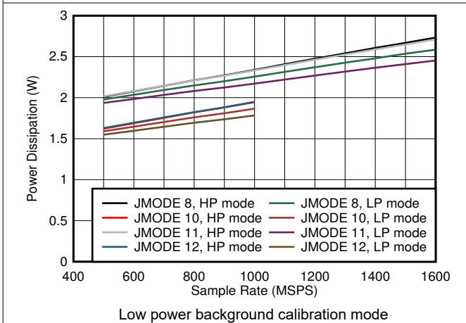
5-81. Quad Channel, Power Dissipation vs F_S and JMODE 8 - 12
