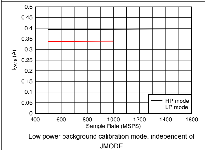
5-93. Dual Channel, I_{VA19} vs F_S
