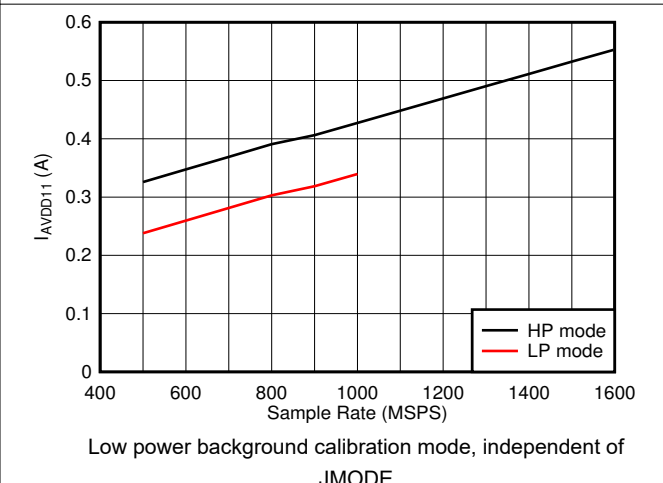
5-94. Dual Channel, I_{VA11} vs F_S
