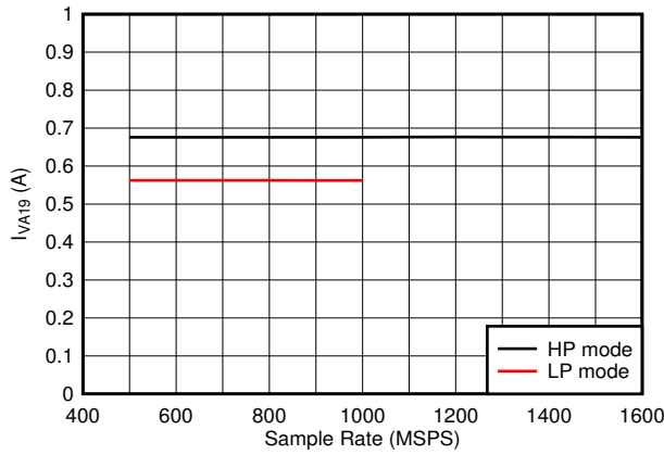
Figure 5-83. Quad Channel, I_{VA19} vs F_S
