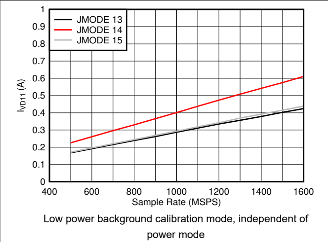
图 5-88. Quad Channel, I_{VD11} vs F_S and JMODE 13 - 15
