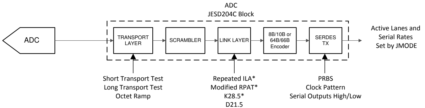
6-12. Test Mode Insertion Points
