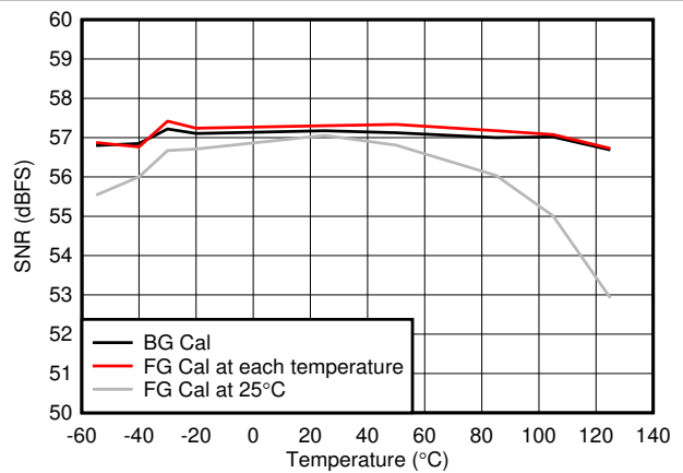
☒ 5-64. SNR vs Temperature
