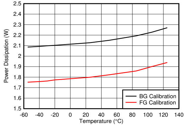
5-122. Dual Channel, Power Dissipation vs Temperature
