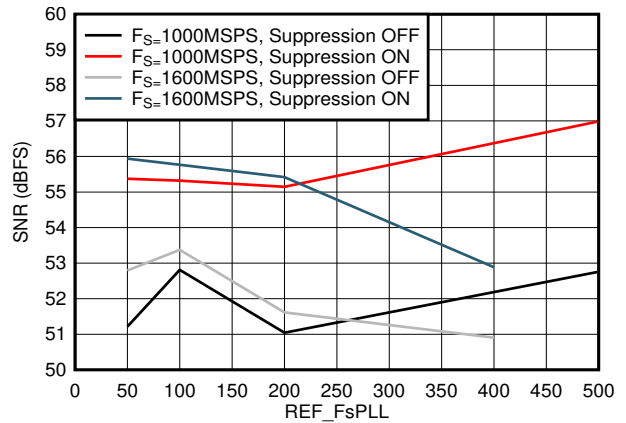
5-38. SNR vs F REF and Suppression
