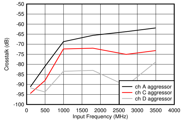
5-78. Crosstalk to Channel B vs F_{IN}
