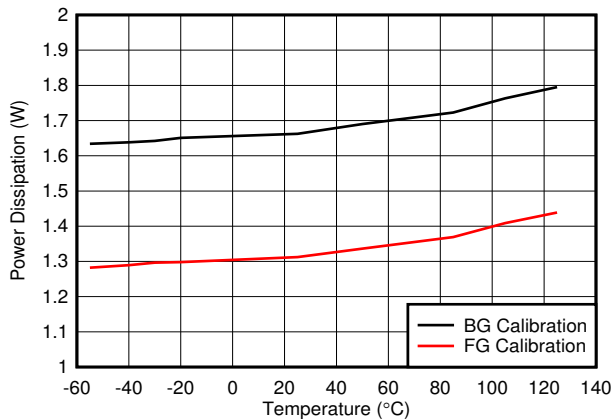
5-123. Single Channel, Power Dissipation vs Temperature
