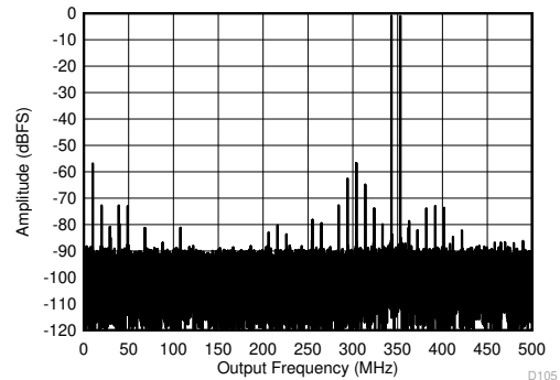
5-70. Two Tone FFT at 1798MHz
