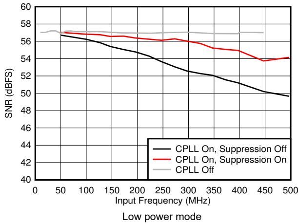
5-45. SNR vs F_{IN} and C-PLL modes
