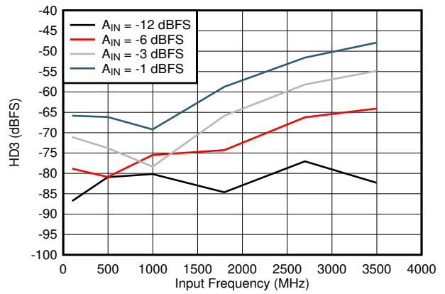
5-22. HD3 vs Input Frequency
