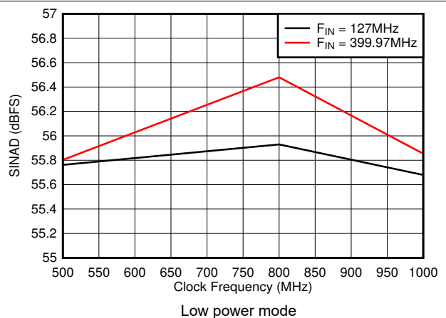
5-30. SINAD vs Sample Rate
