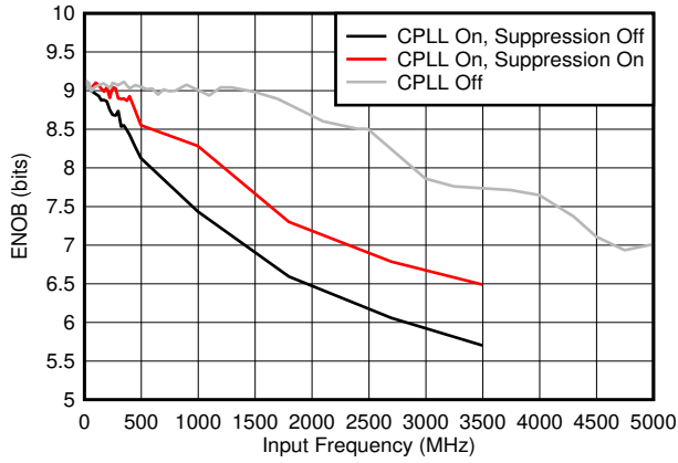
5-43. ENOB vs F_{IN} and C-PLL modes
