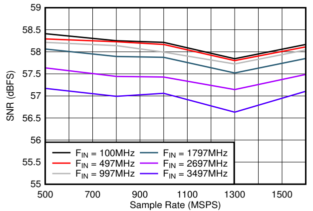
5-24. SNR vs Sample Rate
