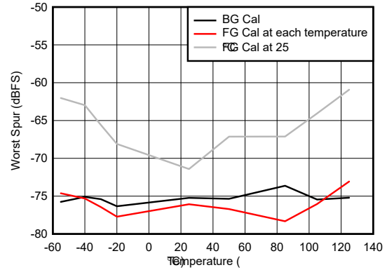
5-68. Worst Spur vs Temperature
