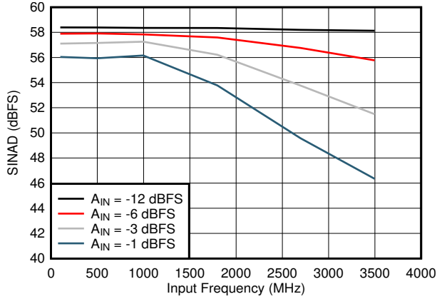
5-19. SINAD vs Input Frequency
