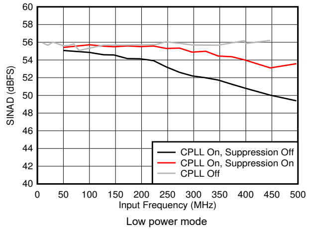
5-46. SINAD vs F_{IN} and C-PLL modes
