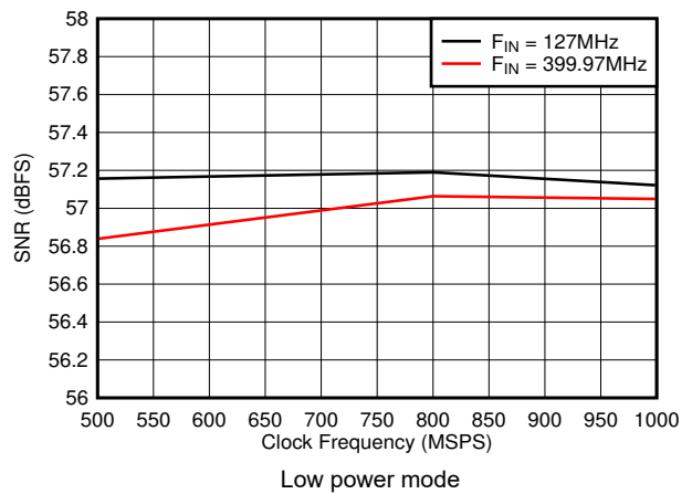
5-28. SNR vs Sample Rate
