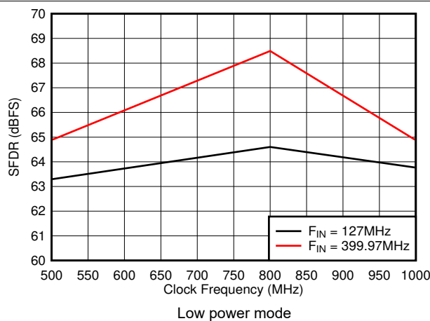
5-29. SFDR vs Sample Rate
