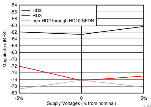
☒ 5-61. HD2, HD3 and Worst non-HD Spur vs Supply Voltage
