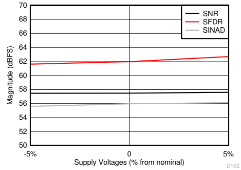
☒ 5-62. SNR, SFDR and SINAD vs Supply Voltages
