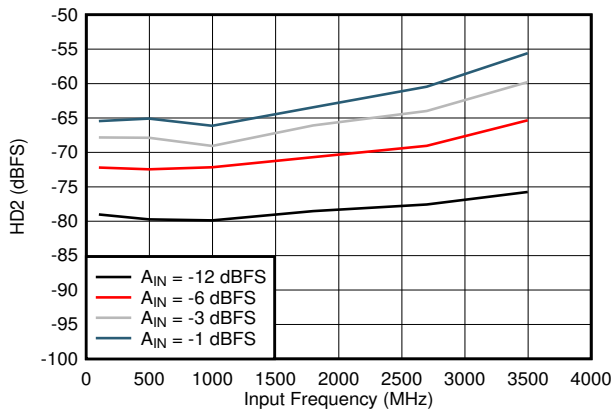
5-21. HD2 vs Input Frequency
