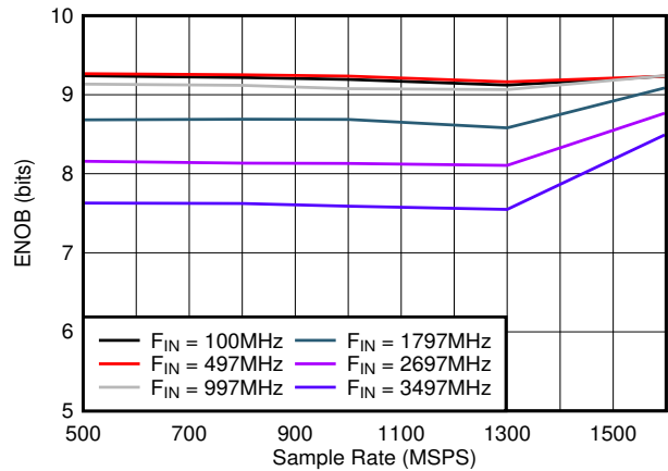
5-26. ENOB vs Sample Rate
