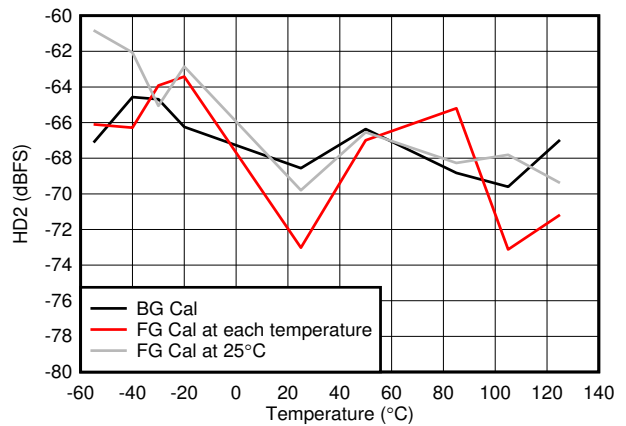
☒ 5-66. HD2 vs Temperature
