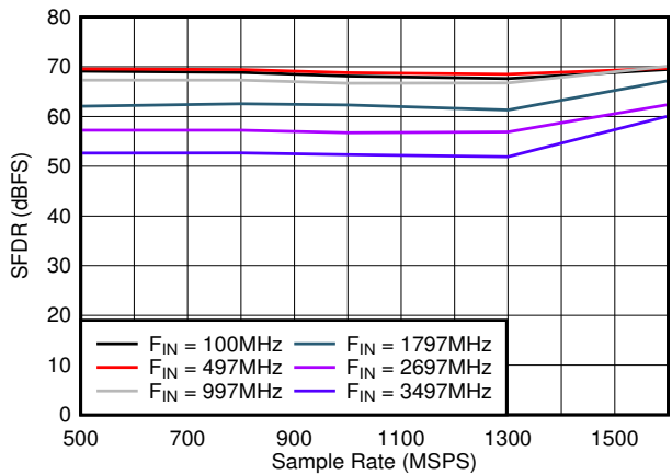
5-23. SFDR vs Sample Rate
