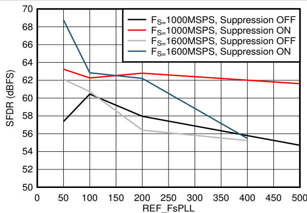
5-39. SFDR vs F REF and Suppression
