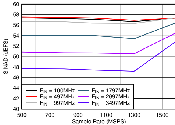
5-25. SINAD vs Sample Rate
