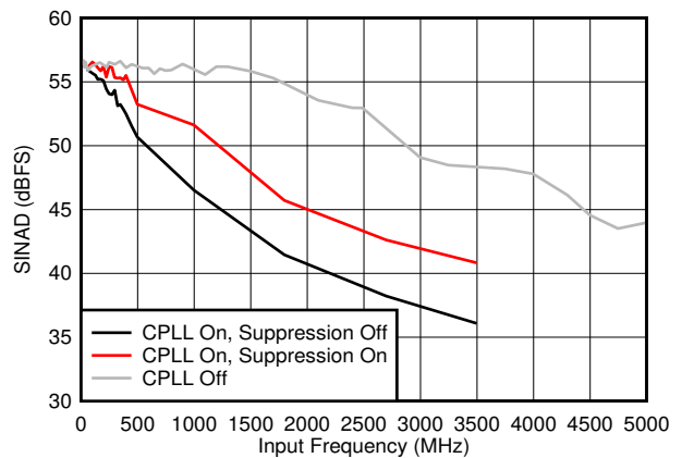
5-42. SINAD vs F IN and C-PLL modes
