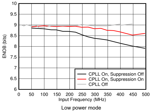
5-47. ENOB vs F_{IN} and C-PLL modes
