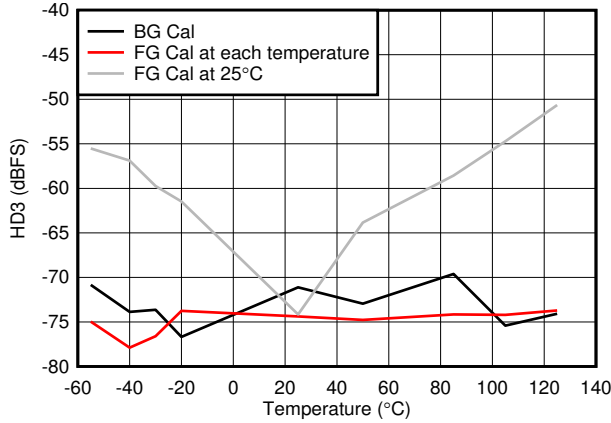
5-67. HD3 vs Temperature
