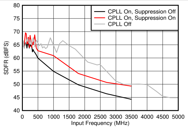
5-40. SFDR vs F IN and C-PLL modes
