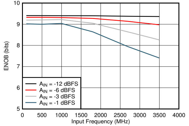
5-20. ENOB vs Input Frequency
