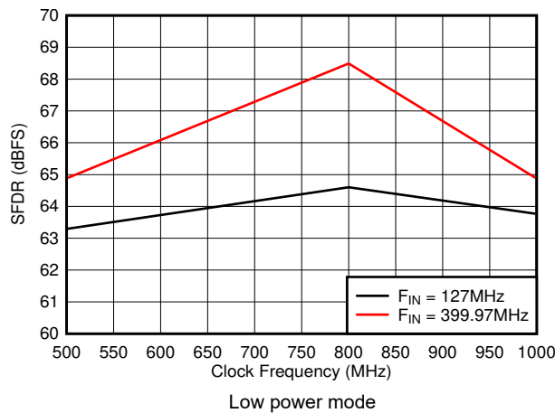
5-27. SFDR vs Sample Rate
