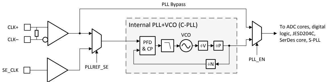
8-4. Converter PLL (C-PLL) Architecture
