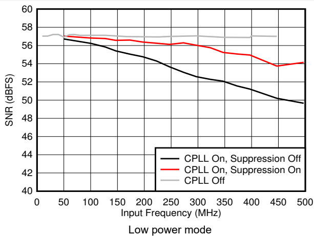
7-45. SNR vs F_{IN} and C-PLL modes
