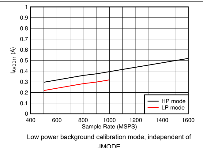
7-104. Single Channel, I_{VA11} vs F_S
