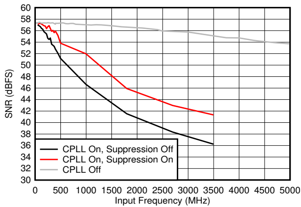
7-41. SNR vs F_{IN} and C-PLL modes
