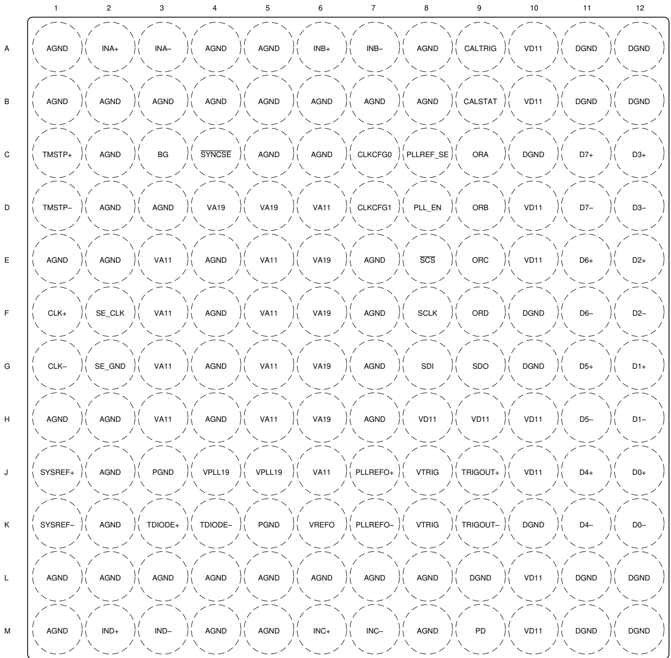
6-1. Quad Channel ALR Package, 144-Ball Flip Chip BGA (Top View)
