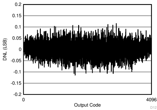
7-1. DNL vs Code
