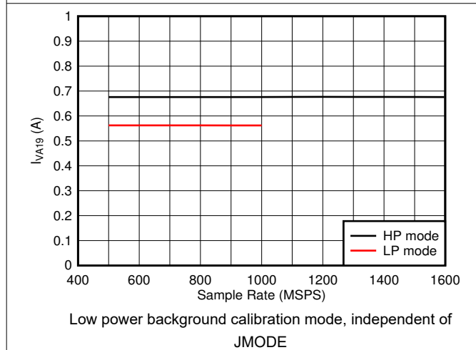
7-83. Quad Channel, I_{VA19} vs F_S
