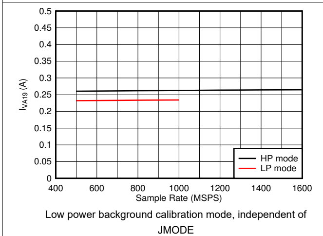
7-103. Single Channel, I_{VA19} vs F_S
