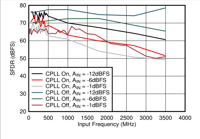
7-48. SFDR vs A_{IN} and C-PLL
