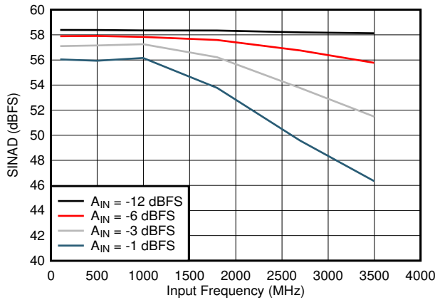
7-19. SINAD vs Input Frequency
