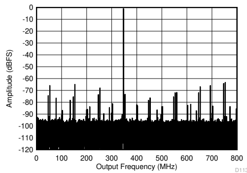
7-6. Single Tone FFT at 347 MHz and -1 dBFS
