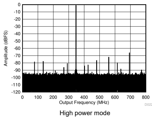
7-4. Single Tone FFT at 347 MHz and -1 dBFS
