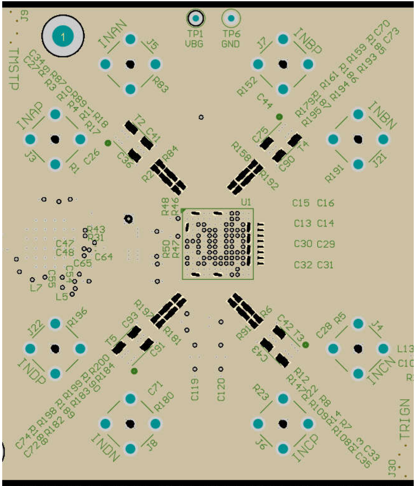
9-6. GND1 Cutouts to Optimize Impedance of Component Pads
