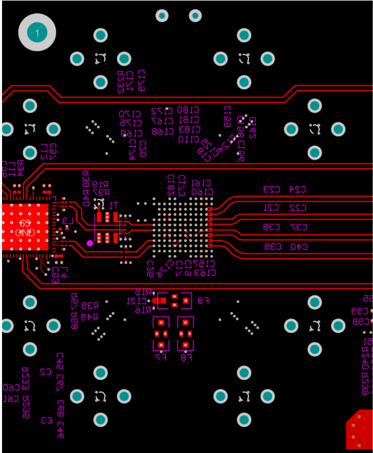
9-7. Bottom Layer Routing: CLK±, SYSREF and D[7:4]± Routing
