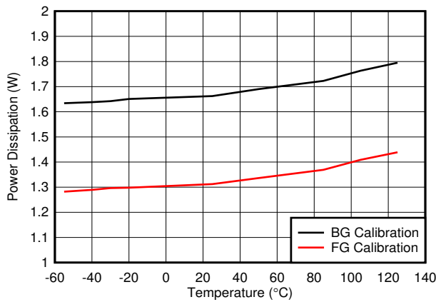
7-123. Single Channel, Power Dissipation vs Temperature
