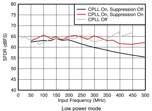
7-44. SFDR vs F_{IN} and C-PLL modes
