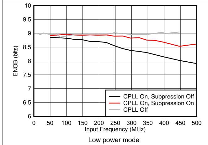
7-47. ENOB vs F_{IN} and C-PLL modes
