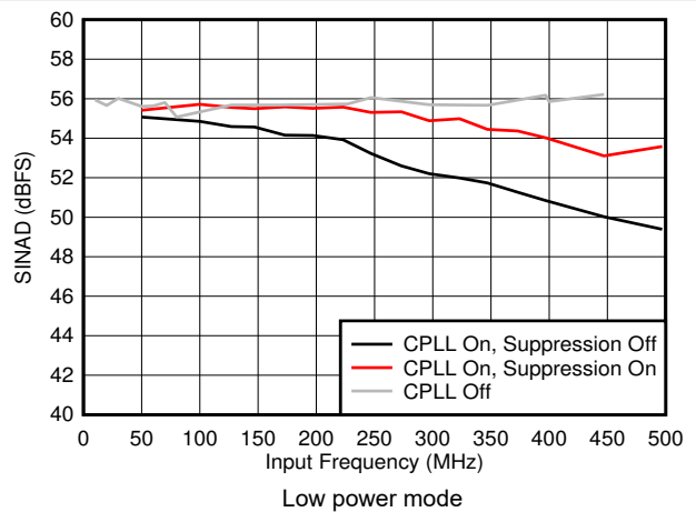
7-46. SINAD vs F_{IN} and C-PLL modes
