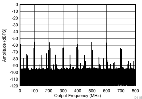
High power mode, C-PLL on, Noise suppression off 7-9. Single Tone FFT at 997 MHz and -1 dBFS
