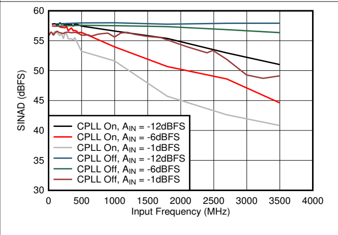
7-50. SINAD vs A_{IN} and C-PLL
