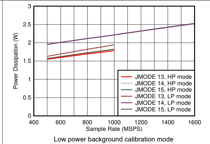
7-82. Quad Channel, Power Dissipation vs F_S and JMODE 13 - 15
