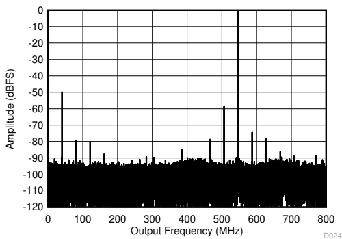
High power mode 7-11. Single Tone FFT at 3797 MHz and -1 dBFS
