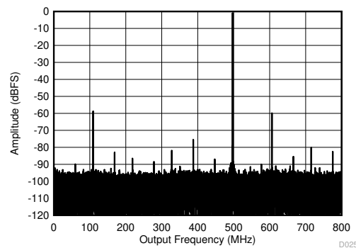
High power mode 7-10. Single Tone FFT at 1797 MHz and -1 dBFS
