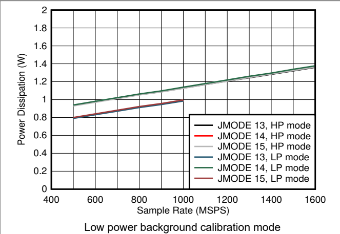
7-102. Single Channel, Power Dissipation vs F_S and JMODE 13 - 15
