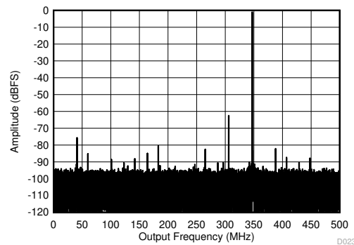
Low power mode, F_S = 1000 MSPS 7-12. Single Tone FFT at 347 MHz and -1 dBFS
