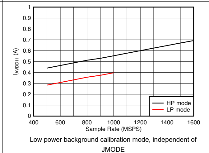
7-84. Quad Channel, I_{VA11} vs F_S
