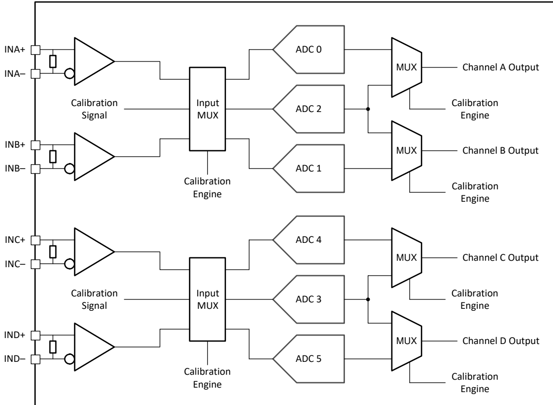
8-13. Quad Channel Calibration System Block Diagram
