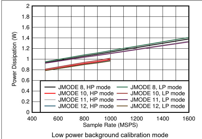
7-101. Single Channel, Power Dissipation vs F_S and JMODE 8 - 12
