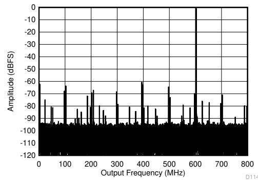
High power mode, C-PLL on 7-8. Single Tone FFT at 997 MHz and -1 dBFS
