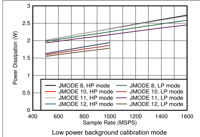
7-81. Quad Channel, Power Dissipation vs F_S and JMODE 8 - 12
