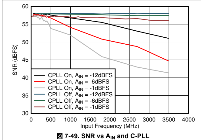
7-49. SNR vs A_{IN} and C-PLL
