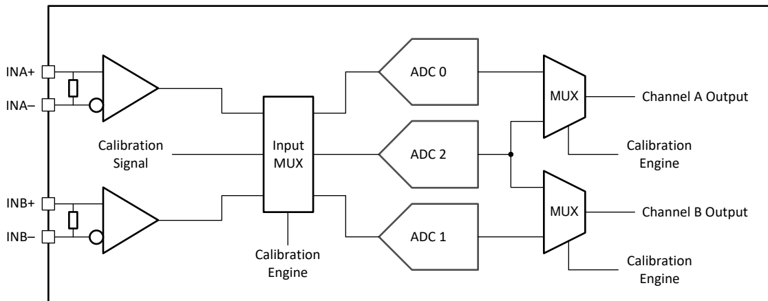
8-14. DualChannel Calibration System Block Diagram
