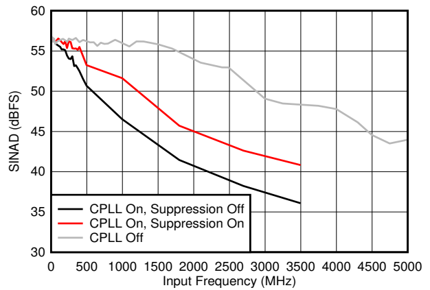
7-42. SINAD vs F_{IN} and C-PLL modes
