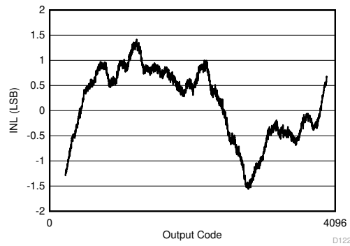
7-2. INL vs Code
