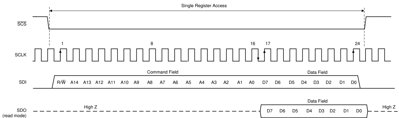
8-16. Serial Interface Protocol: Single Read/Write
