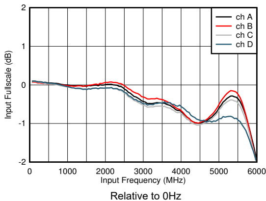
7-3. Input Fullscale vs Frequency
