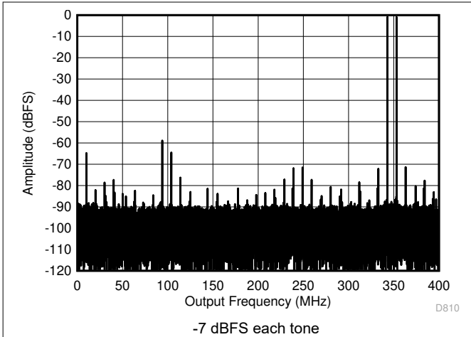
5-69. Two Tone FFT at 347 MHz in Low Power Mode
