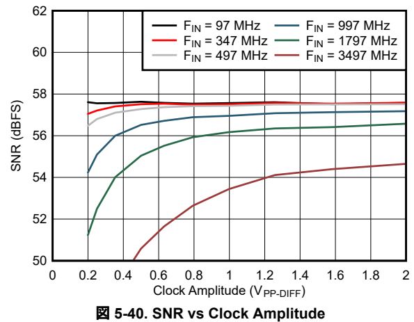
Figure 5-40. SNR vs Clock Amplitude
