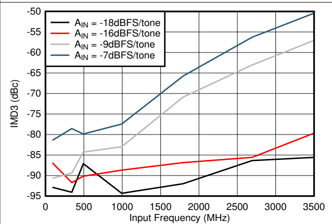
5-72. IMD3 vs Input Frequency
