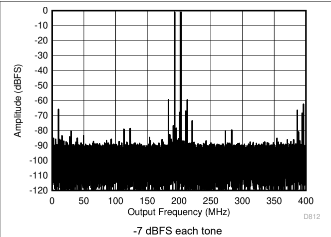
5-70. Two Tone FFT at 1798 MHz in Low Power Mode
