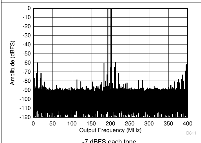
Figure 5-67. Two Tone FFT at 1798 MHz
