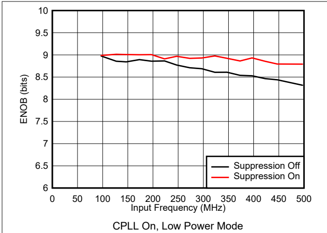
Figure 5-63. ENOB vs Input Frequency
