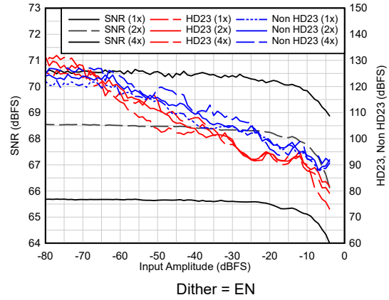
6-34. AC Performance vs A_{IN}
