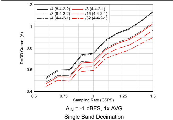
6-51. Current vs Sampling Rate vs Complex Decimation
