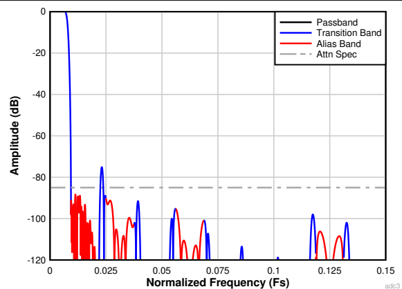
7-30. Complex Decimation by 64 Filter Response
