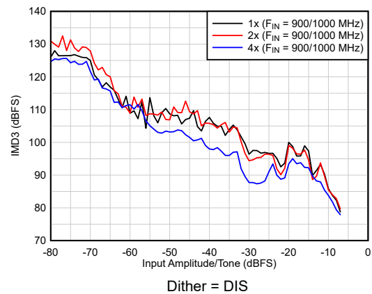
6-36. IMD3 Performance vs A_{IN}
