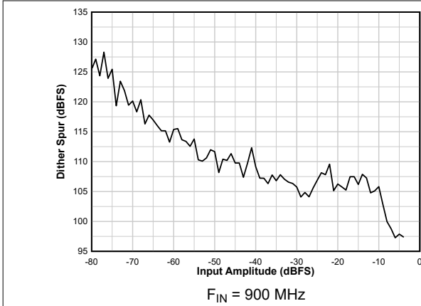
6-31. Dither Spur vs A_{IN}
