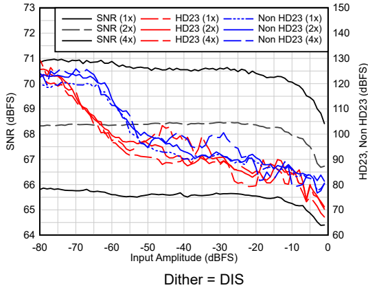
6-33. AC Performance vs A_{IN}
