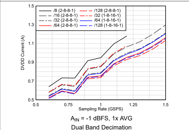
6-54. Current vs Sampling Rate vs Complex Decimation
