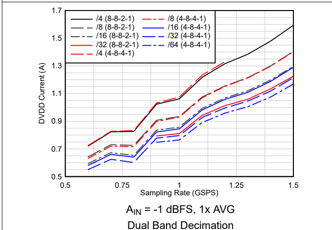
6-53. Current vs Sampling Rate vs Complex Decimation
