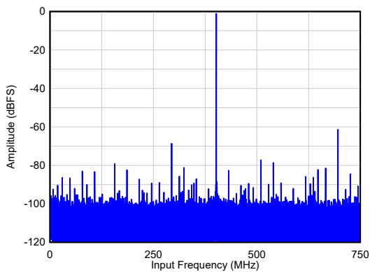
6-7. Single Tone FFT at F_{IN} = 1400\text{ MHz}
