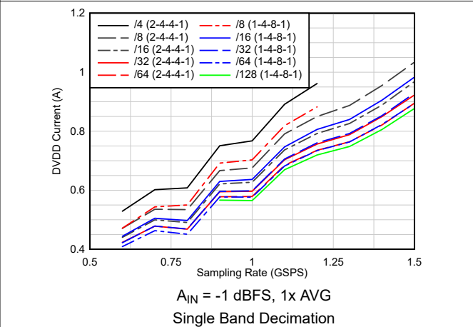
6-52. Current vs Sampling Rate vs Complex Decimation
