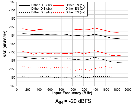
6-32. NSD Performance vs F_{IN}
