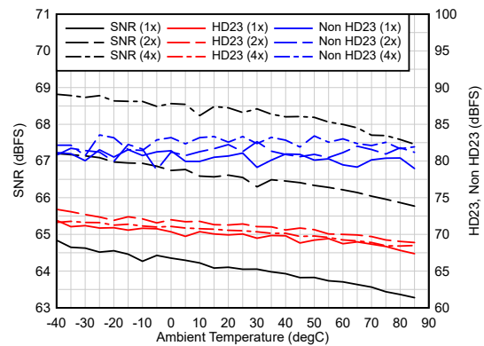
Figure 6-42. AC Performance vs Temperature F_{IN} = 900\text{ MHz} , A_{IN} = -1\text{ dBFS} , Dither = DIS
