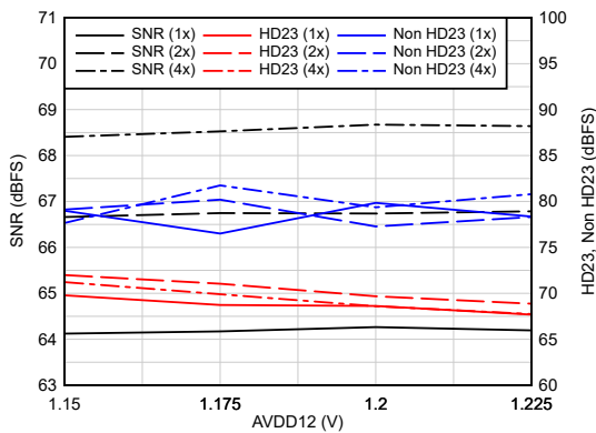
Figure 6-41. AC Performance vs AVDD12 F_{IN} = 900\text{ MHz} , A_{IN} = -1\text{ dBFS} , Dither = DIS
