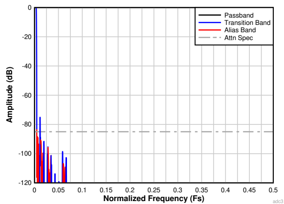
7-32. Complex Decimation by 128 Filter Response
