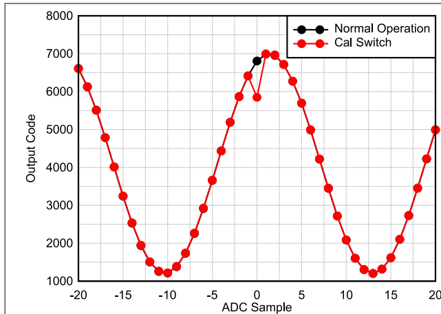
図 7-18. Output Code vs ADC Sample
