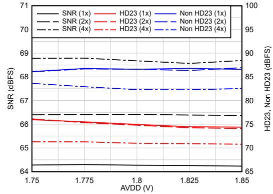
Figure 6-40. AC Performance vs AVDD18 F_{IN} = 900\text{ MHz} , A_{IN} = -1\text{ dBFS} , Dither = DIS
