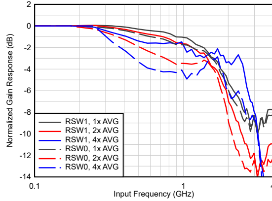
図 7-2. Full power input bandwidth
