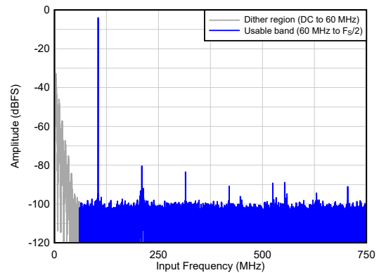
6-2. Single Tone FFT at F_{IN} = 100\text{ MHz}
