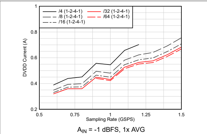
6-50. Current vs Sampling Rate vs Real Decimation
