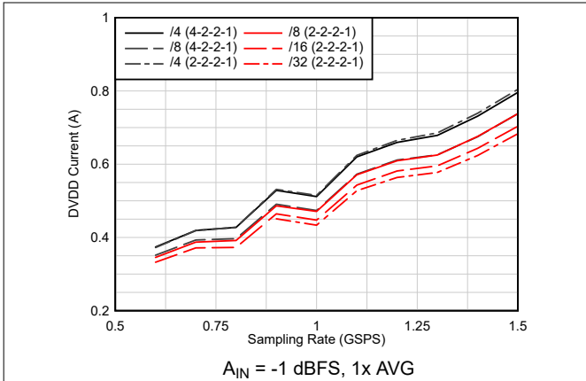
6-49. Current vs Sampling Rate vs Real Decimation
