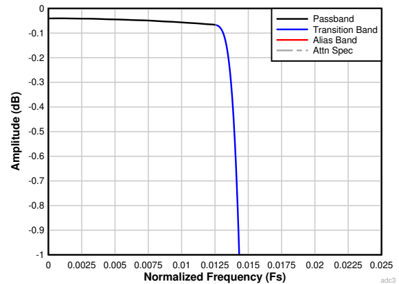
7-28. Decimation by 32 Passband Ripple Response
