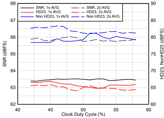
Figure 6-39. AC Performance vs Clock Duty Cycle F_{IN} = 900\text{ MHz} , A_{IN} = -1\text{ dBFS} , Dither = DIS
