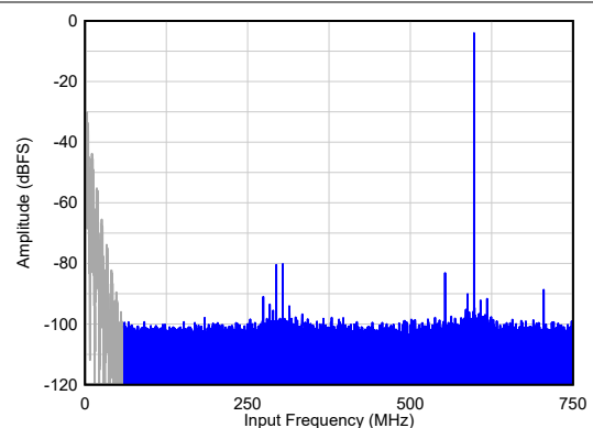
6-4. Single Tone FFT at F_{IN} = 600\text{ MHz}
