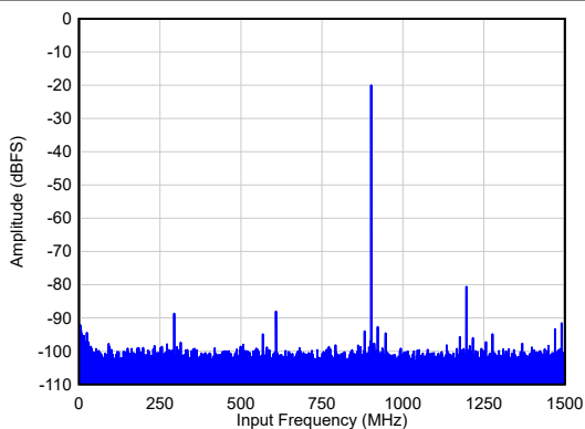
5-13. Single Tone FFT at F_{IN} = 900\text{ MHz}
