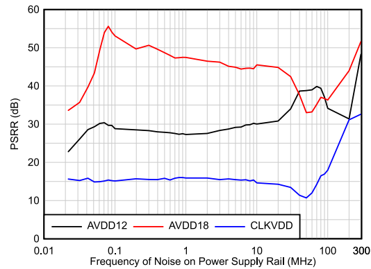
図 7-5. Power supply rejection ratio (PSRR) vs frequency
