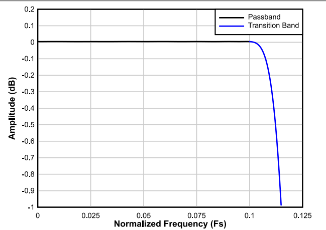
6-25. Decimation by 4 Passband Ripple Response
