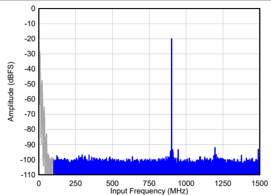
5-14. Single Tone FFT at F_{IN} = 900\text{ MHz}
