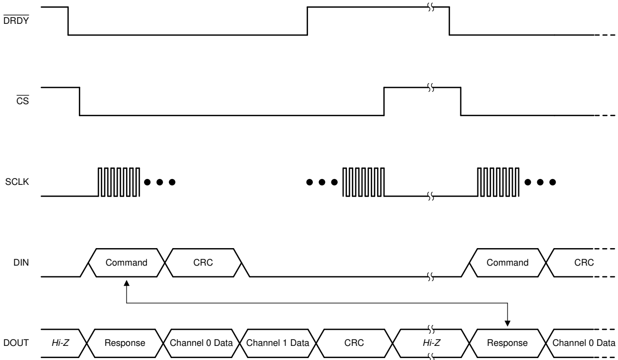
图 8-14. Typical Communication Frame
