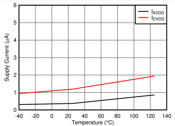
6-13. Analog Supply Current vs Temperature
