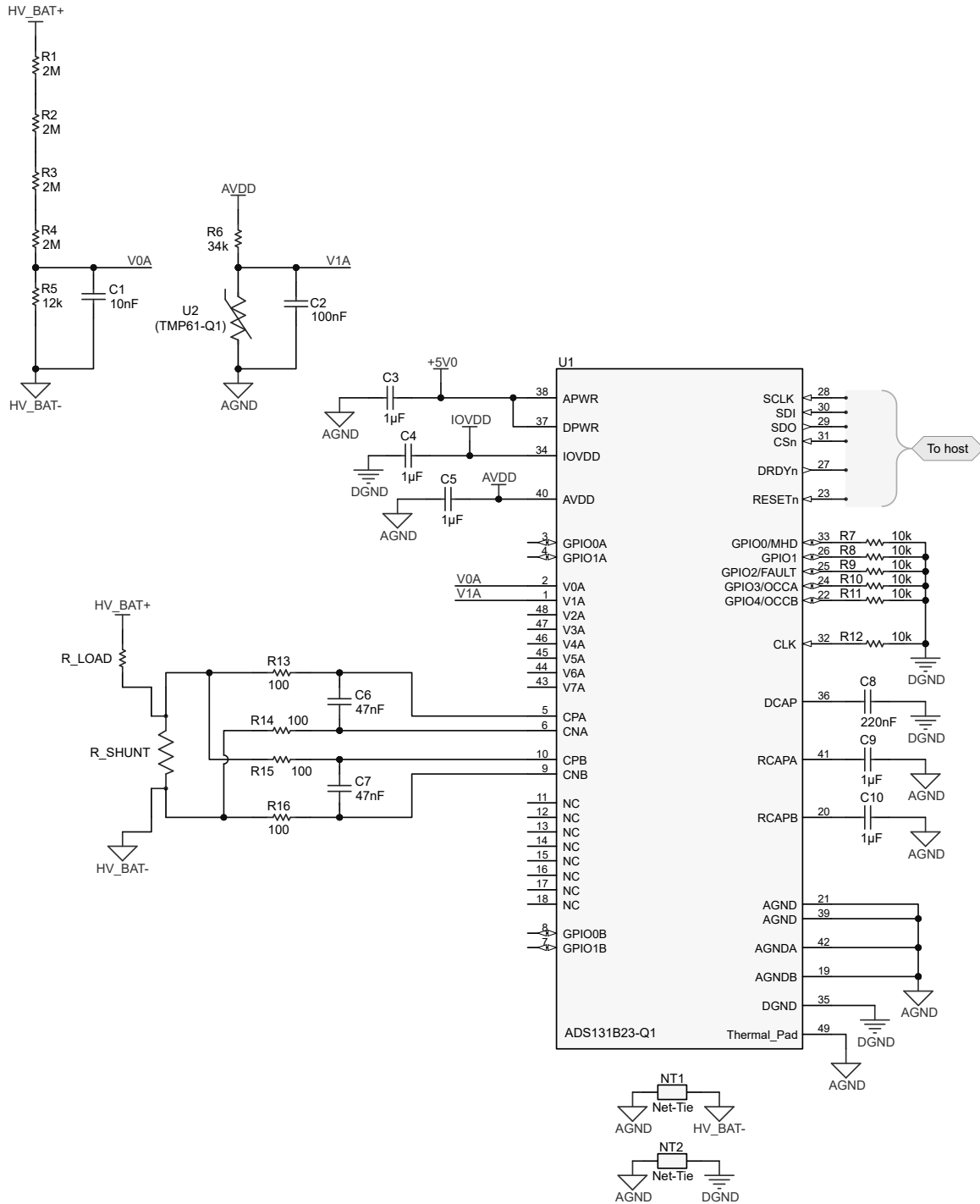
10-1. The ADS131B23-Q1 in a Typical Battery Management System Application
