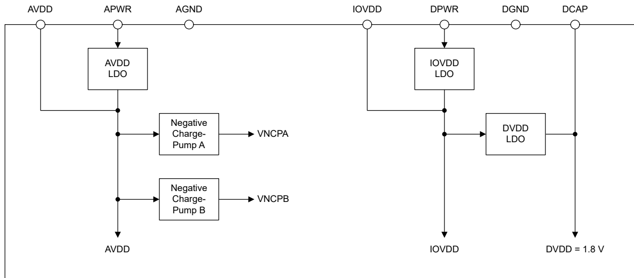
10-4. Power-Supply Architecture
