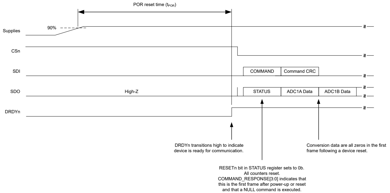
9-26. DRDYn Pin Behavior After POR
