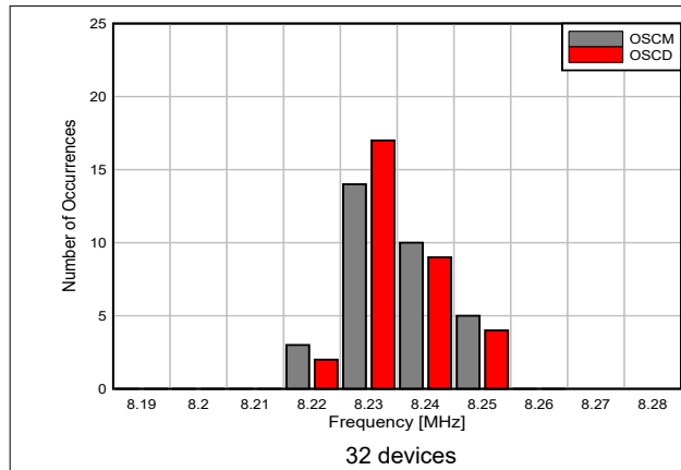
7-14. OSCM and OSCD Frequency Histogram
