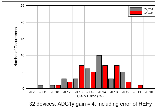
7-18. OCCy Gain Error Histogram
