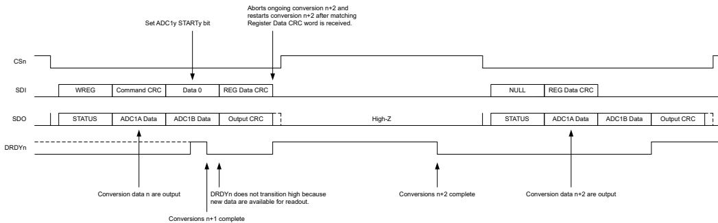
9-45. DRDYn Pin Behavior: Setting the STARTy Bit and Reading Conversion Data While New Conversions Complete
