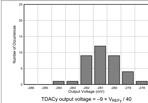
7-24. Test DACy Output Voltage Histogram
