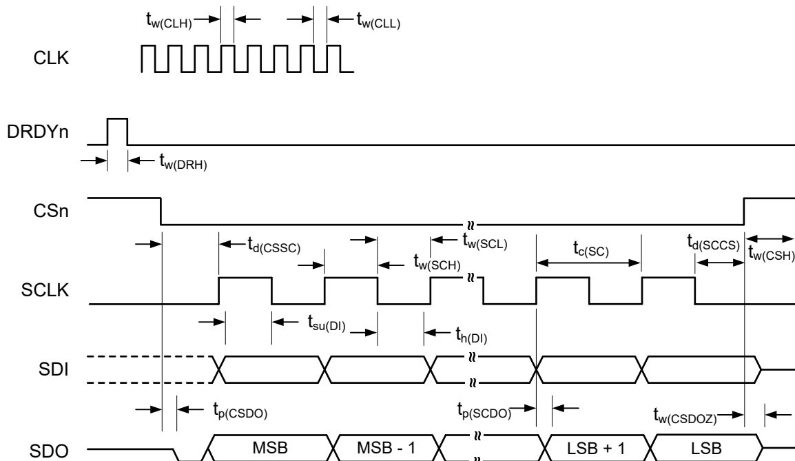
FIG 7-1. SPI Timing Requirements and Switching Characteristics
