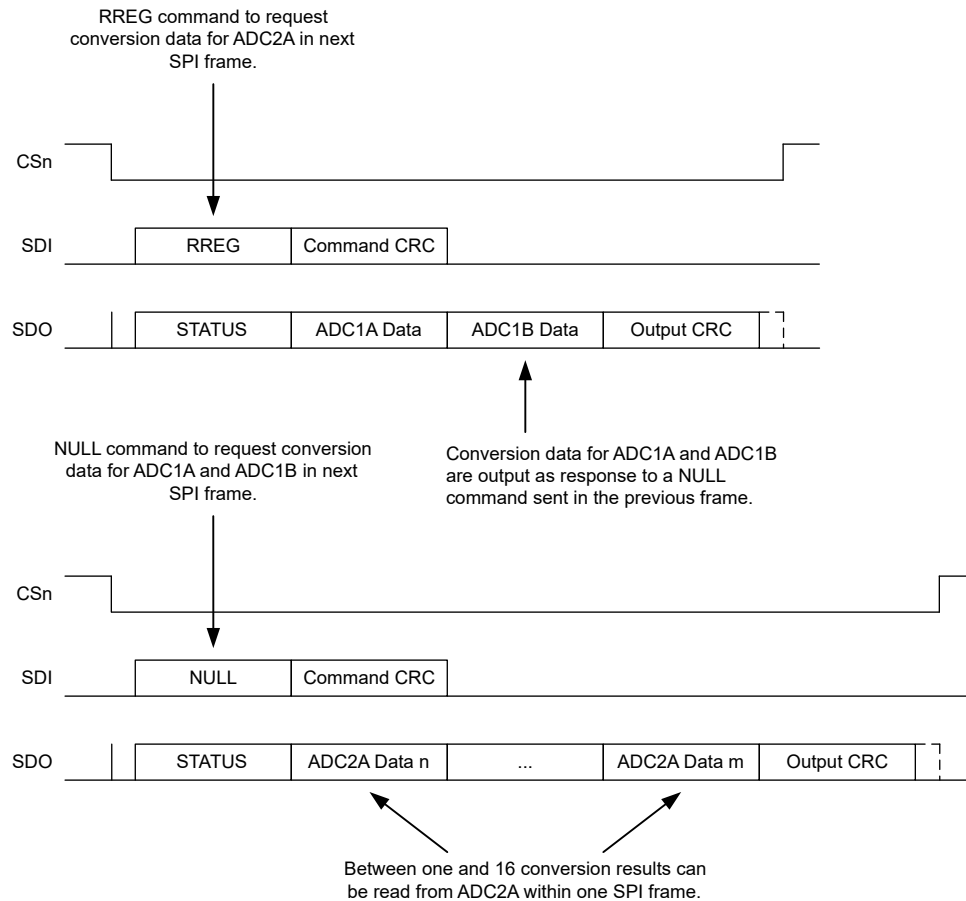
Figure 9-38. Reading Conversion Data From ADC1A, ADC1B, and ADC2A Within Two SPI Frames
