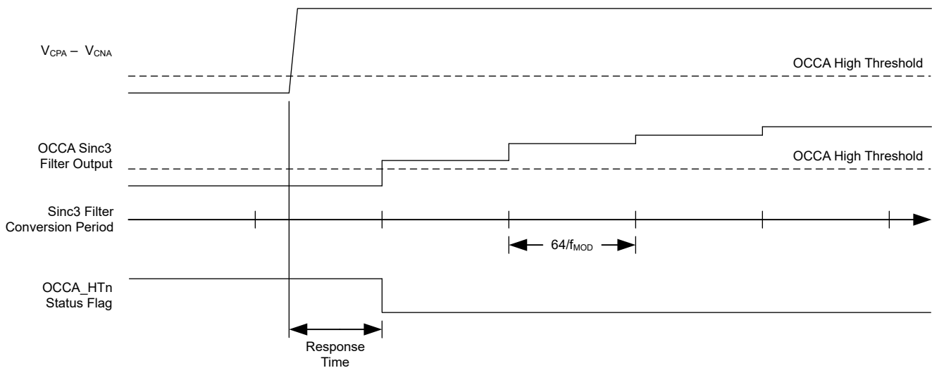
☒ 9-14. OCCA Behavior With Large Input Overshoot
