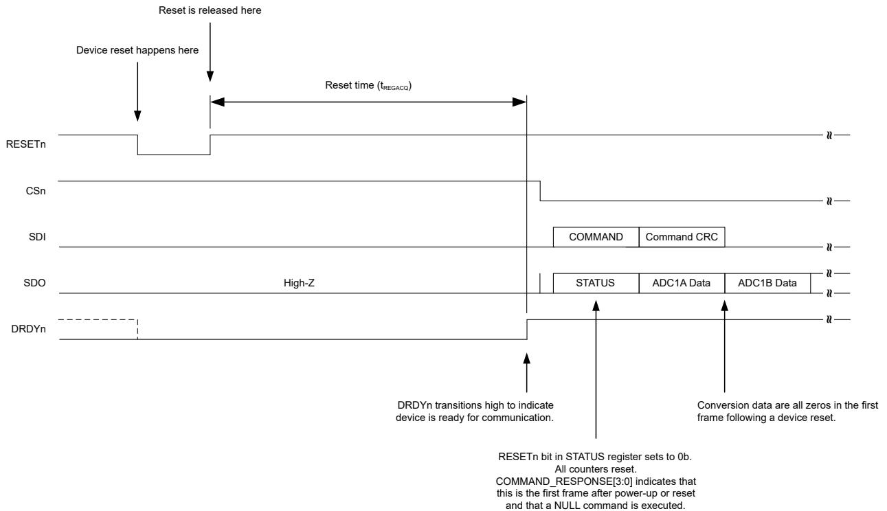
9-27. DRDYn Pin Behavior After Device Reset
