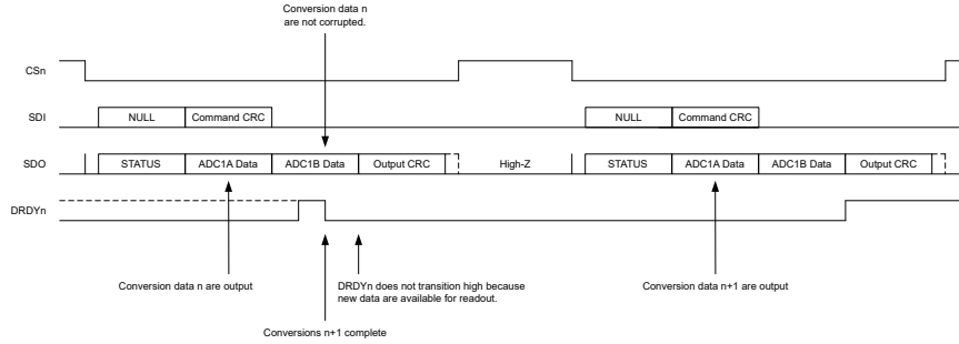
9-42. DRDYn Pin Behavior: Reading Conversion Data While New Conversions Complete
