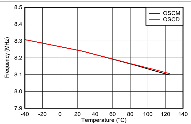
7-15. OSCM and OSCD Frequency vs Temperature
