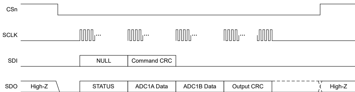
Figure 9-28. Typical Communication Frame
