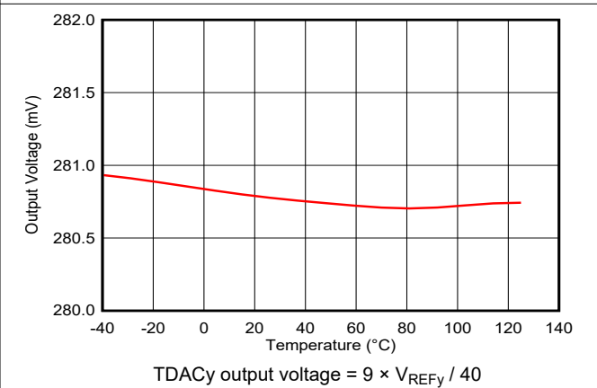
7-23. Test DACy Output Voltage vs Temperature
