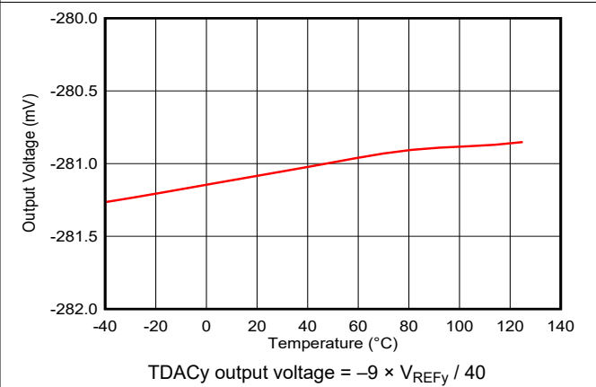
7-25. Test DACy Output Voltage vs Temperature
