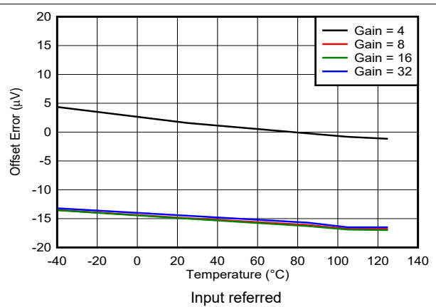
7-17. OCCy Offset Error vs Temperature
