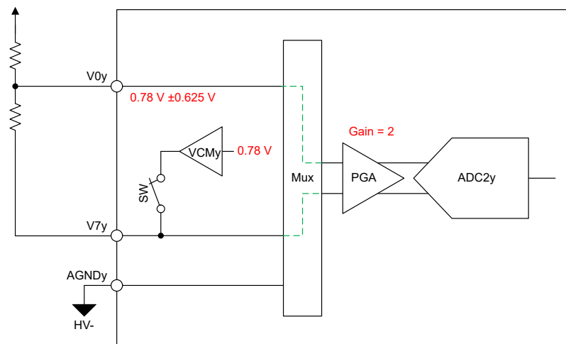
☒ 9-11. Pseudo-Differential Input, Bipolar Voltage Measurement (Gain = 2, Using Internal Bias Voltage)
