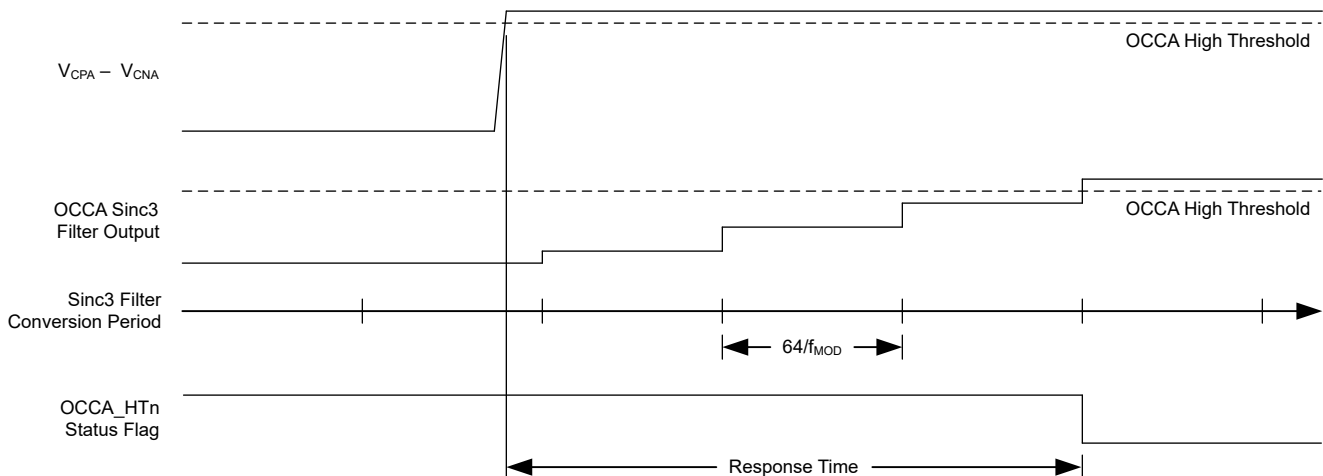
☒ 9-15. OCCA Behavior With Small Input Overshoot
