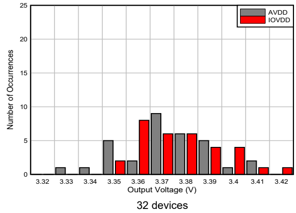
7-33. AVDD and IOVDD LDO Output Voltage Histogram
