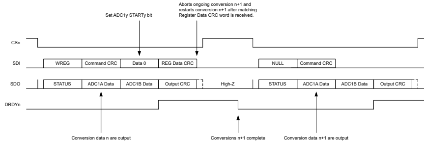
9-44. DRDYn Pin Behavior: Setting the STARTy Bit While Reading Conversion Data
