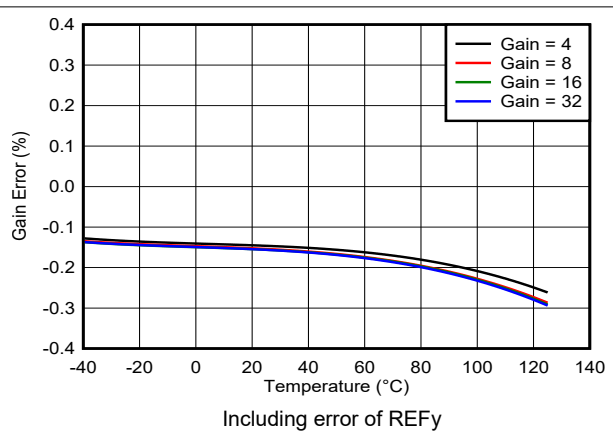
7-19. OCCy Gain Error vs Temperature
