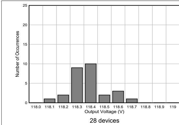
7-20. Temperature Sensor Output Voltage Histogram
