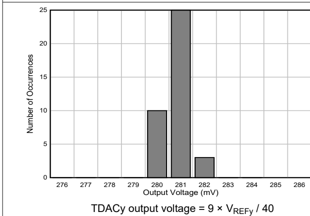
7-22. Test DACy Output Voltage Histogram
