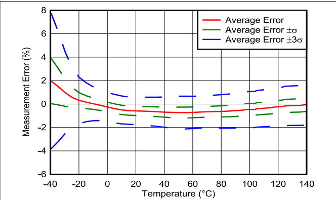
7-21. Temperature Sensor Measurement Error vs Ambient Temperature
