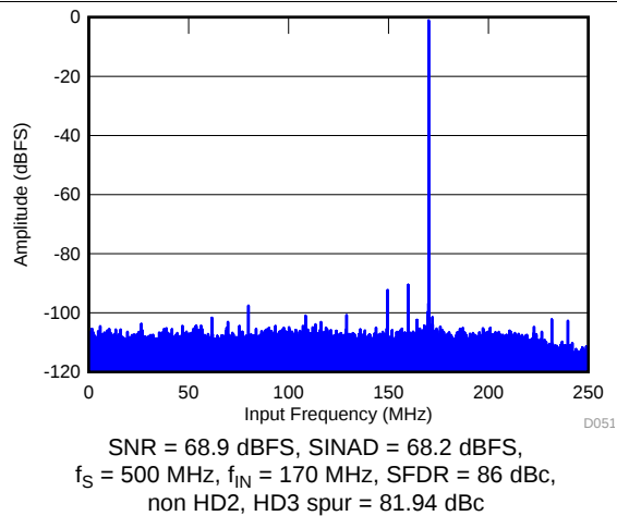
Figure 53. FFT for 170-MHz Input Signal in Decimate-by-2 Mode
