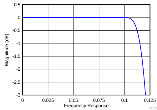
Figure 65. Decimate-by-4 IQ Output Filter Response (Zoomed)
