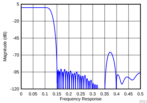
Figure 64. Decimate-by-4 IQ Output Filter Response
