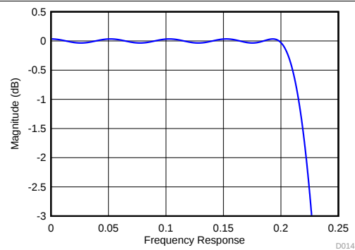
Figure 61. Decimate-by-2 Filter Response (Zoomed)
